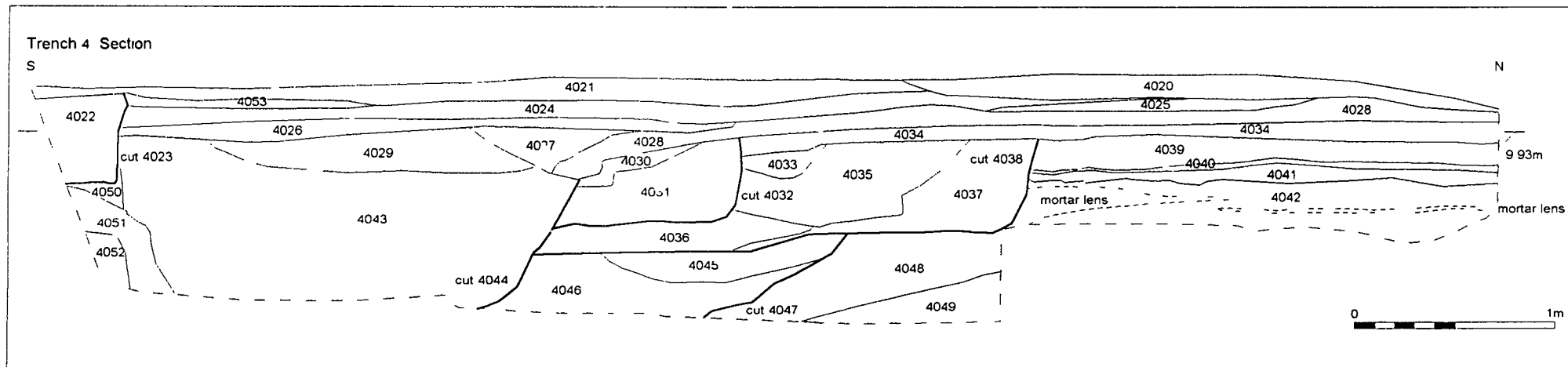
Figure 8 Trench 4 East Facing Section
