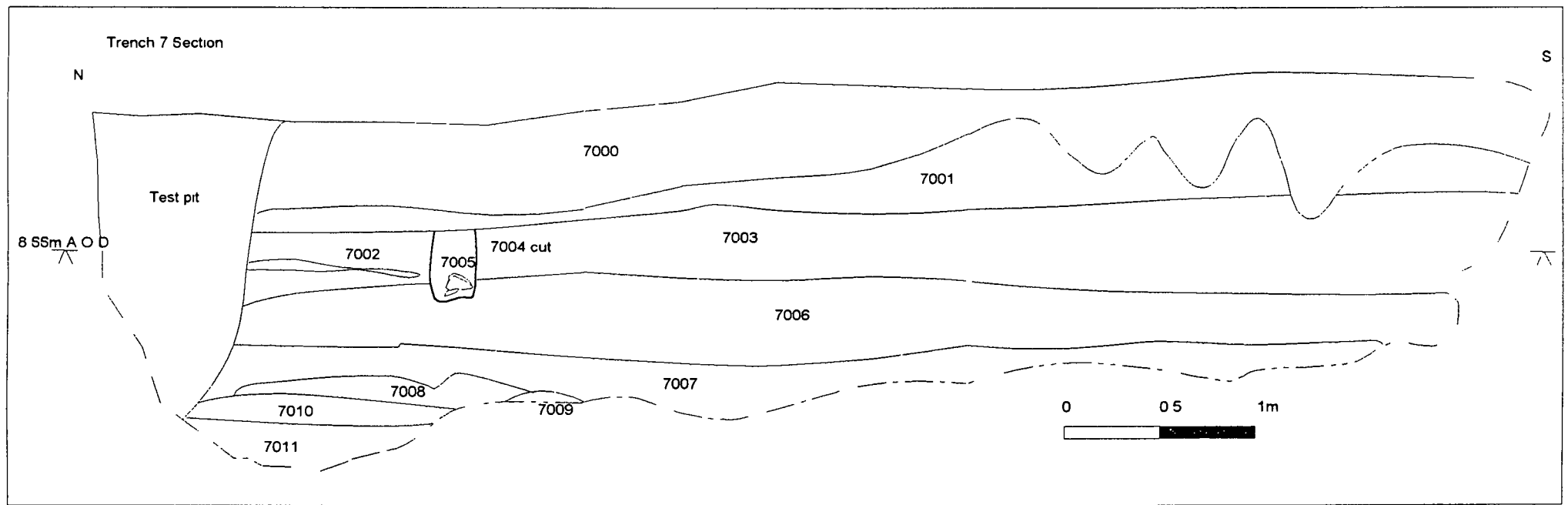
Figure 15 Plan of Trench 7
