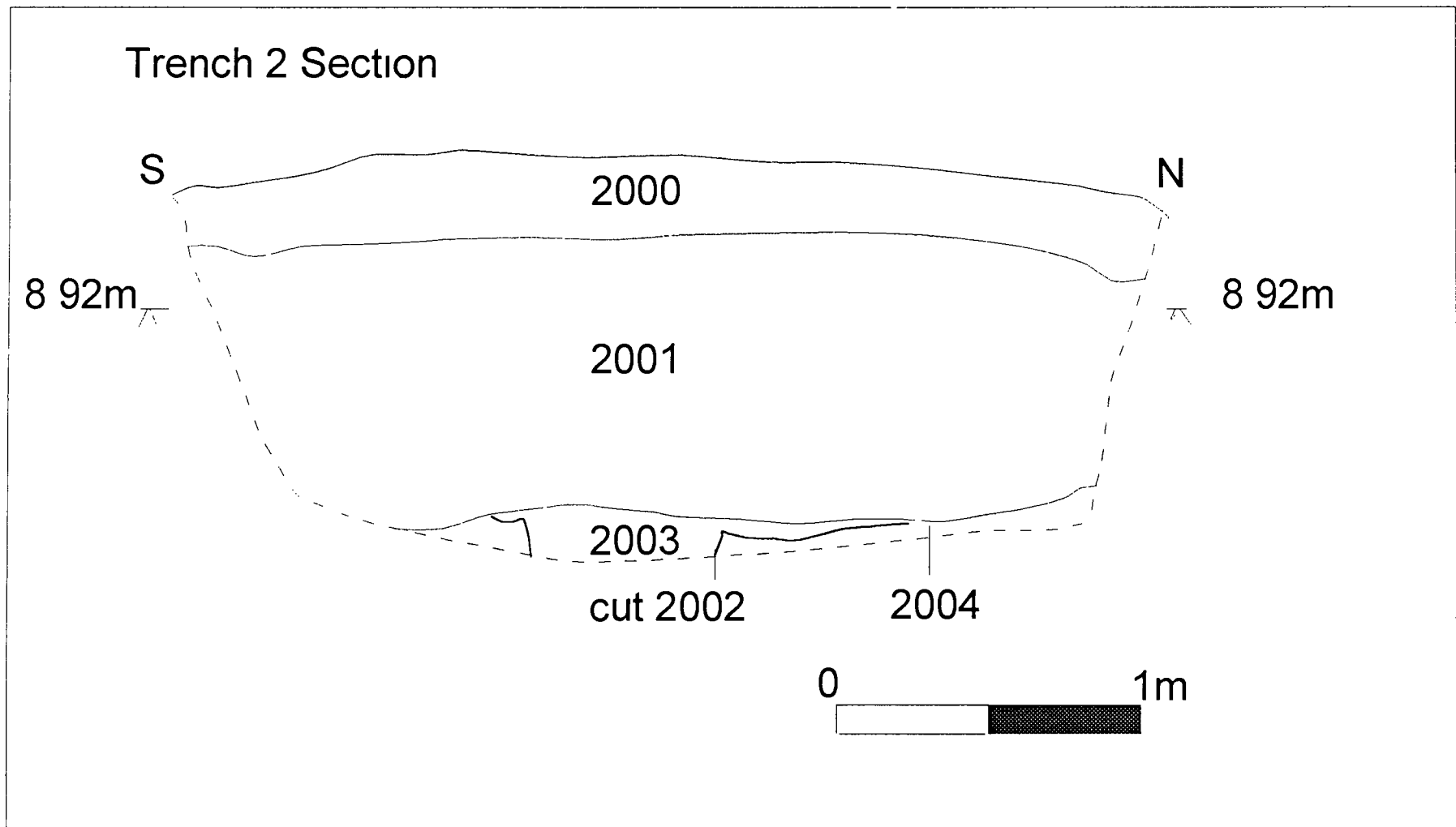
Figure 12 Trench 2 East Facing Section
