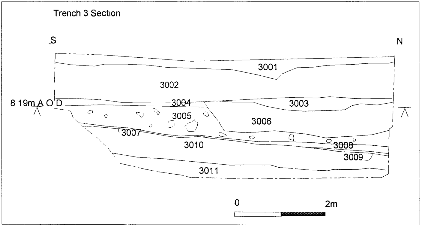
Figure 14 Trench 3 East Facing Section
