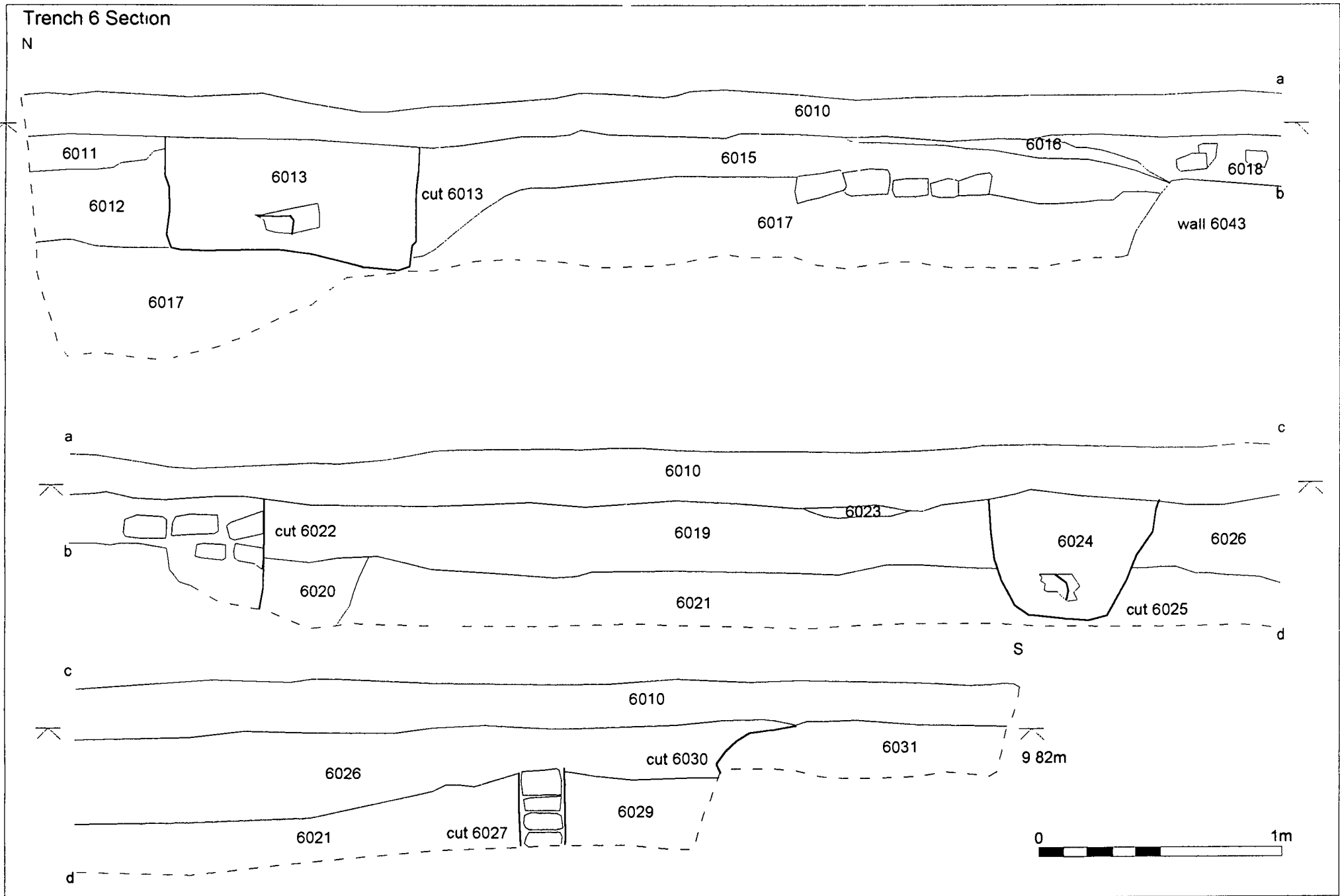
Figure 10 Trench 6 East Facing Section
