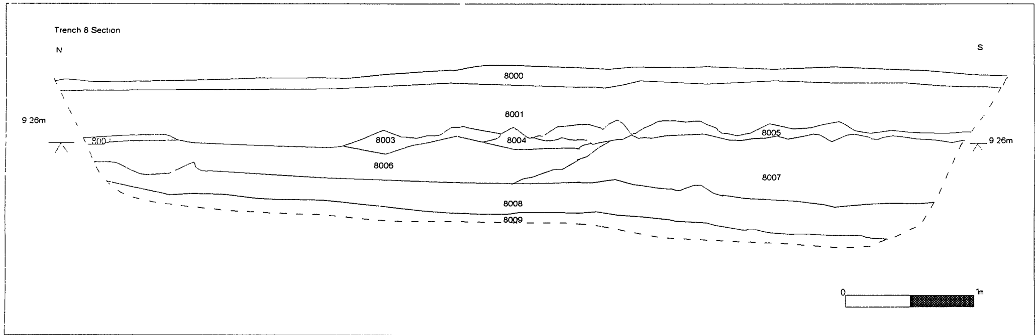
Figure 17 Trench 8 West Facing Section
