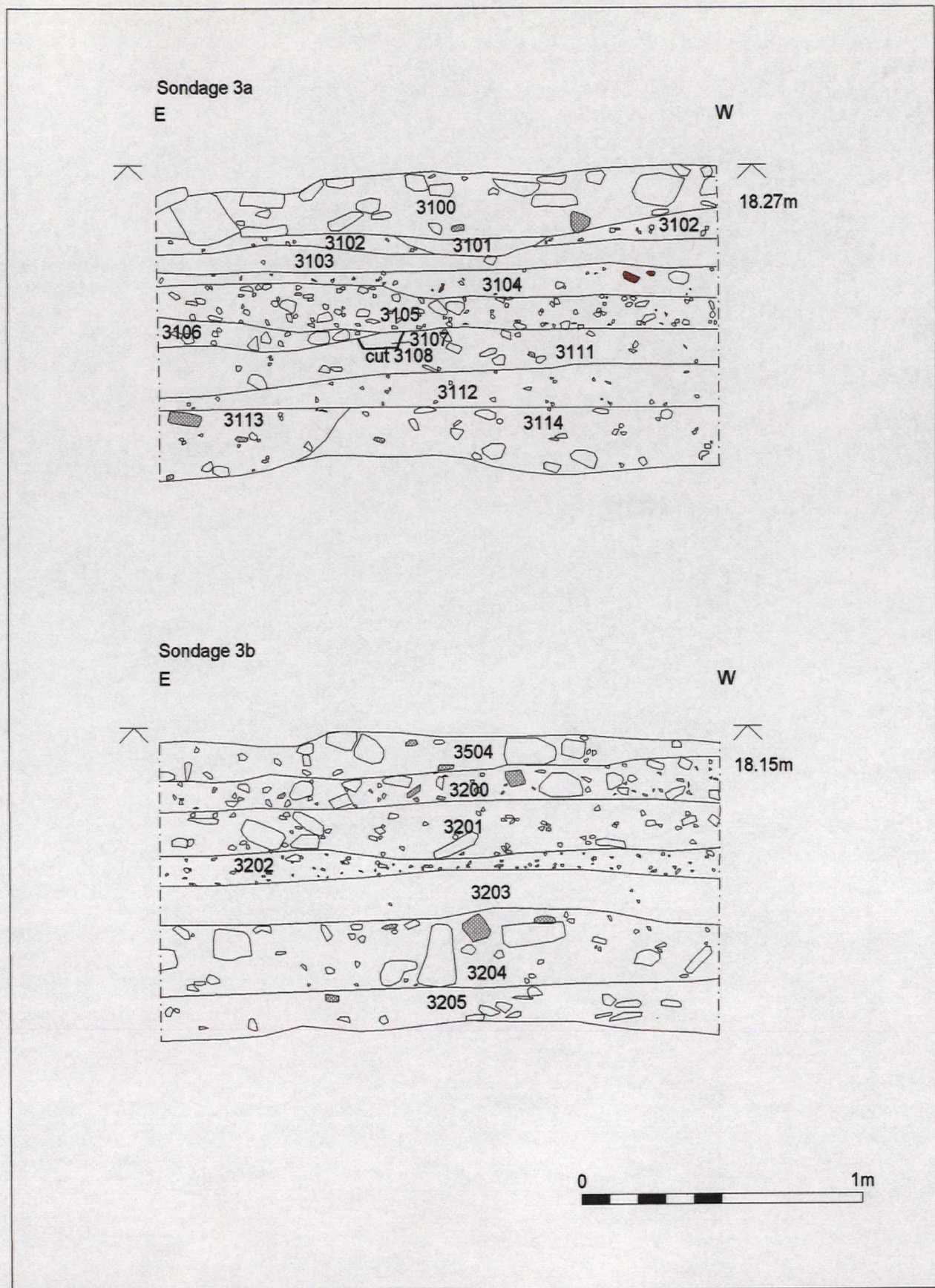
Figure 13. Trench 3 Sections.
