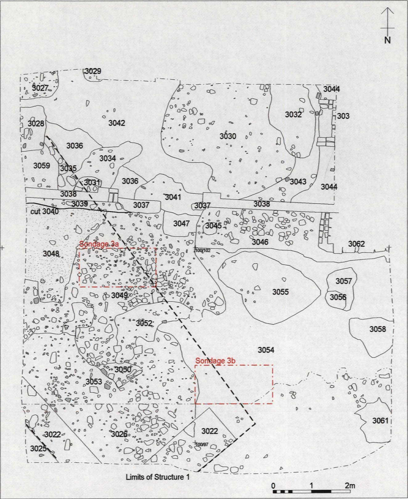
Figure 12. Trench 3 Plan.
