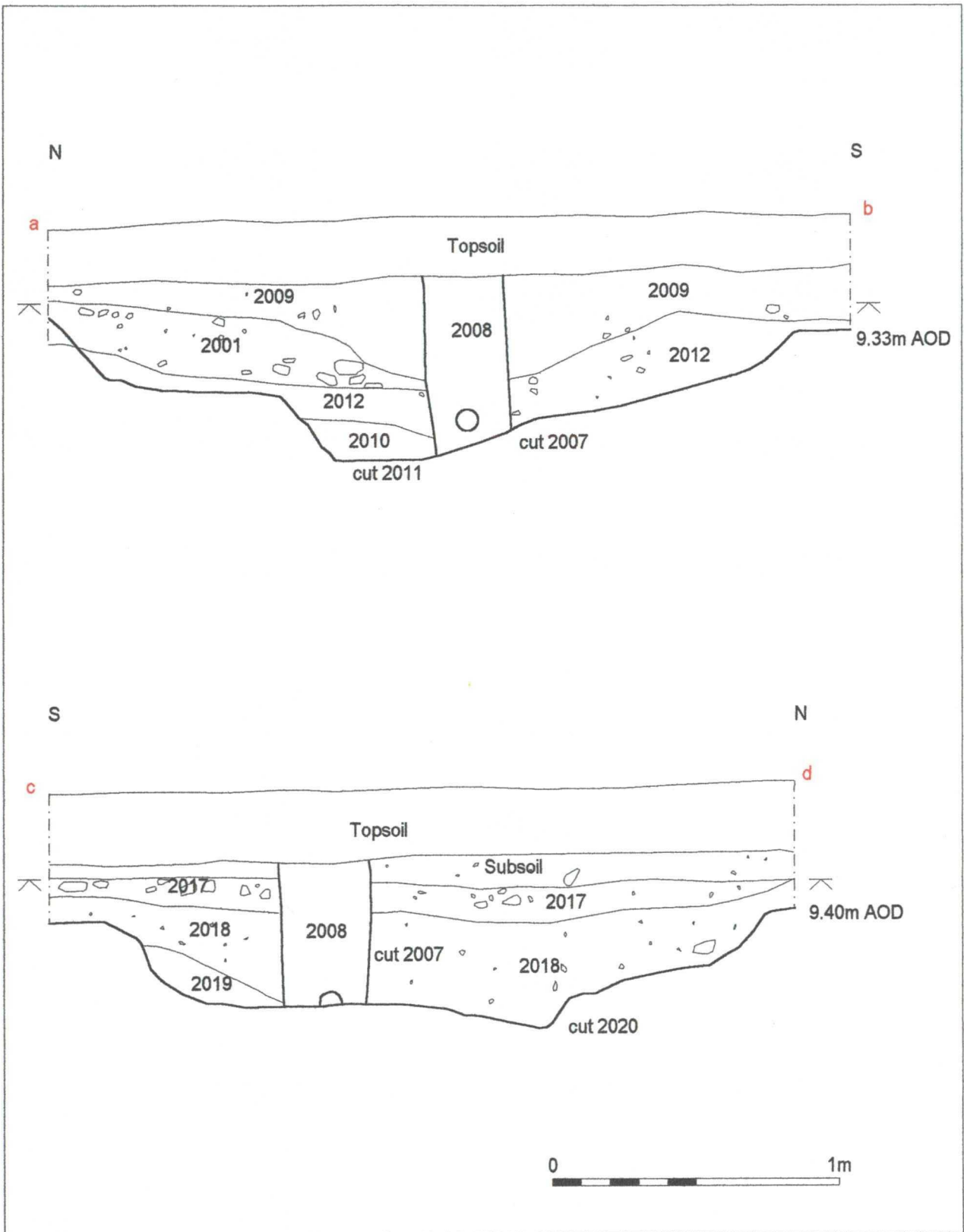
Figure 13. Trench 2 Sections.
