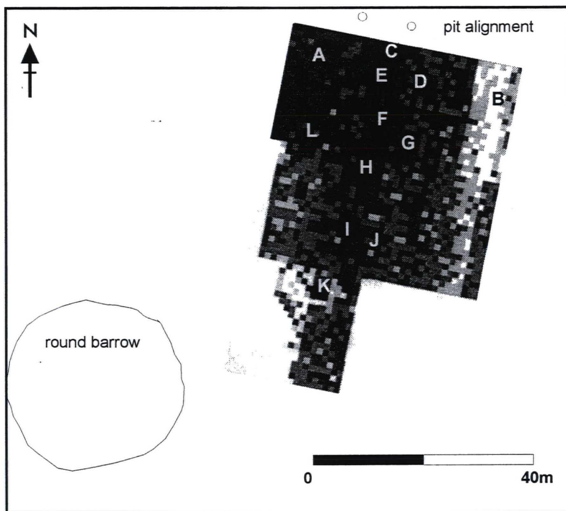
Fig.7 Labelled greyscale image of the magnetometer survey at Grid 1
