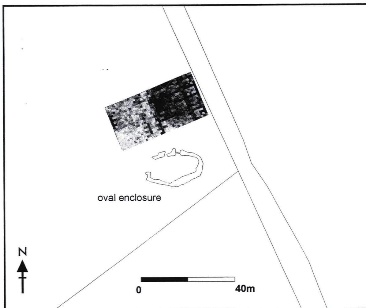
Fig.11 Greyscale image of the magnetometer survey at Grid 3
