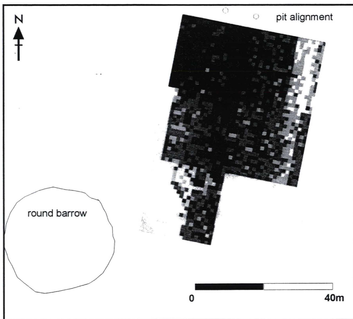
Fig.6 Greyscale image of the magnetometer survey at Grid 1
