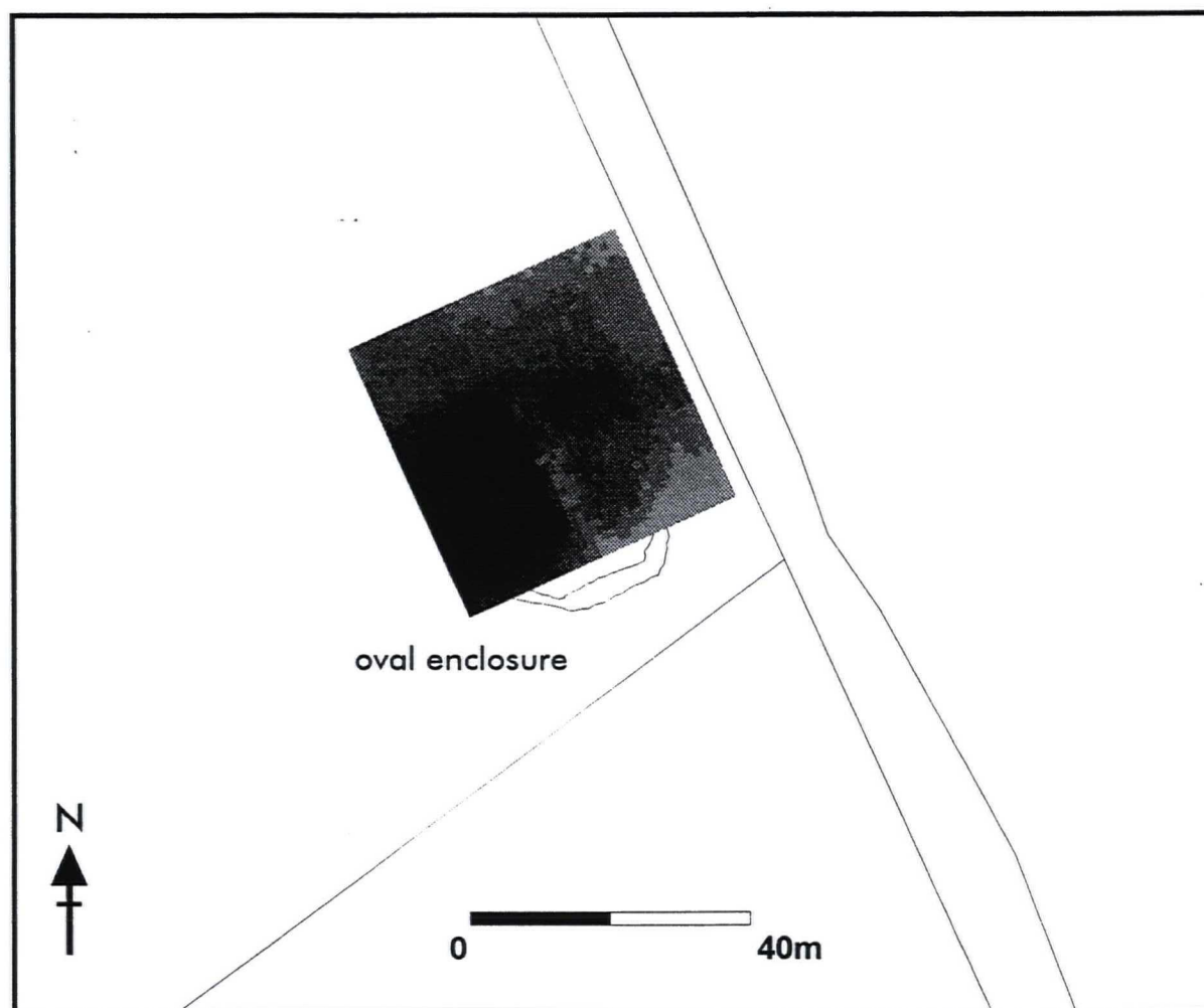
Fig.10 Greyscale image of the resistivity survey at Grid 3
