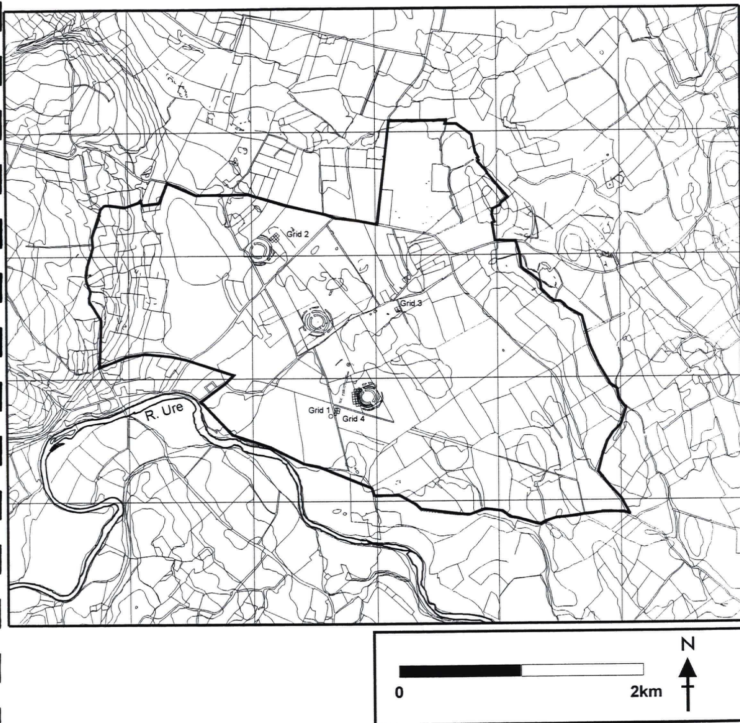
Fig.2 The Thornborough study area, showing the location of geophysical survey grids
