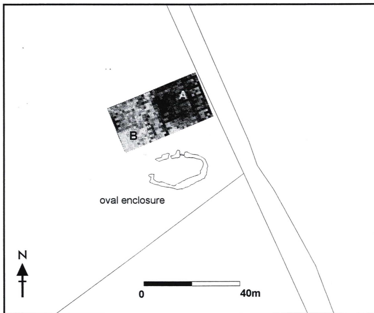
Fig.13 Labelled greyscale image of the magnetometer survey at Grid 3
