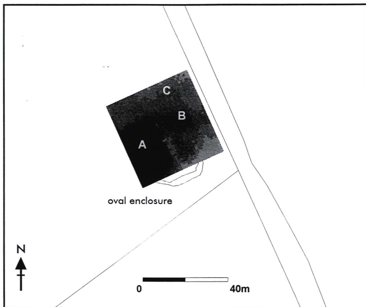
Fig.12 Labelled greyscale image of the resistivity survey at Grid 3
