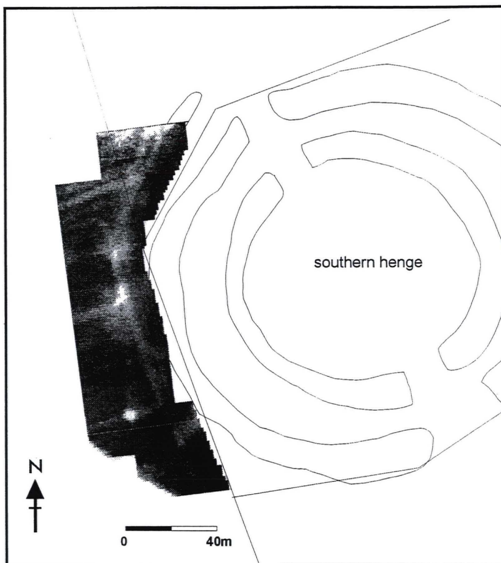
Fig.14 Greyscale image of resistivity survey at Grid 4
