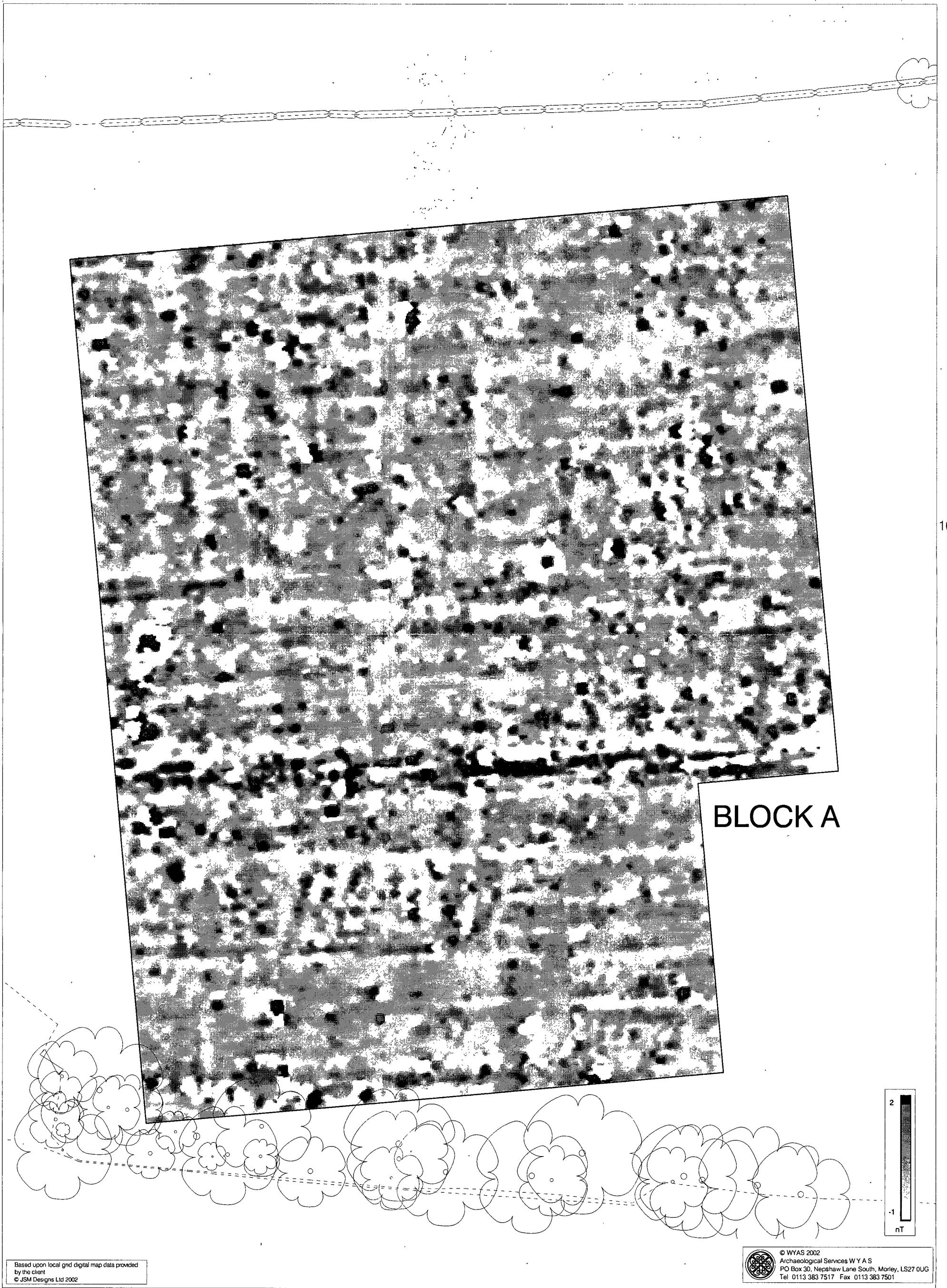
Land off Gatherley Road, Brompton on Swale Greyscale gradiometer data; Block A
