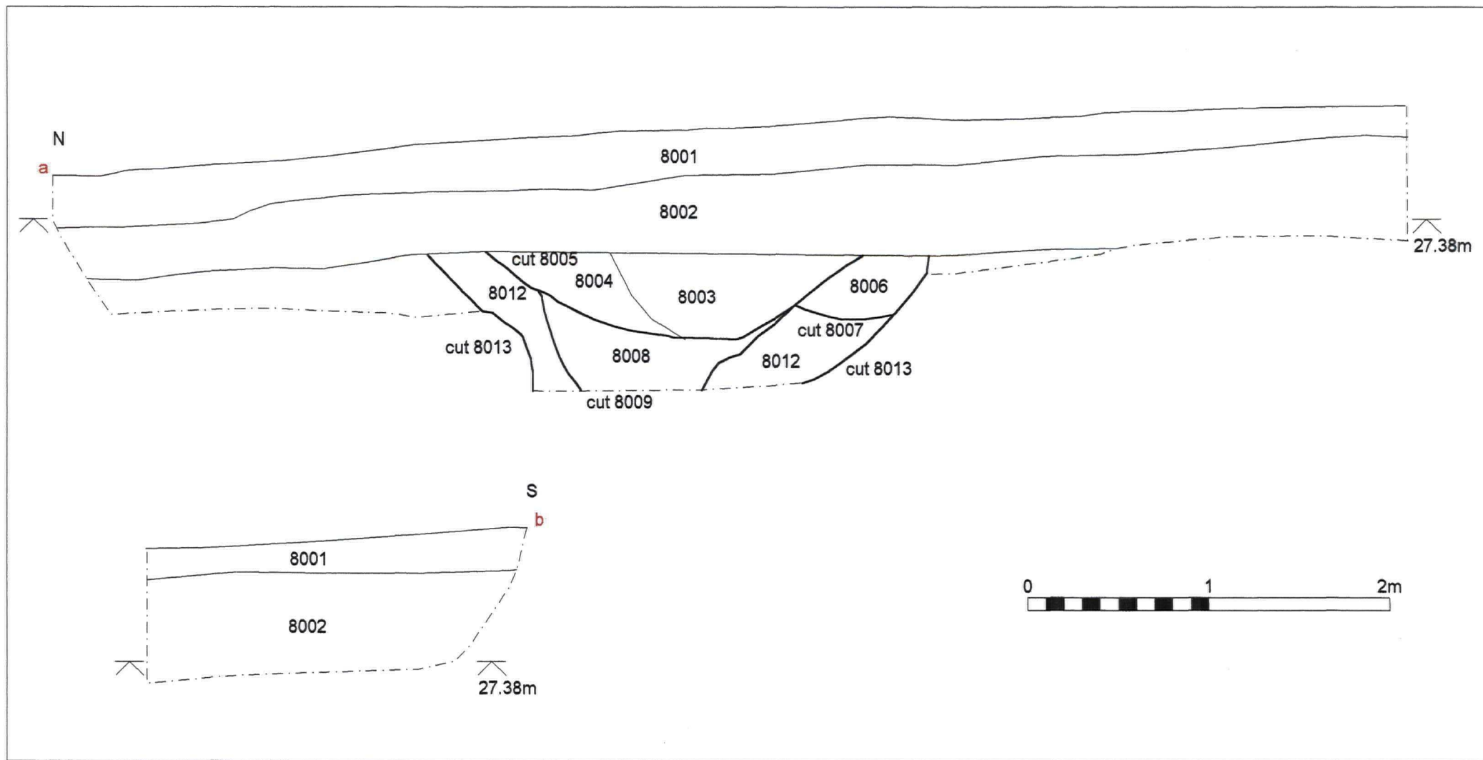
Figure 11. Trench 8 Section.
