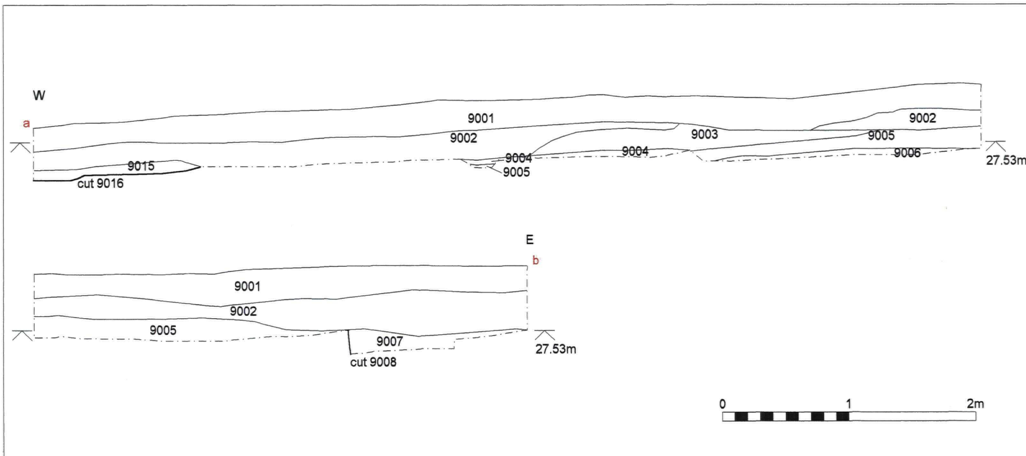
Figure 13. Trench 9 Section.
