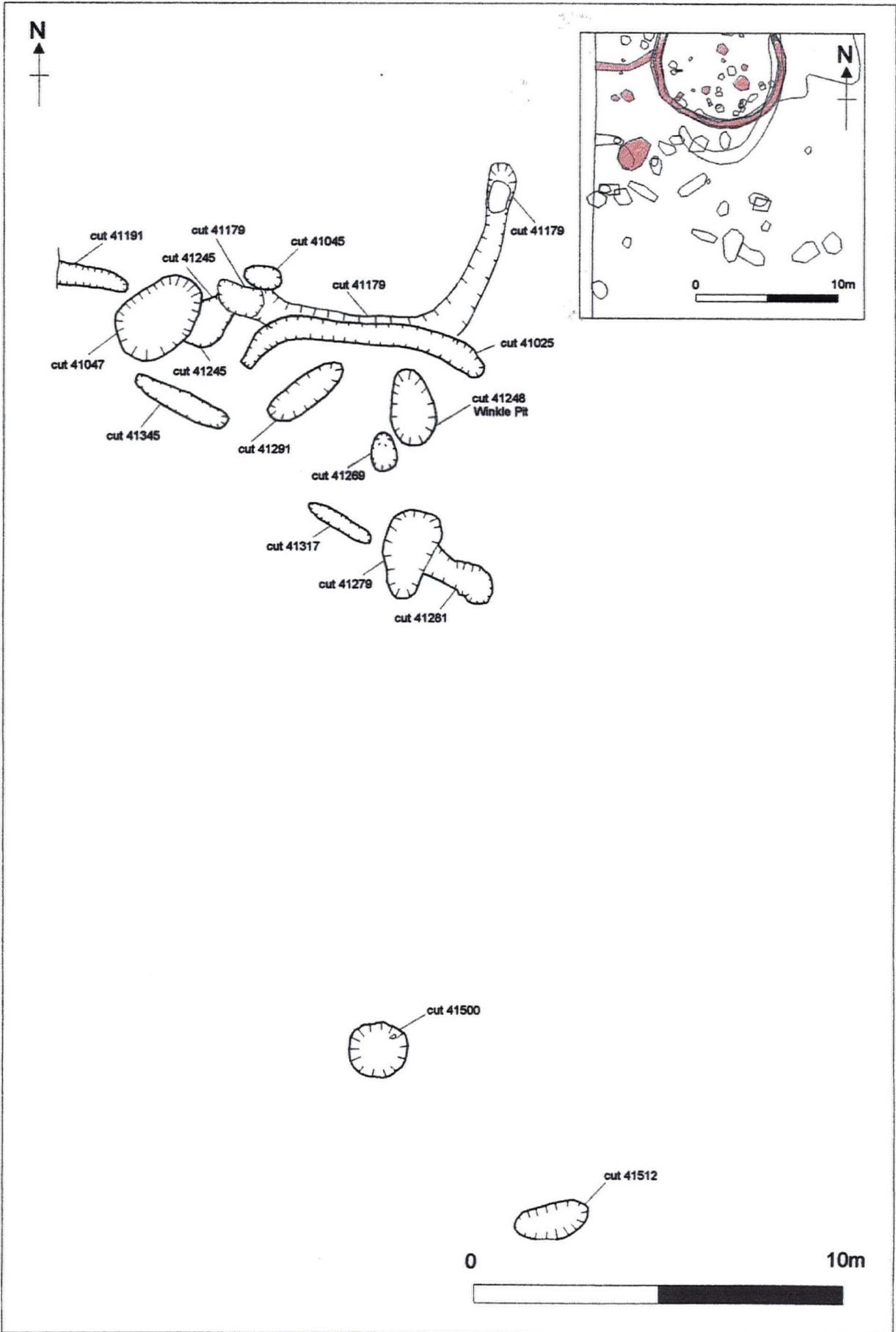
Figure 12. Gullies 41179 & 41025
