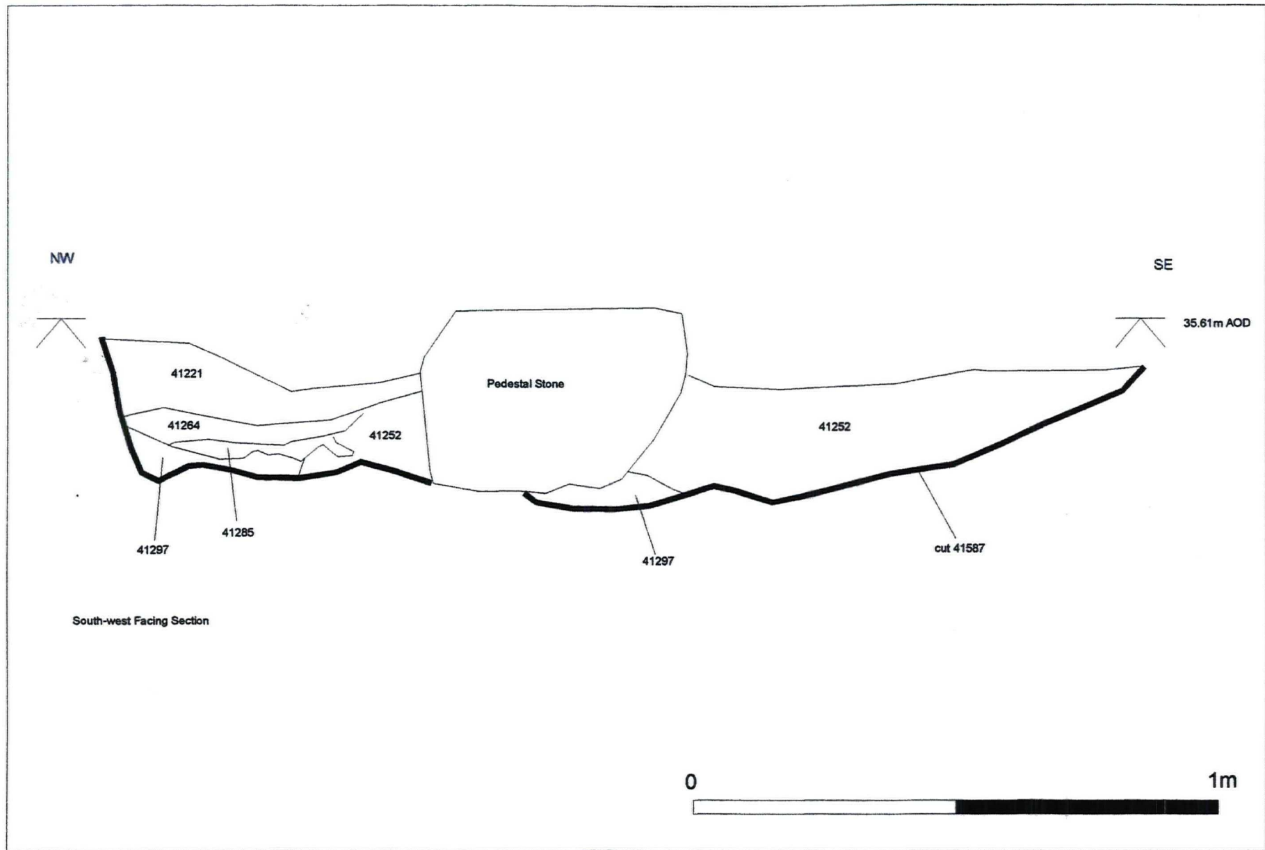
Figure 16. Kiln Section
