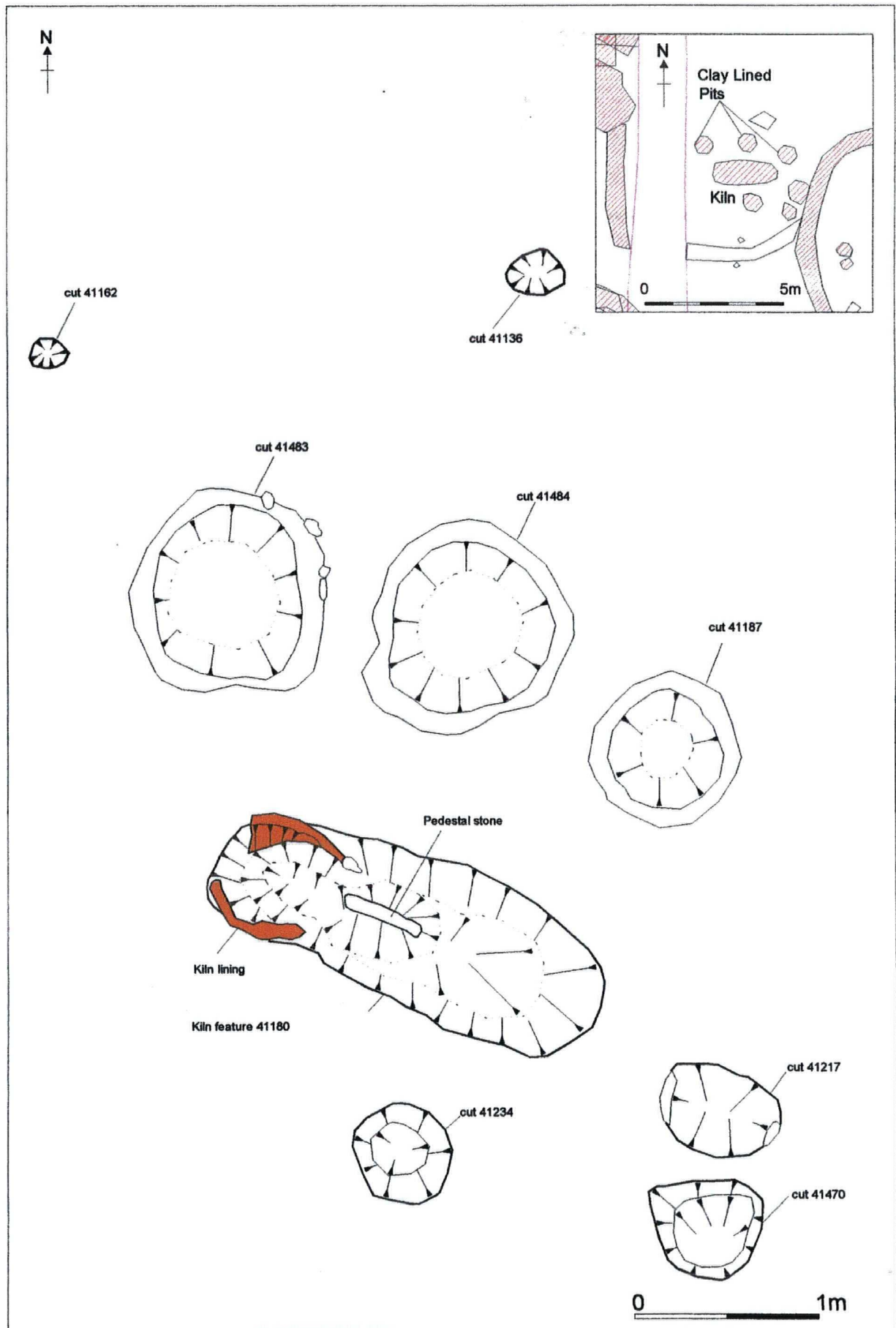
Figure 15. Kiln plan & clay pits
