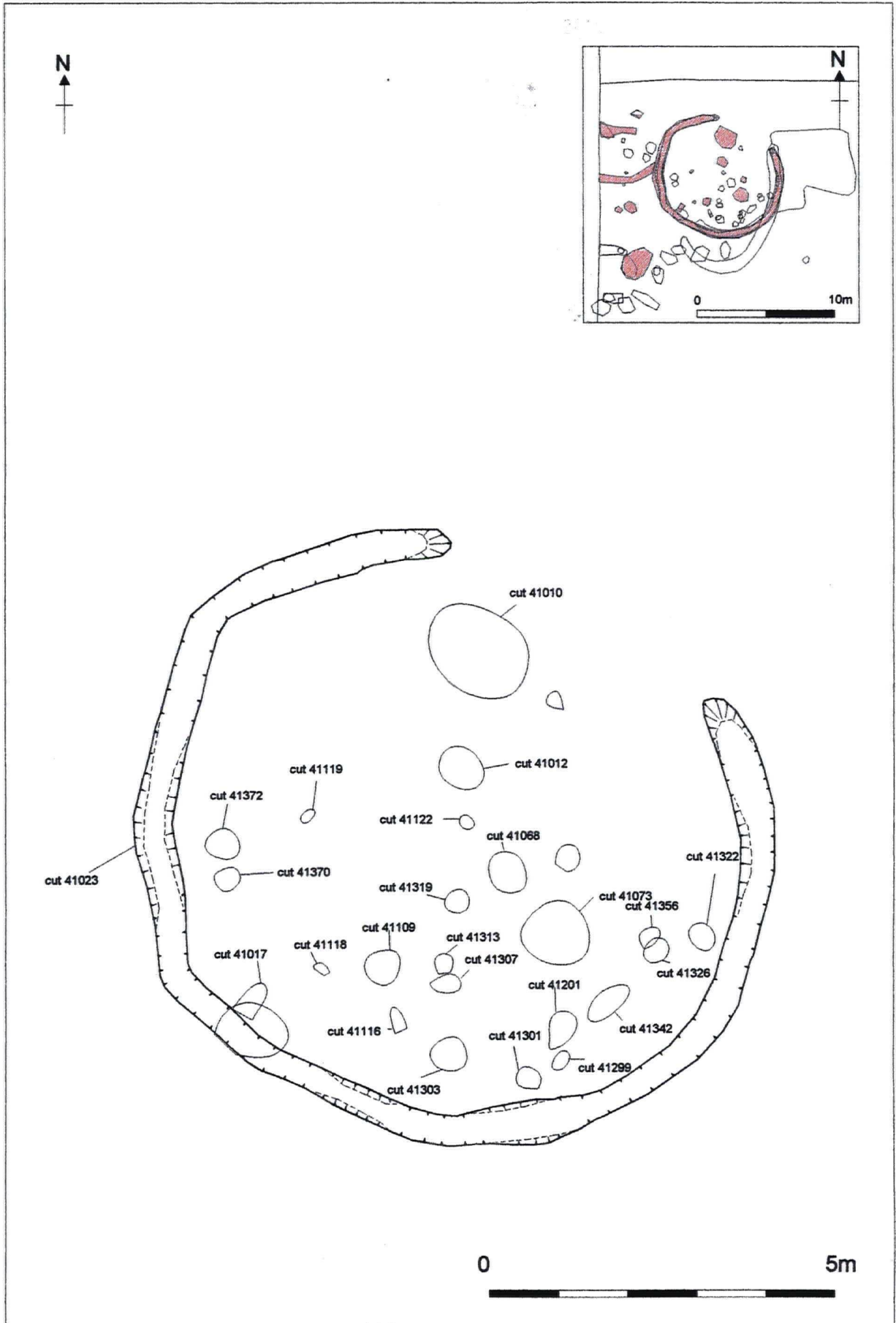
Figure 11. Structure 2
