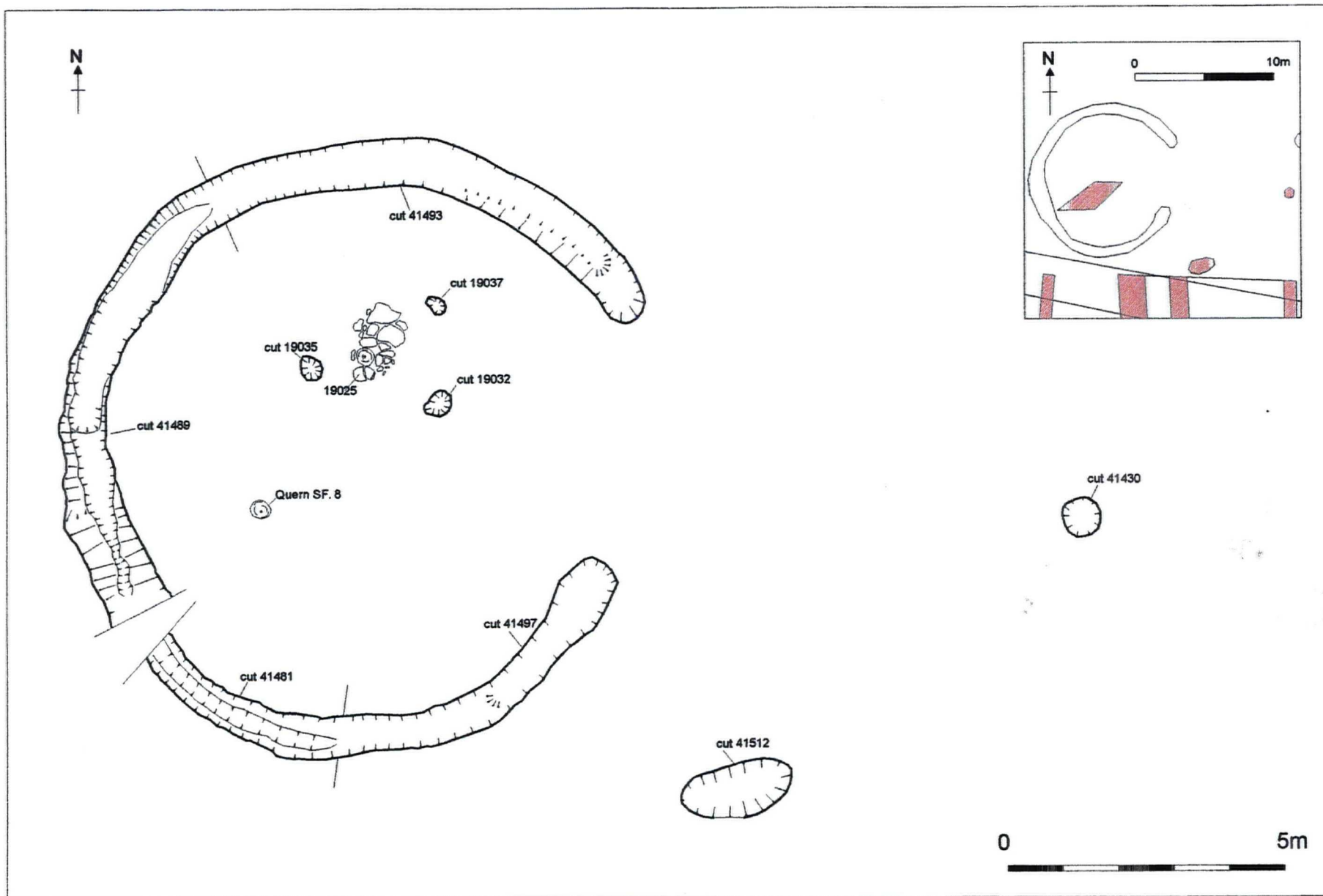
Figure 14. Structure 4 & pits 411430 & 41512
