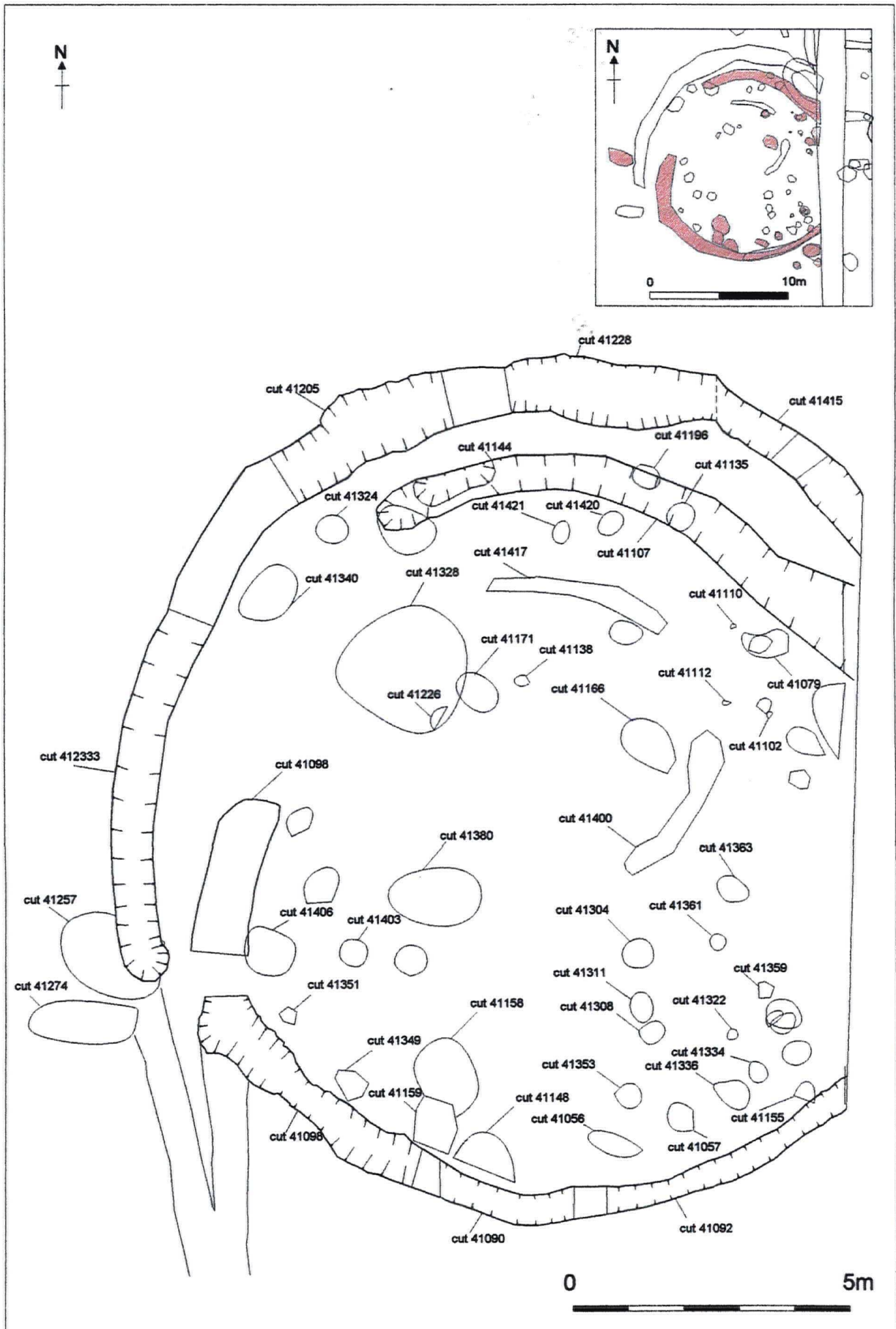
Figure 13. Structure 3
