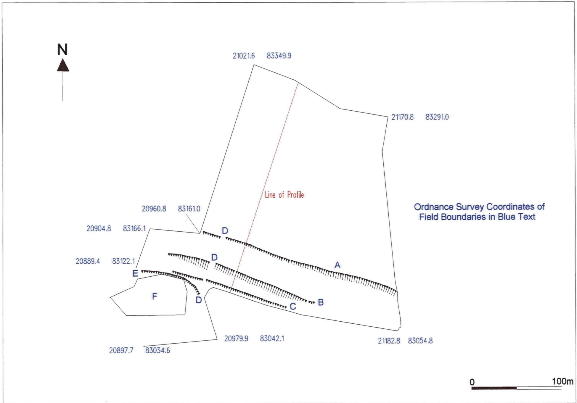
Figure 7: Earthwork Survey and Interpretation. Scale 1:2500
