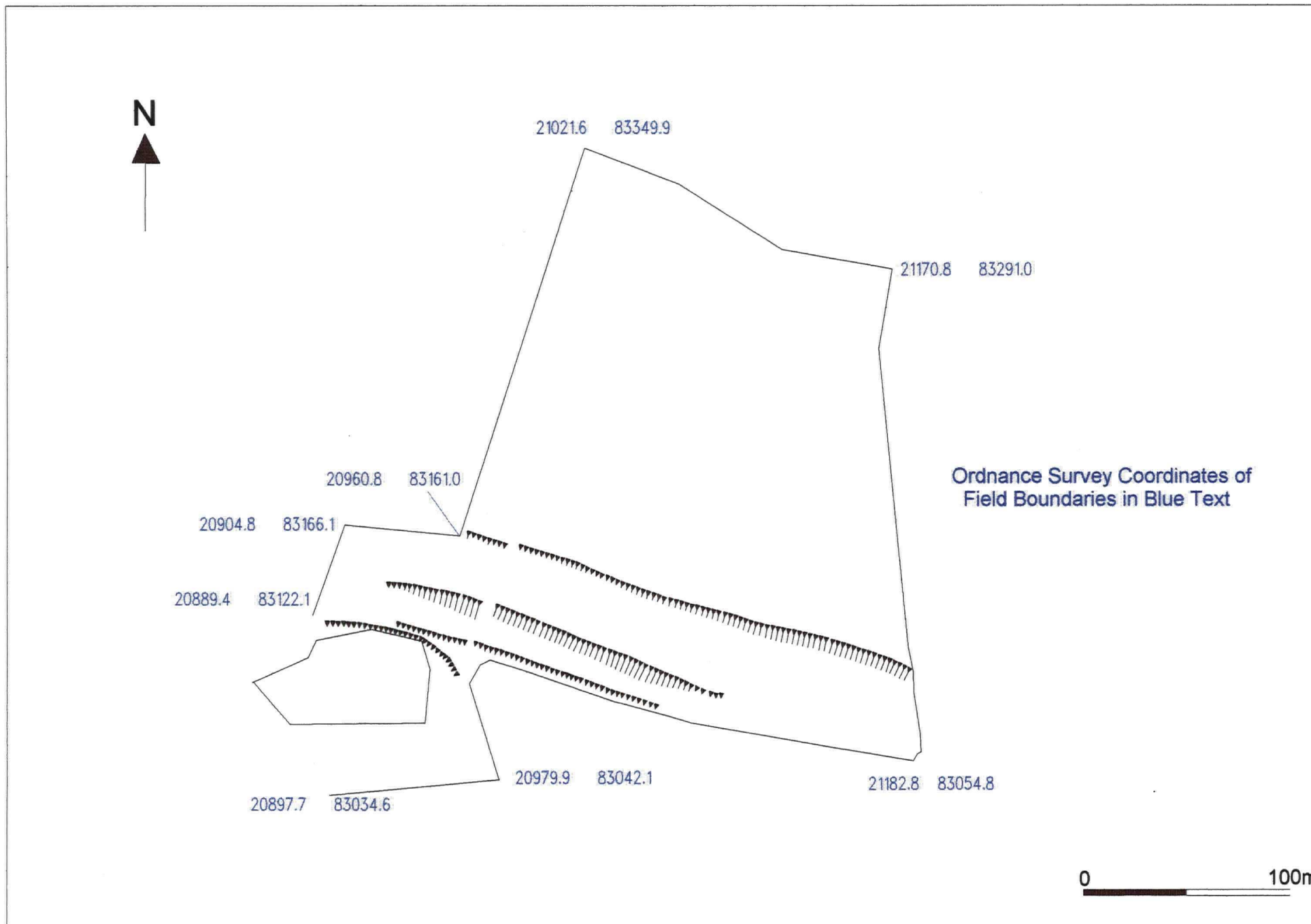
Figure 6: Earthwork Survey. Scale 1:2500
