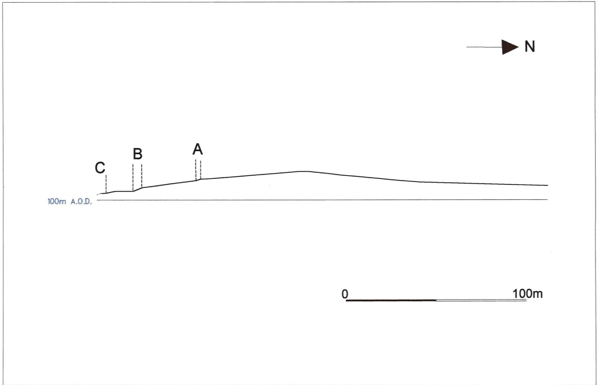
Figure 9: Section Through Earthworks. Scale 1:1250
