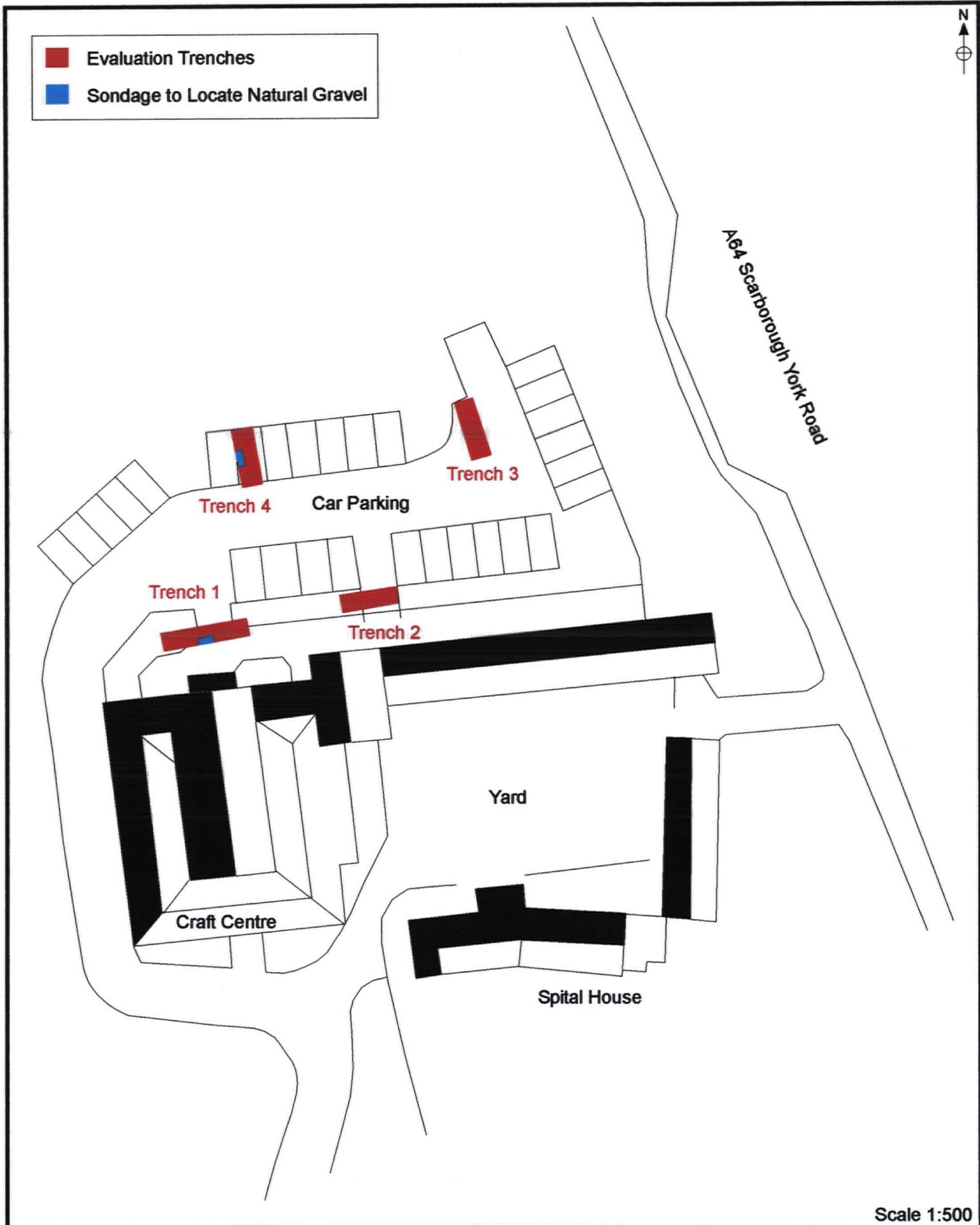
Figure 2. Trench Location
