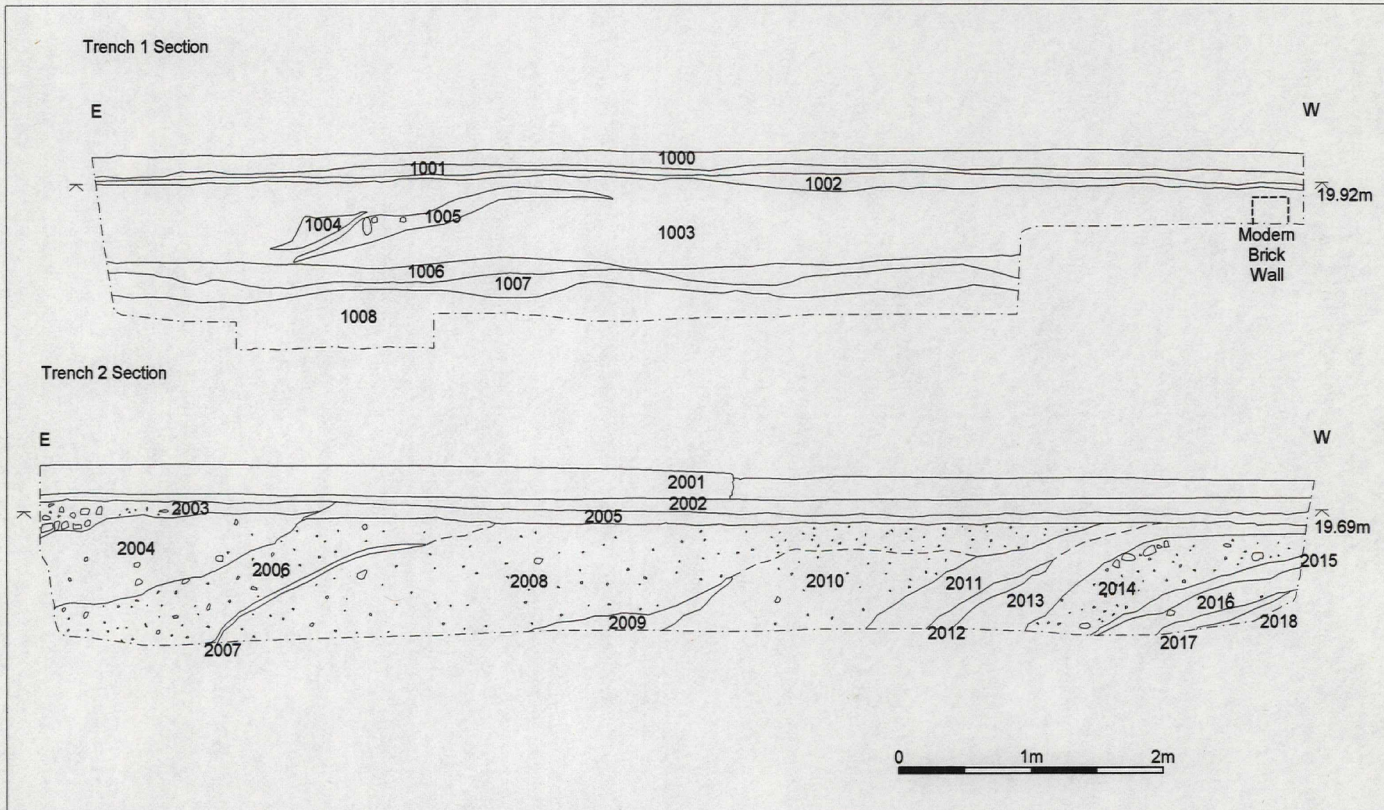
Figure 14. Trenches 1 and 2 Sections.
