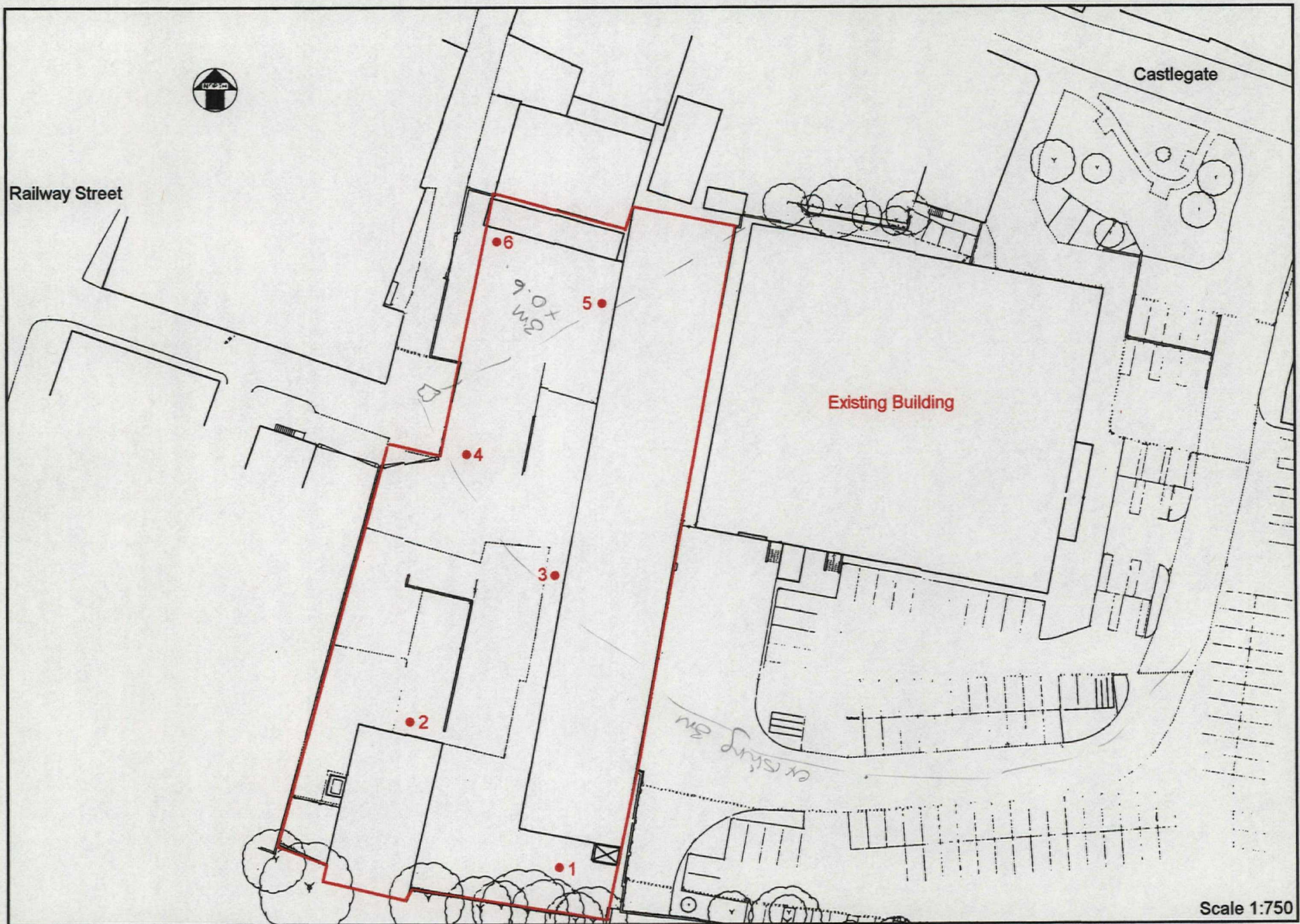
Figure 20. Location of Boreholes.
