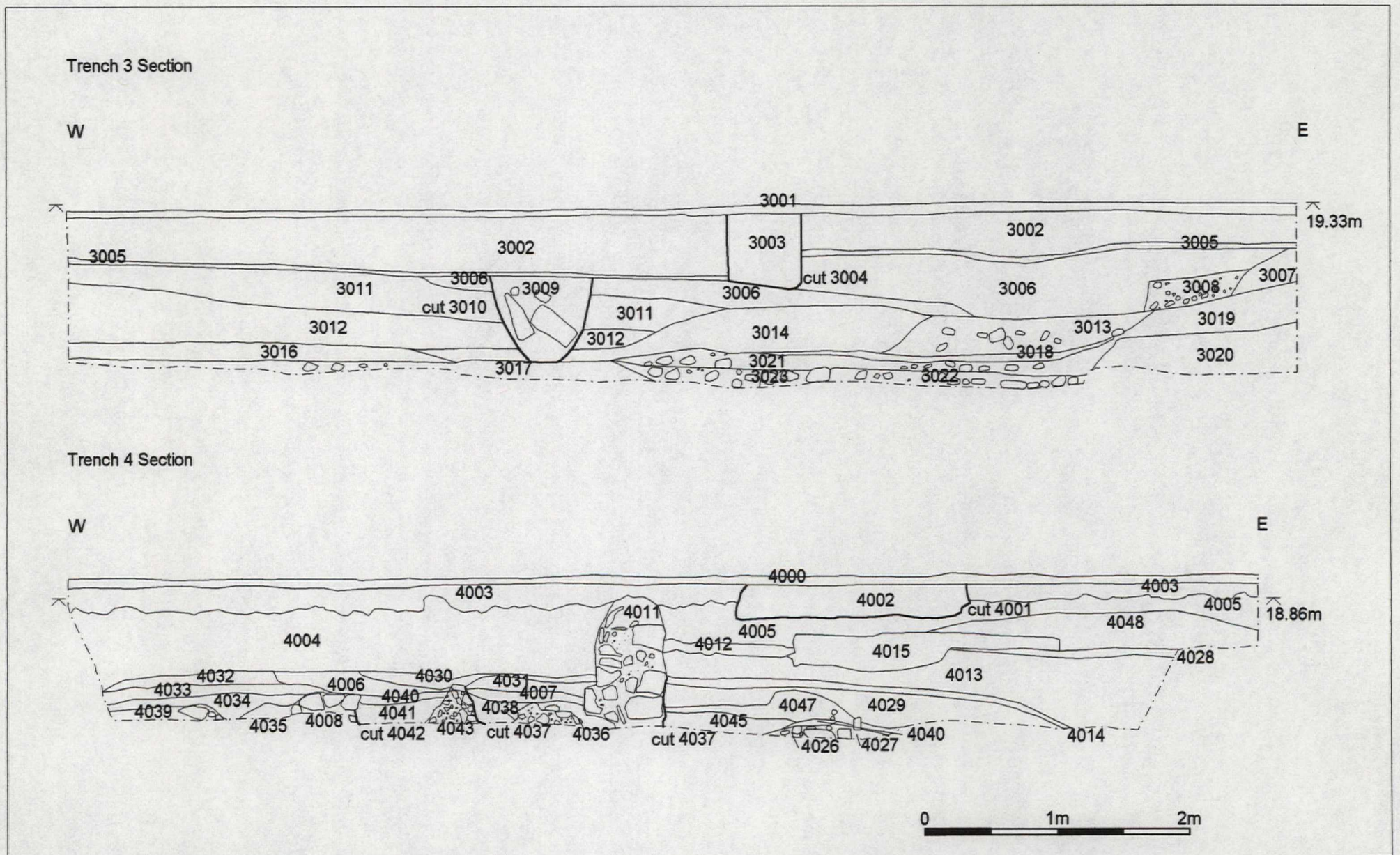
Figure 16. Trenches 3 and 4 Sections.
