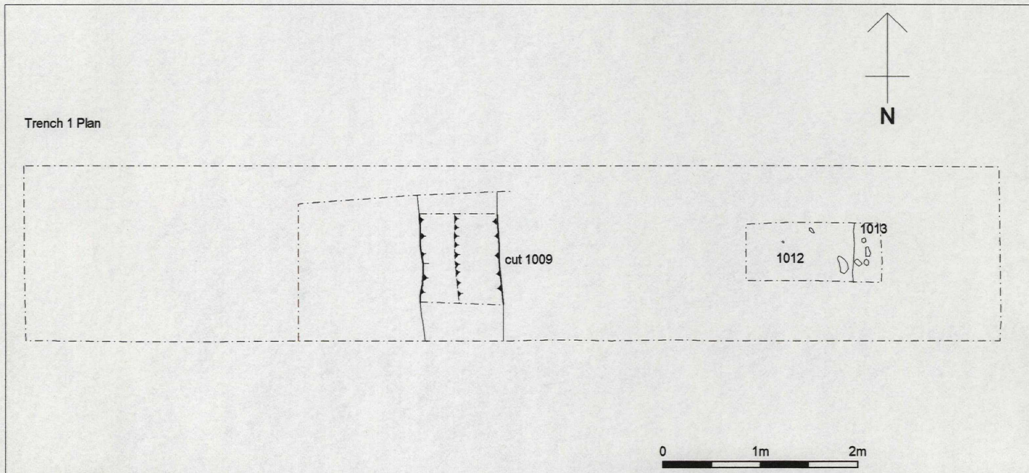
Figure 13. Trench 1 Plan.
