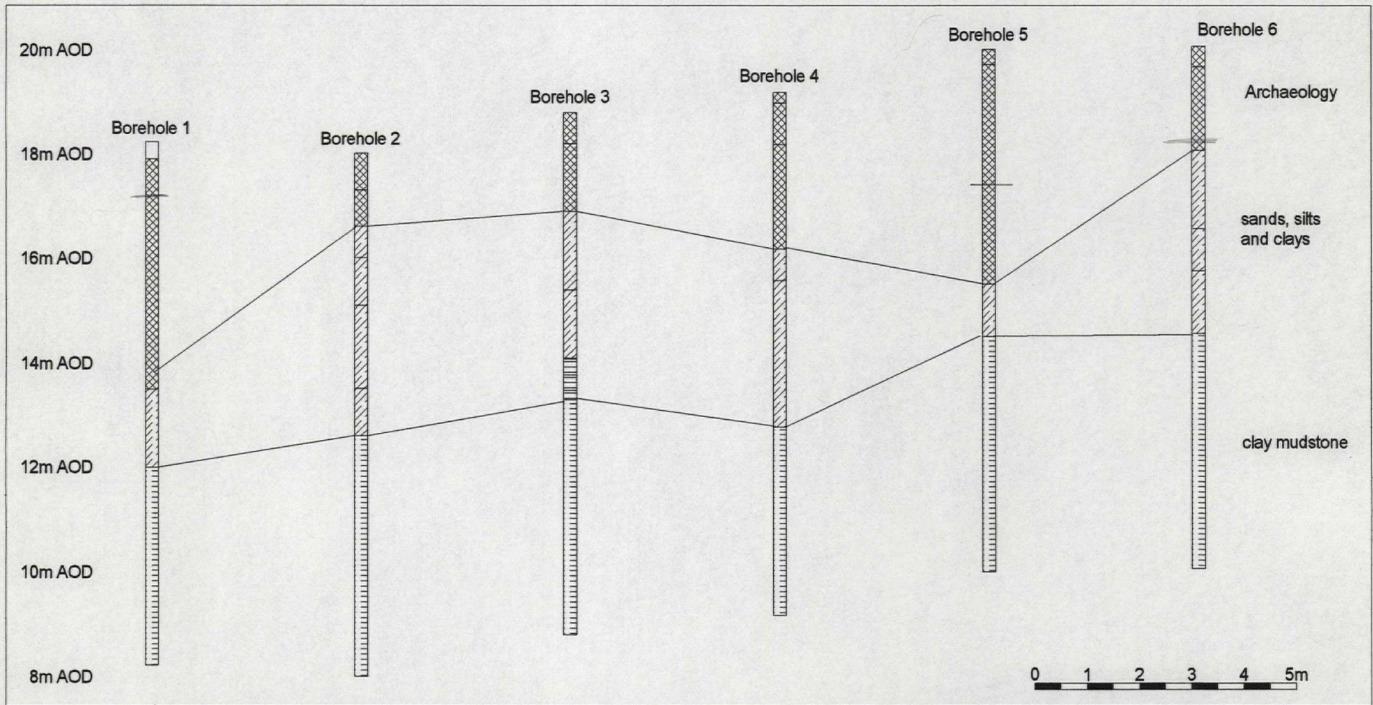
Figure 21. Bore Hole Soil Descriptions (after Hymas).
