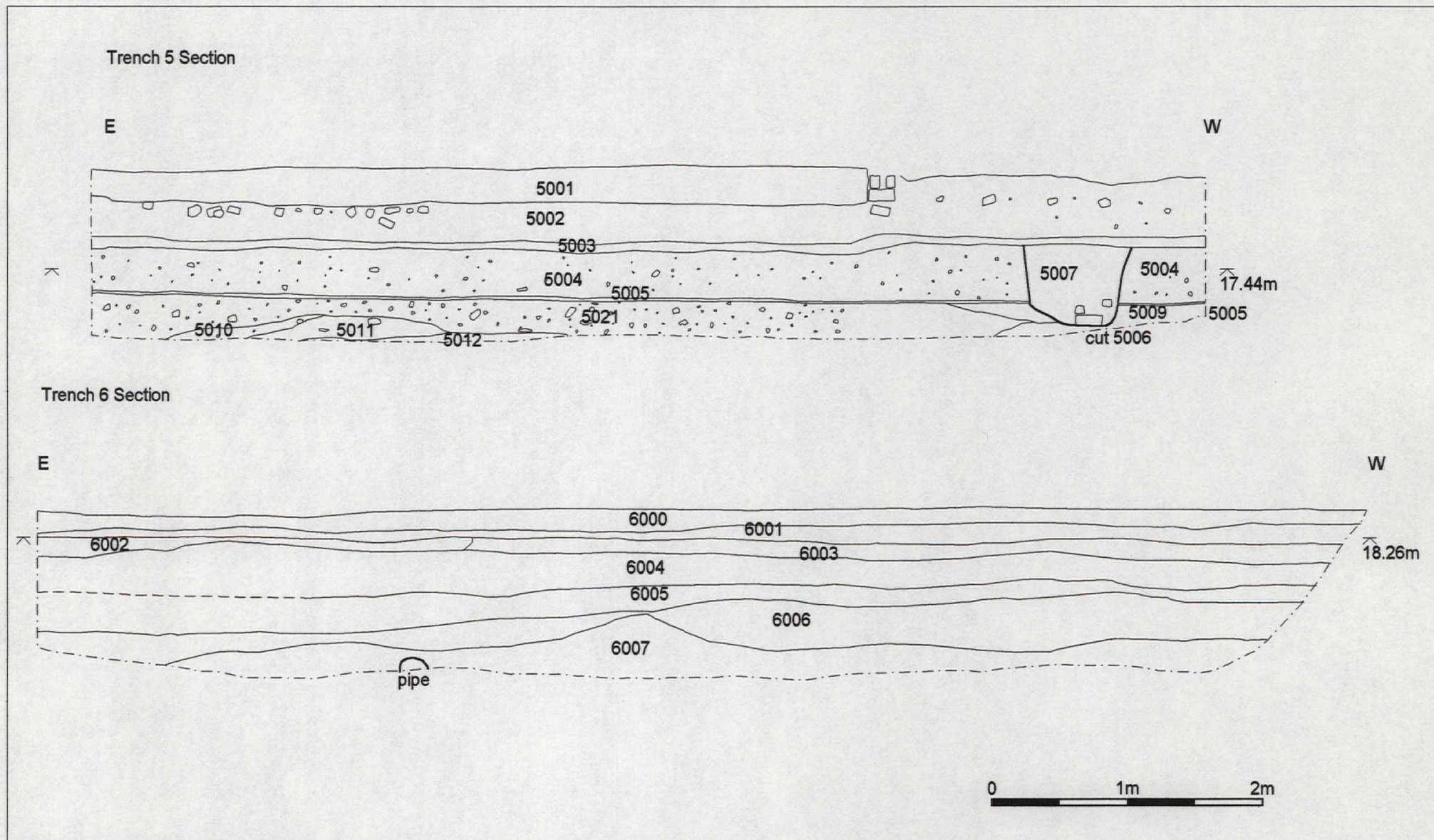
Figure 18. Trenches 5 and 6 Sections.
