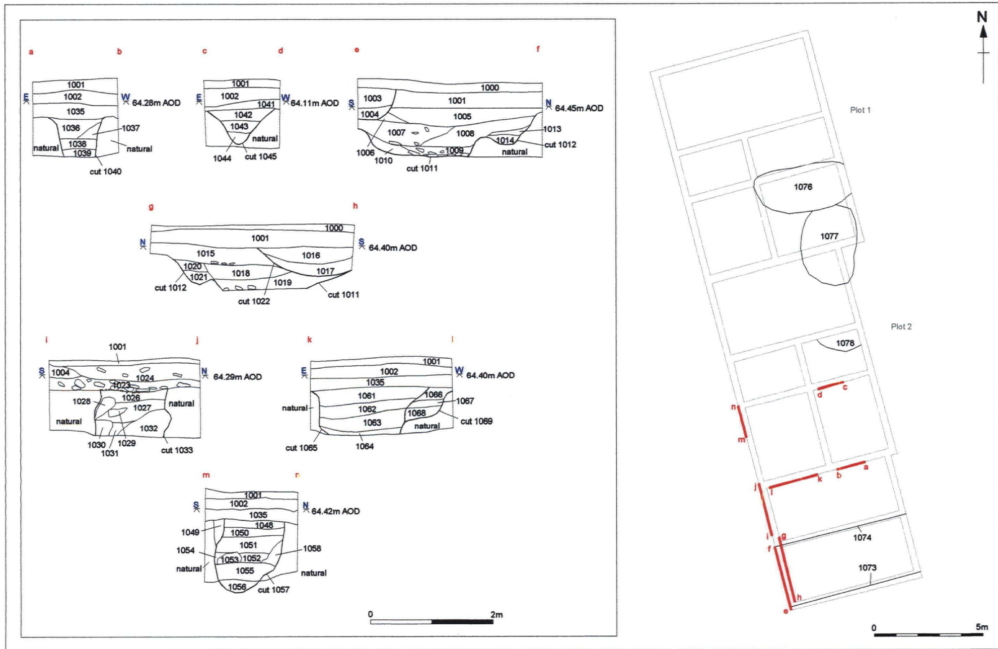
Figure 4. Plan and Sections of Plots 1 and 2 Features
