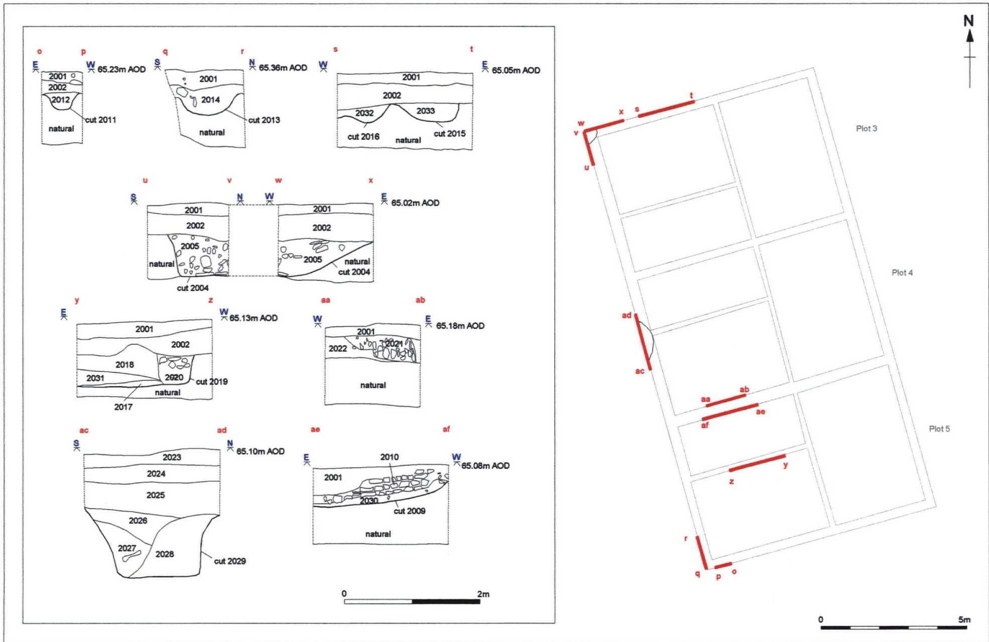
Figure 5. Plan and Sections of Plots 3, 4 and 5 Features
