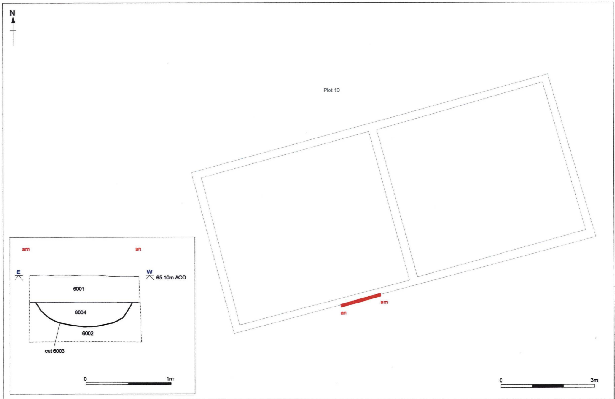
Figure 8. Plan and Section of Plot 10 Feature
