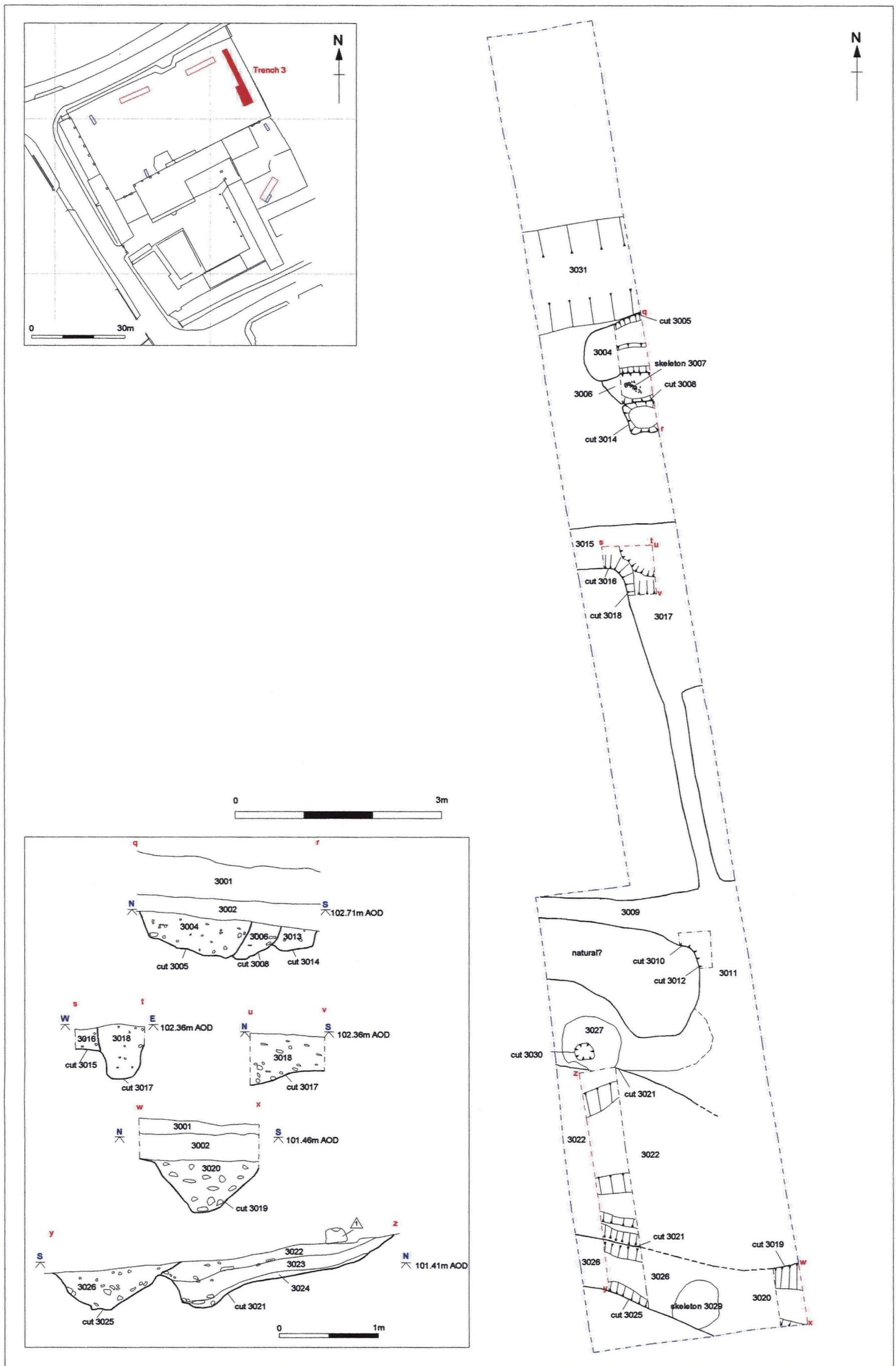
Figure 5. Plan and Sections of Trench 3 Features
