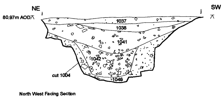
Figure 5. Sections
