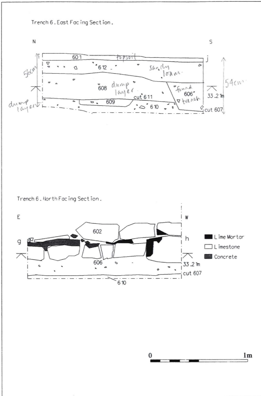
Figure 9 . Trench 6 Sections .
