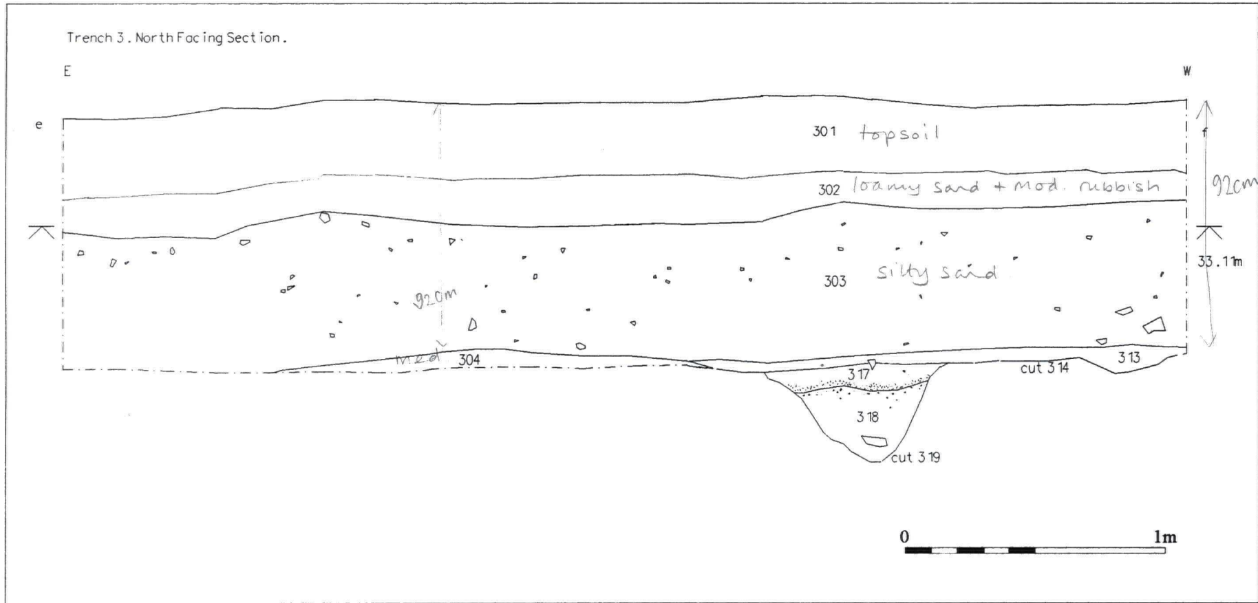
Figure 8. Trench 3. Section.
