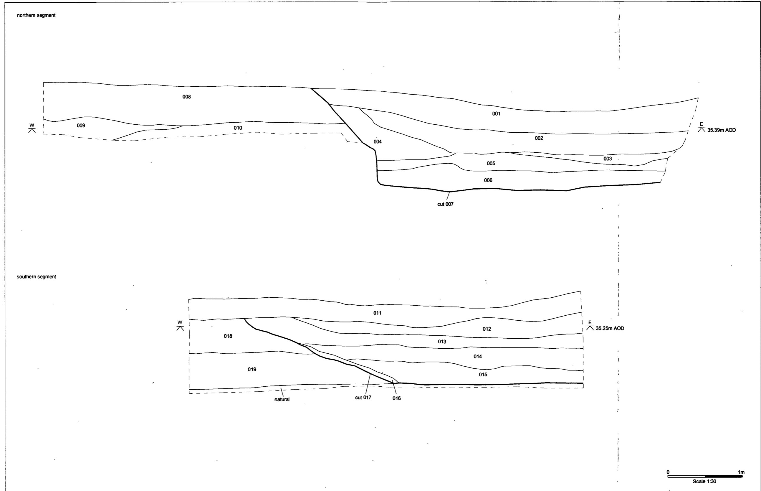
Figure 7. Ditch Sections
