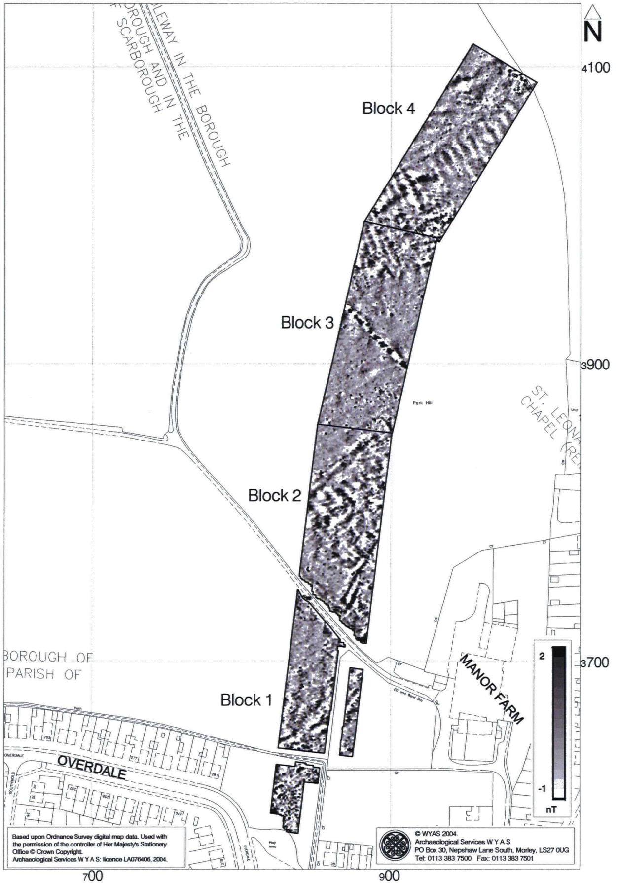
Fig. 3. Greyscale plot of gradiometer data; Site 1
