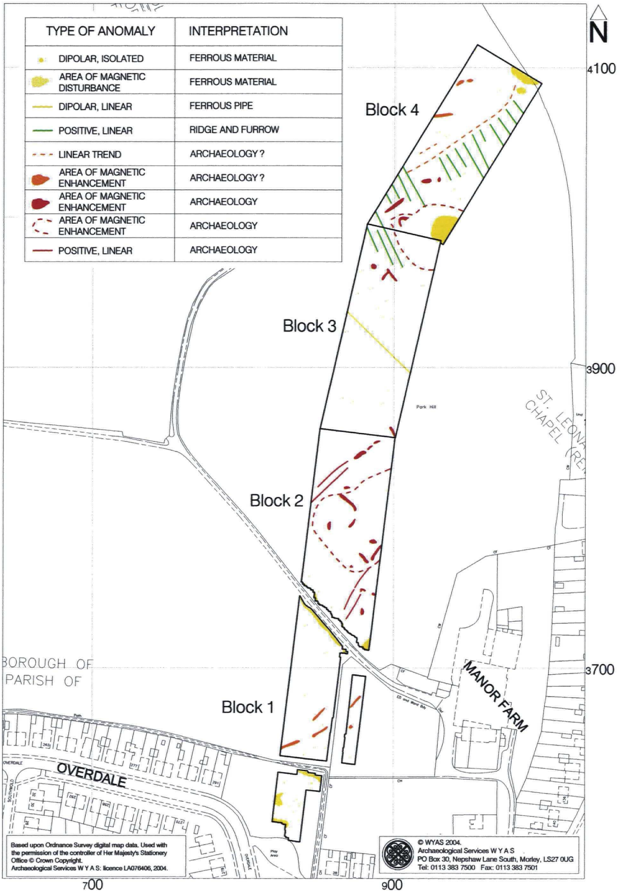
Fig. 4. Interpretation of gradiometer data; Site 1
