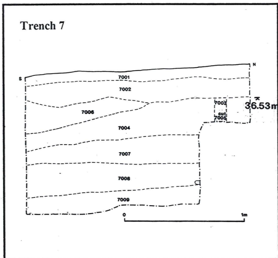
Figure 19. Trench 7. East facing section.
