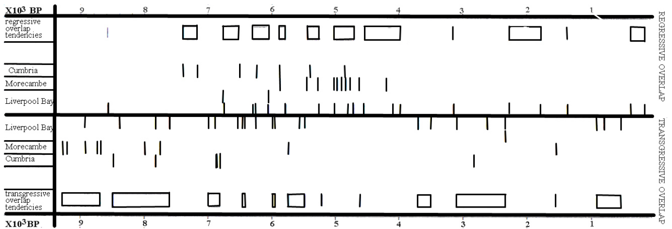
Figure 1. Transgressive and regressive overlap tendencies from sites in Cumbria (including the Isle of Man), Liverpool Bay and Morecambe Bay. Each bar is an uncorrected radiocarbon date from transgressive and regressive overlaps or from sand dune paleosols. For the whole of North West England these can be resolved into 12 transgressive and 12 regressive overlap tendencies, represented by the rectangles (summarized from Tooley, 1982).
