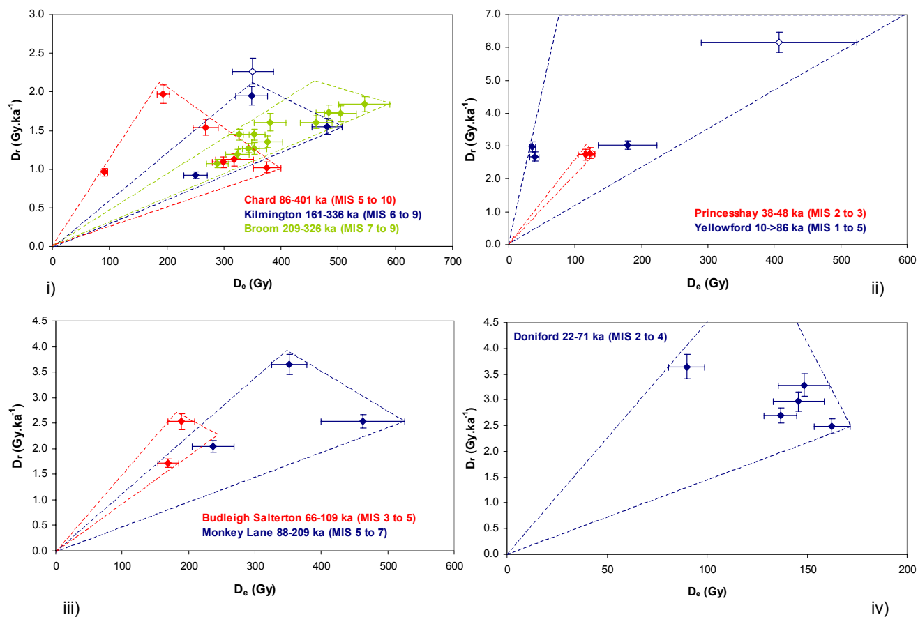
Figure 10: Age envelopes for site deposits of the former i) Axe, ii) Exe, iii) Otter, and iv) Doniford Rivers
