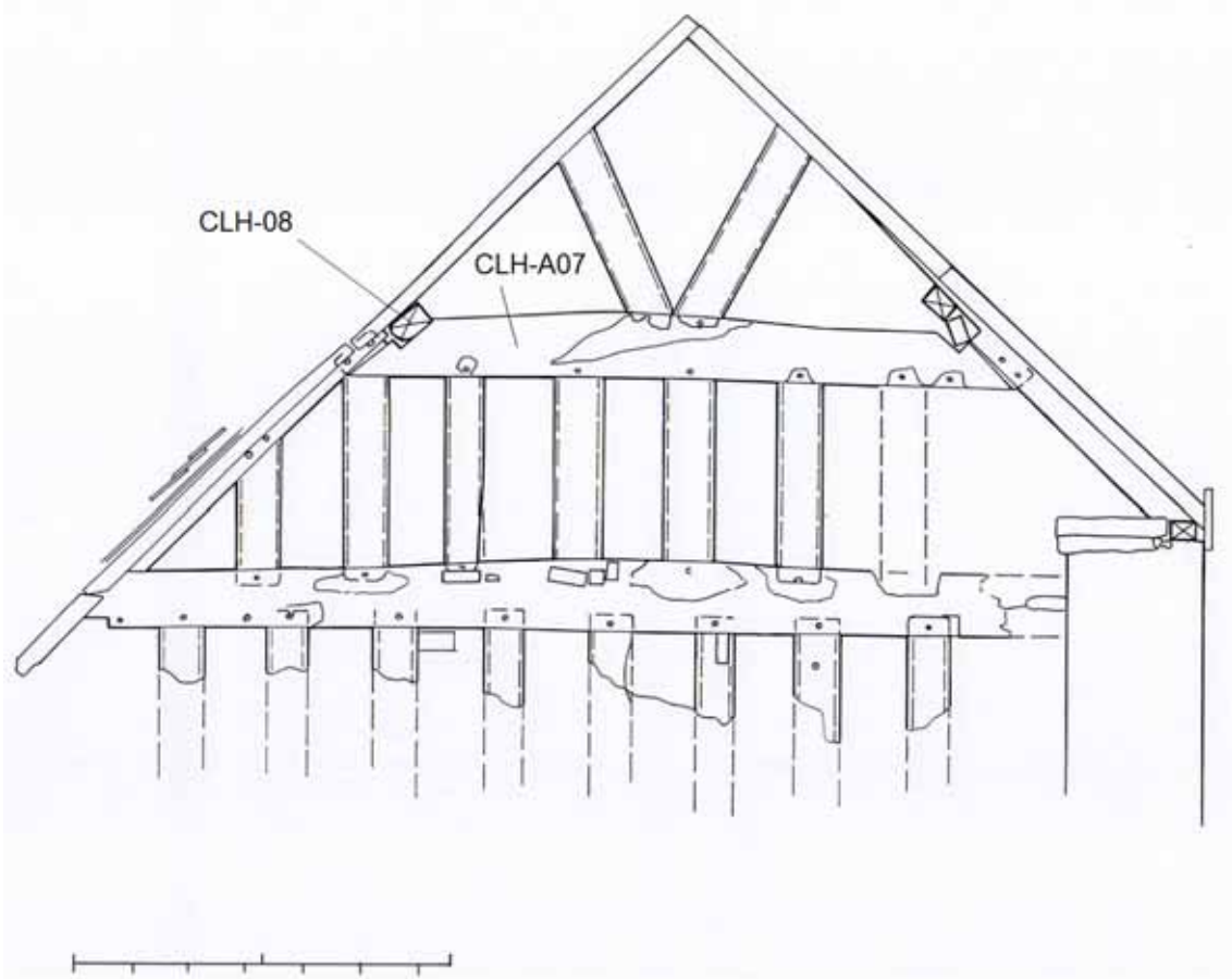
Figure 8: North gable truss (north face); showing the location of samples CLH-A07 and CLH-A08 (Bob Meeson)
