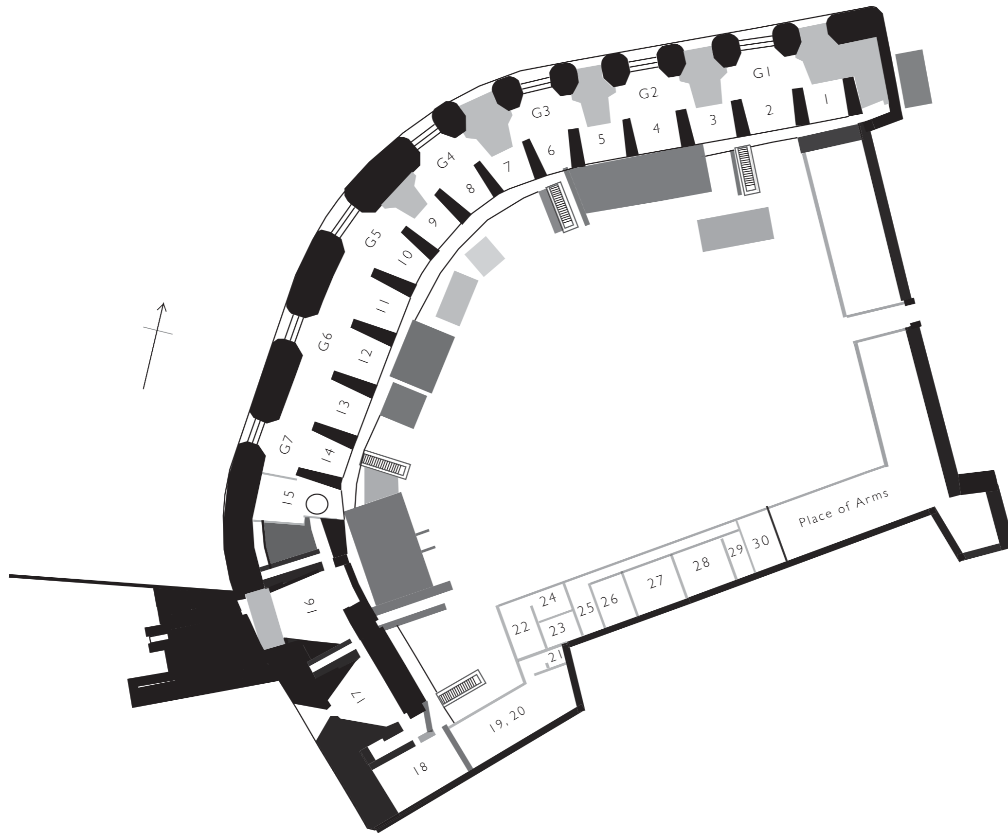
Appendix Figure 5: Gun floor plan with areas numbered as mentioned in the text. Based on Thames Defences: Cliffe Fort: Plan of Gun Floor 1899 ©The National Archives: WO78/4963
