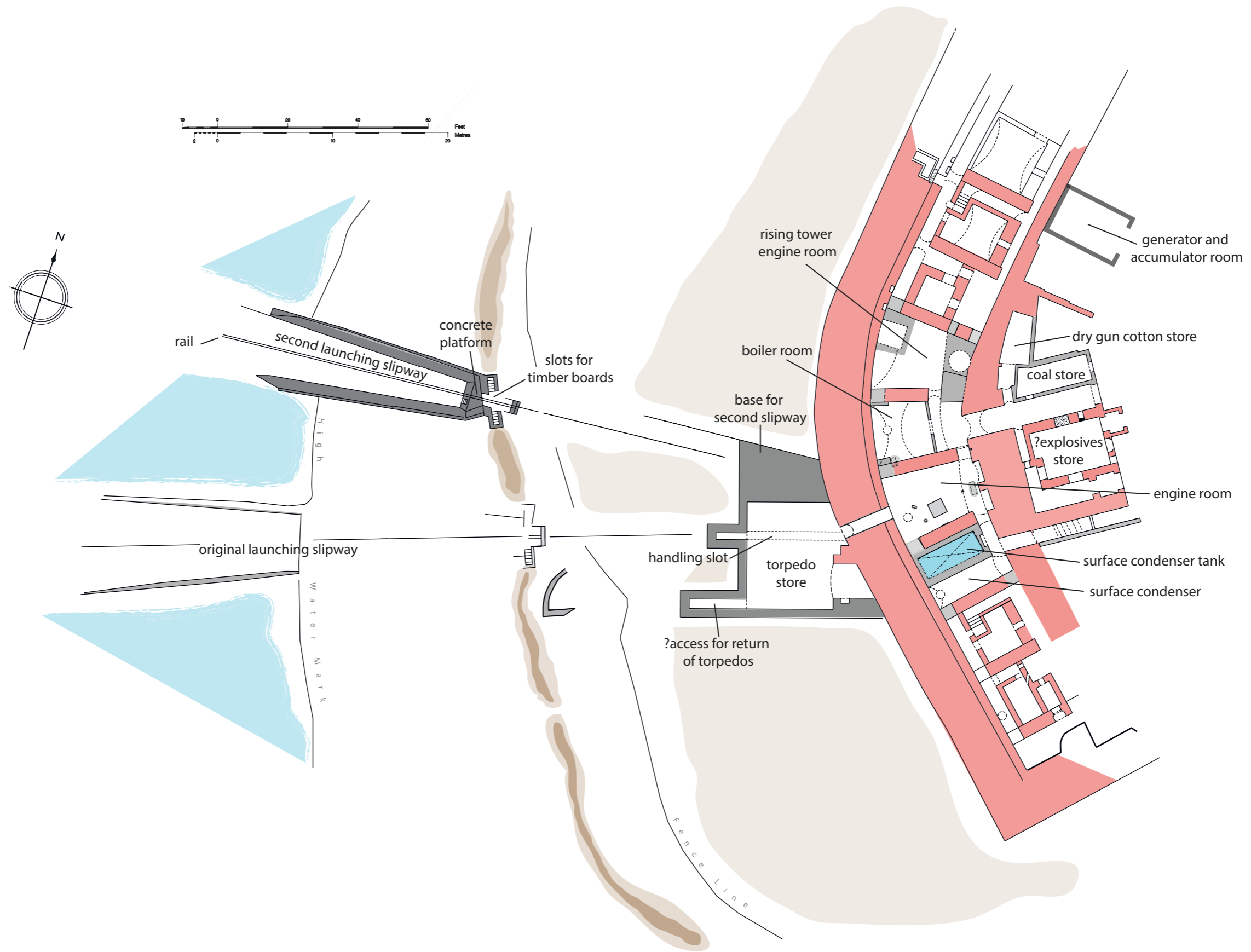
Appendix Figure 6: Sketch plan of basement level of Brennan Torpedo Installation based on information detailed in this report, Pattison (1993) and TNA: WO78/4963. (NB Original fort fabric in red, additions for the Brennan Torpedo in grey, dotted lines indicate overhead detail).
