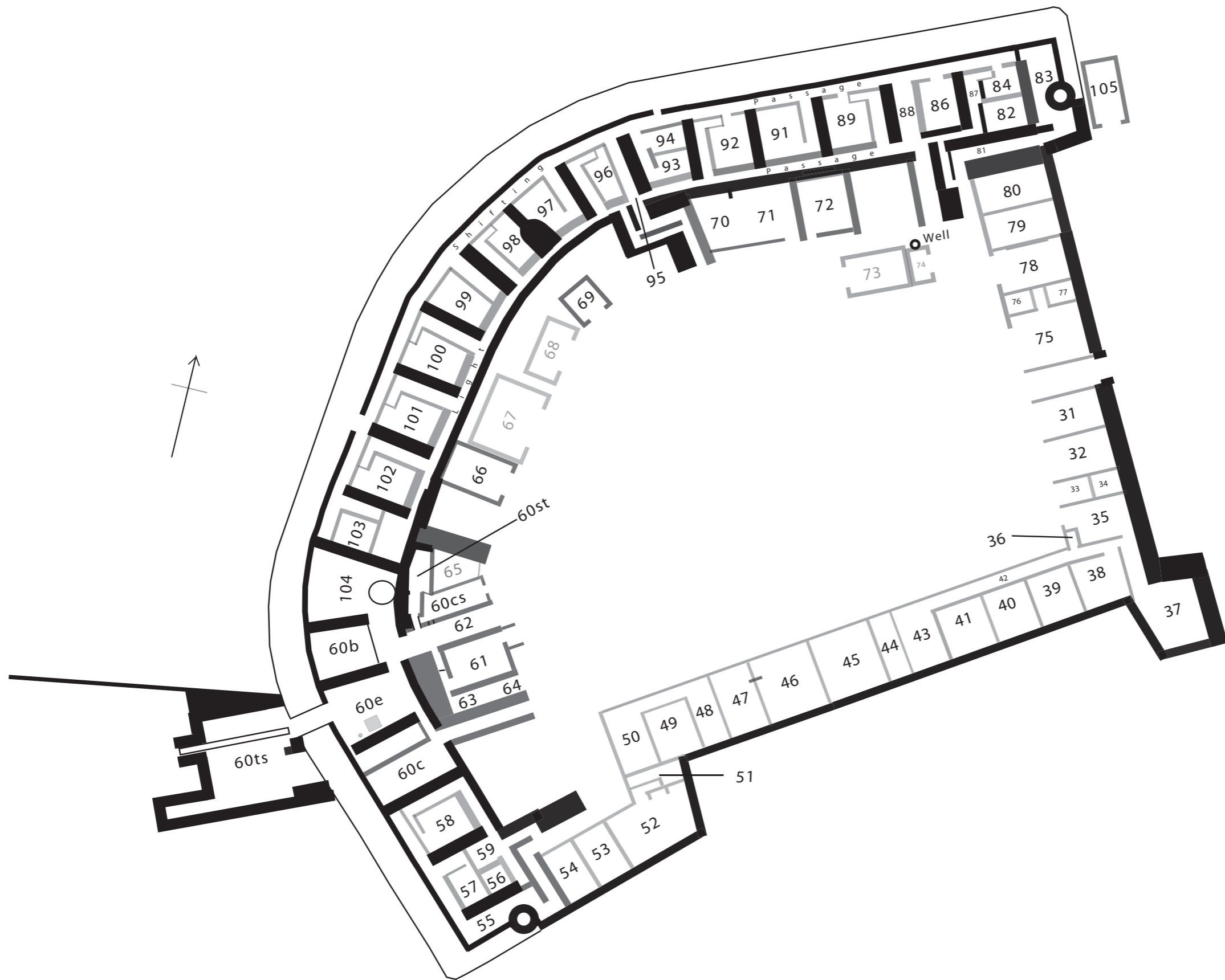
Appendix Figure 4: Basement plan with rooms numbered as mentioned in the text based on Thames Defences: Cliffe Fort: Plan of Magazines, Drains etc 1899 ©The National Archives: WO78/4963
