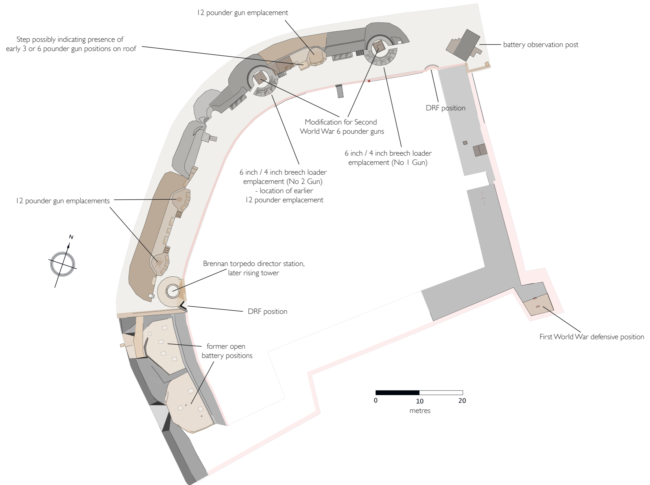
Appendix Figure 8: Plan of roof based on measured survey and the 1899 plan (TNA: WO78/4963). (NB Original and mid-19th century fabric in grey and pink, 12 pounder battery in brown, Brennan installation in cream, 6 inch battery in dark grey, Second World War additions in dark brown, areas of measured survey outlined in black).
