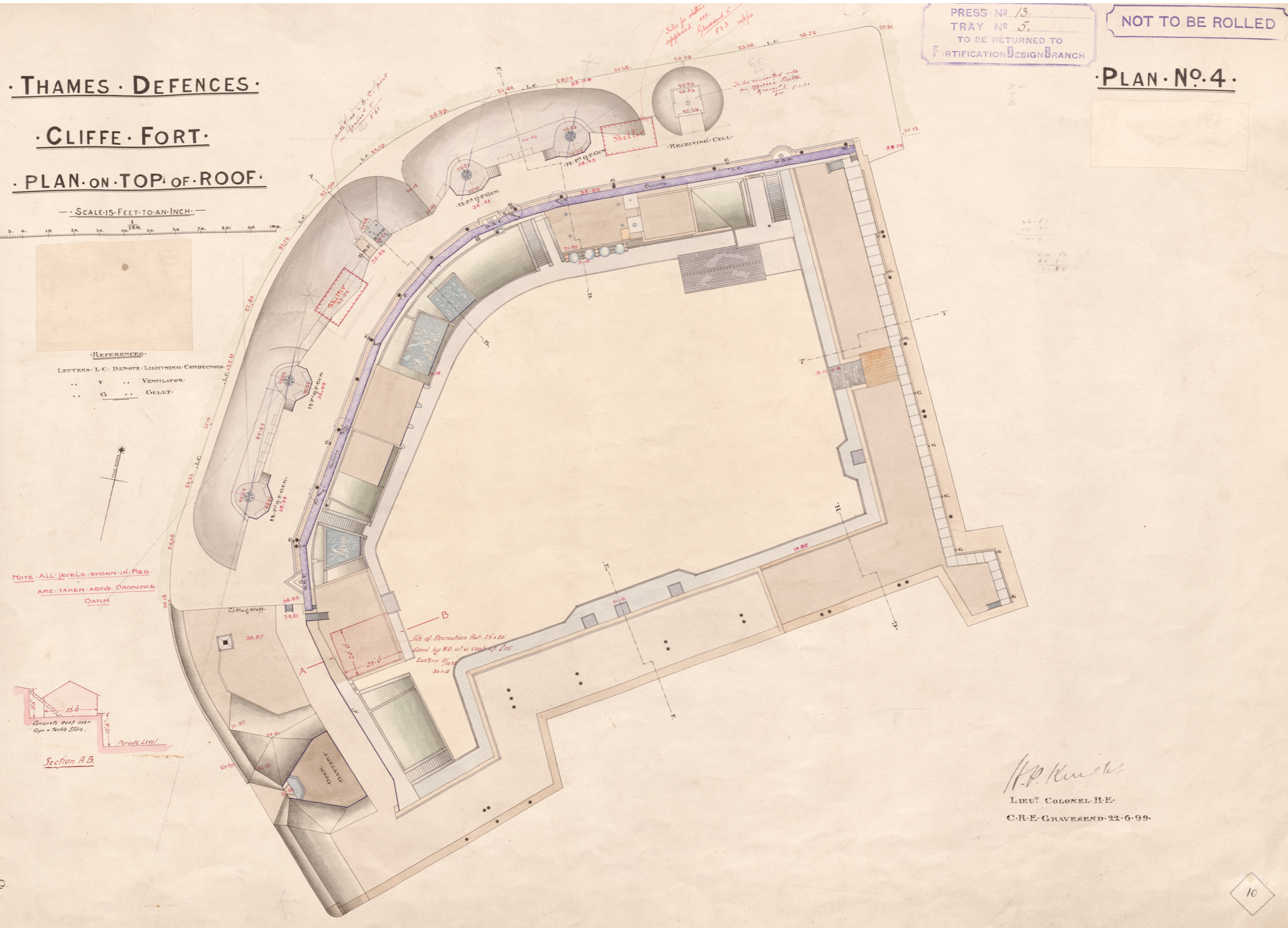
Appendix Figure 3: Thames Defences: Cliffe Fort: Plan on Top of Roof 1899 ©The National Archives: WO78/4963
