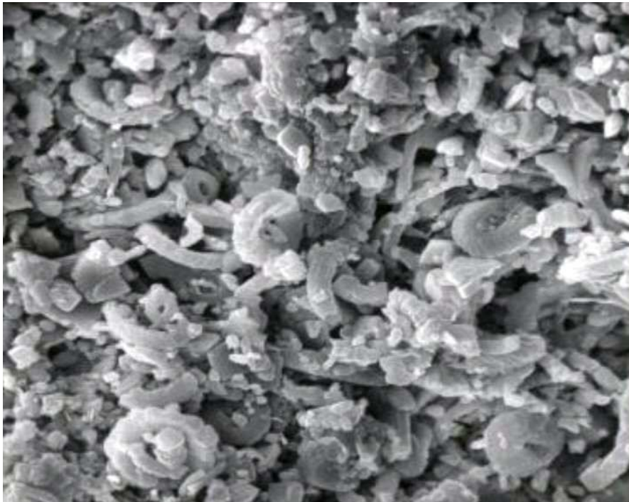
Figure 6: SEM photograph of the Chalk, which is composed of microfossil rings (up to 10µm in diameter).
