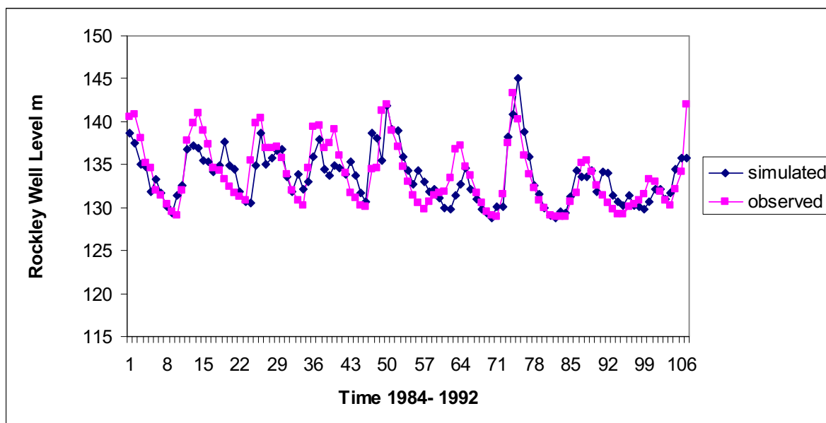
Figure 3: Simulated and observed Rockley well levels using the IHACRES model
