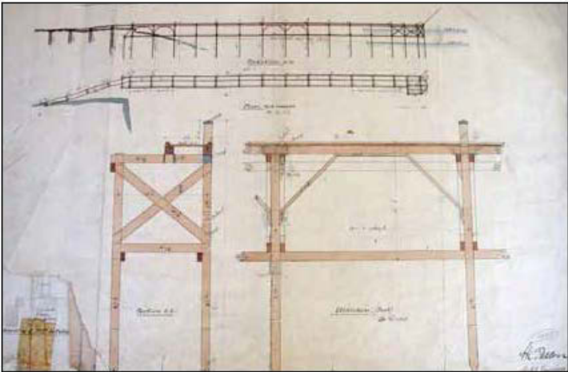
Figure 20. 1880's plan for the east jetty extension (EHA MD 95/6482)
