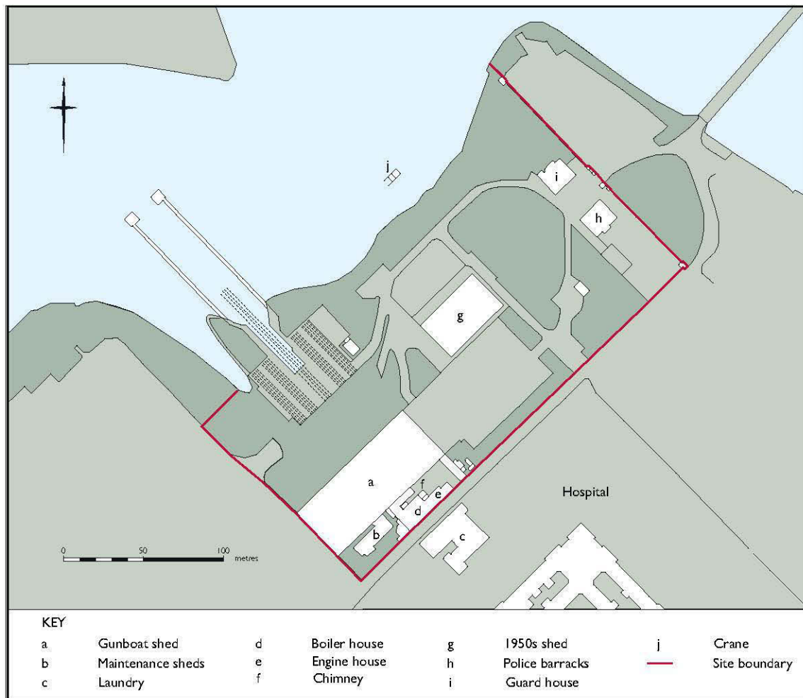
Figure 26. Site plan
