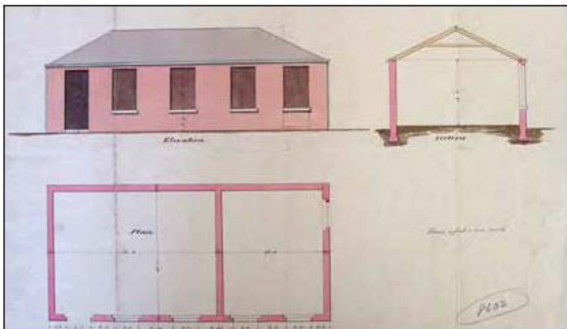
Figure 10. Plan for a storehouse, 1859 (EHA MD 9516503)
