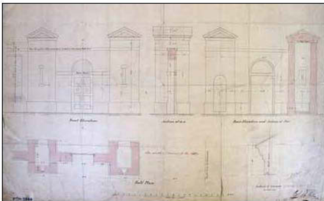
Figure 13. Plan and section of entrance gateway (EHA MD 95/6512)
