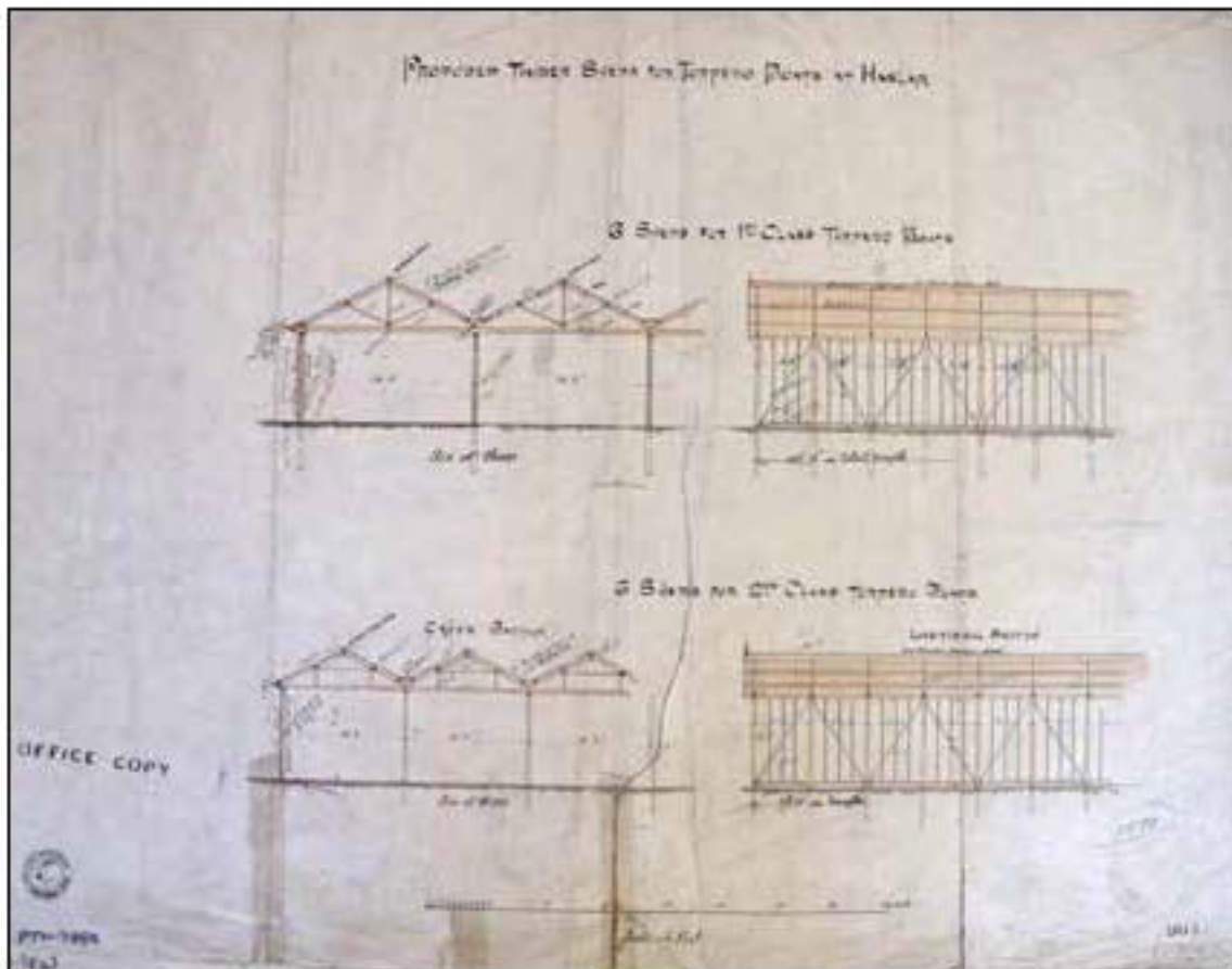
Figure 9. Mid-19th century plan of sheds for torpedo boats (EHA MD 9516505)
