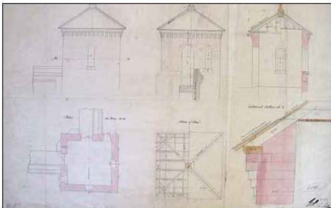
Figure 17. Late 19th century plan of the sentry towers (EHA MD 9516516)
