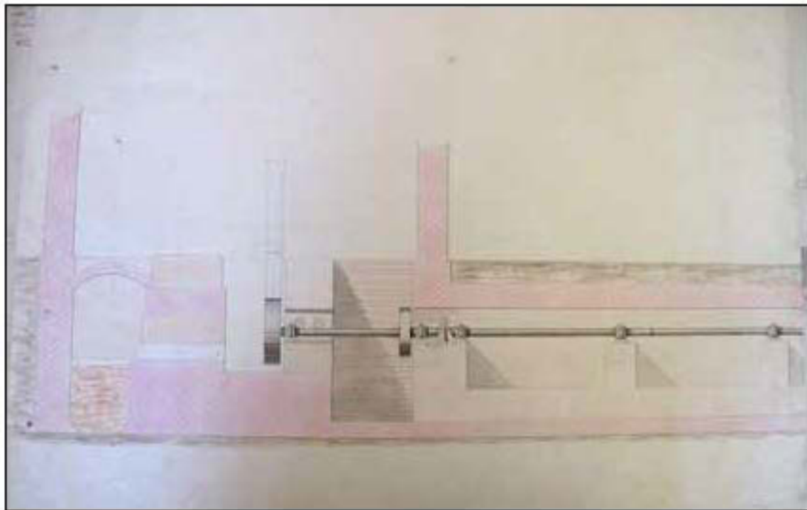
Figure 12. Section through tunnel connecting the boiler house to Haslar laundry (EHA MD9512798)
