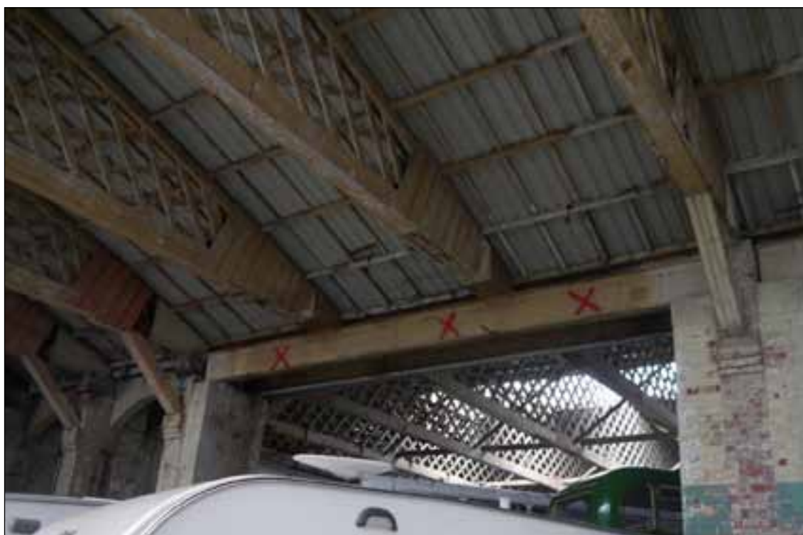
Figure 24: Central arcade showing where the arches have been removed and replaced by an RSJ, Building 17 (© English Heritage, photograph: Simon Taylor).
