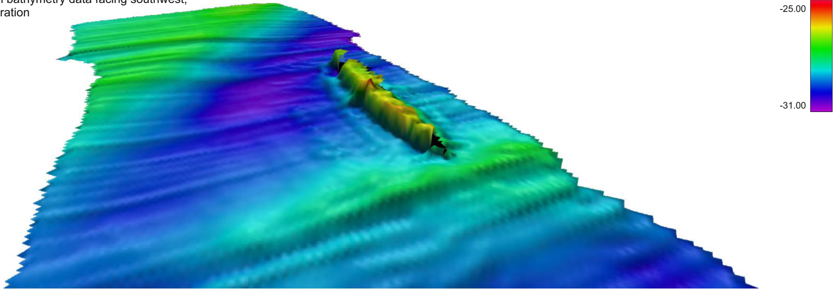
B. 2007 CHP multibeam bathymetry data facing southwest, 1x vertical exaggeration
