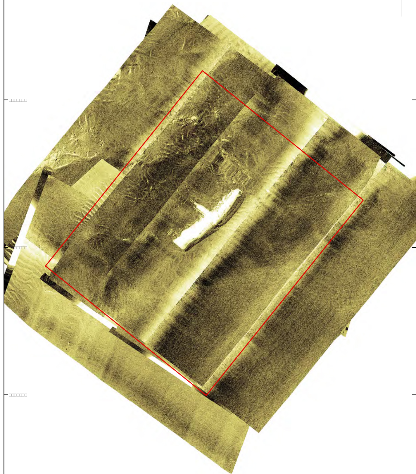
A. Sidescan sonar mosaic
