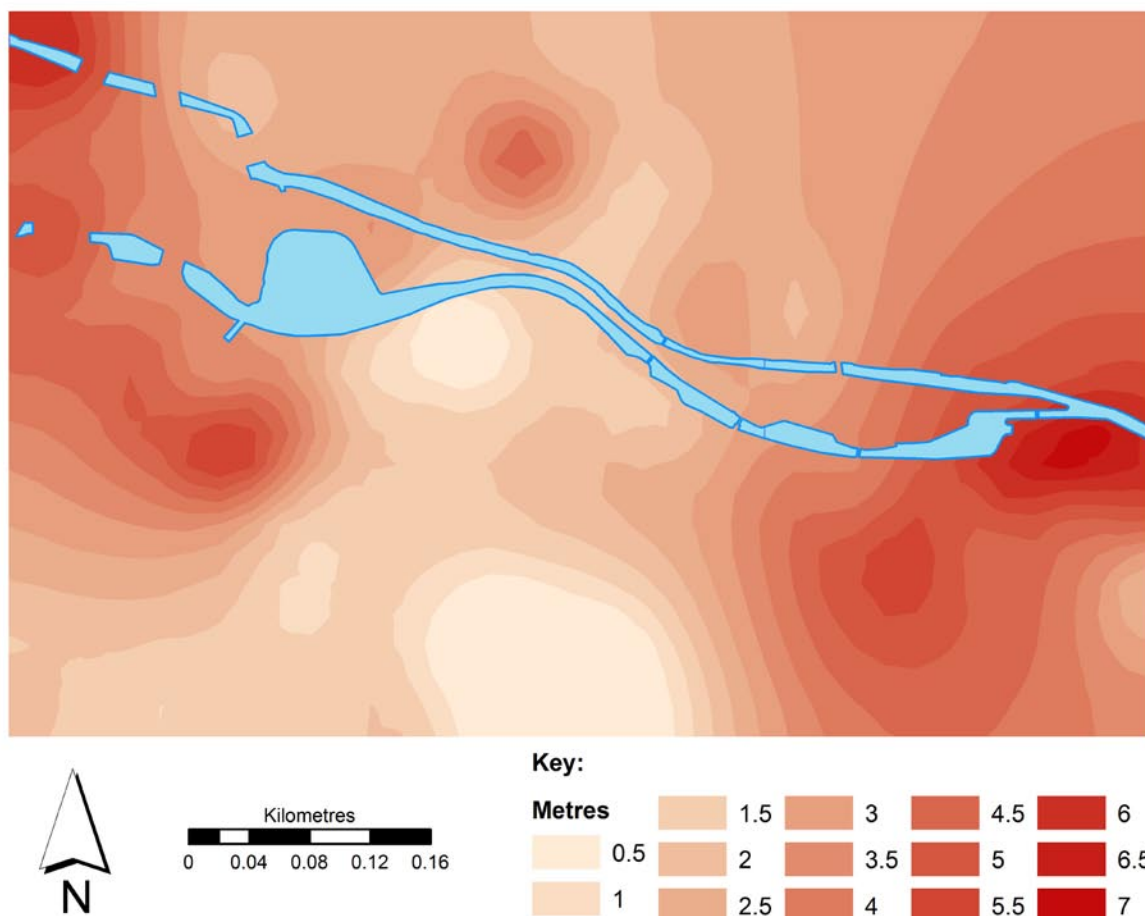
Figure 10. Core survey area: thickness of Quaternary deposits. The plot indicates major areas of Quaternary deposits to the east and the west with a small area in the centre (north side). To the east this coincides with a considerable hollow in the underlying Mercia Mudstone surface, and, to the west, with two lesser hollows. The small central (north side) deposit may be anomalous.
