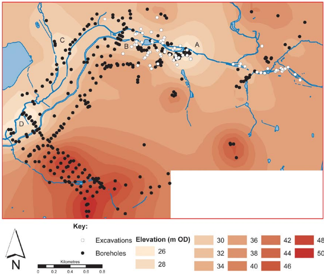
Figure 4. Surface modelling of the underlying Mercia Mudstone geology, which shows an apparent succession of hollows (A-D) along the base of the Salwarpe valley.
