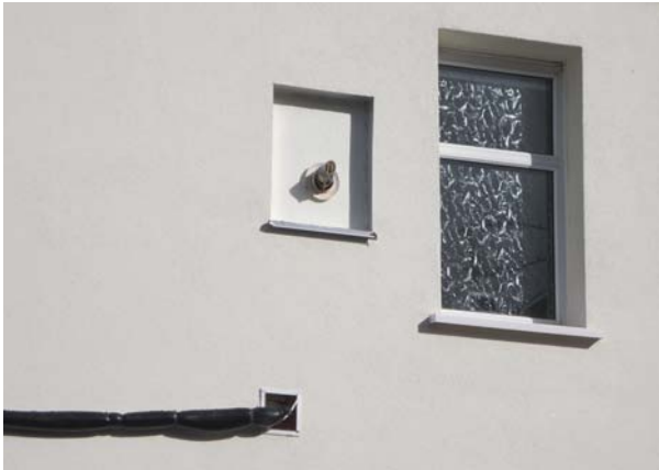
Figures 86 & 87 Uninsulated boiler flue surrounds (note flashing on left vs no flashing on right)
