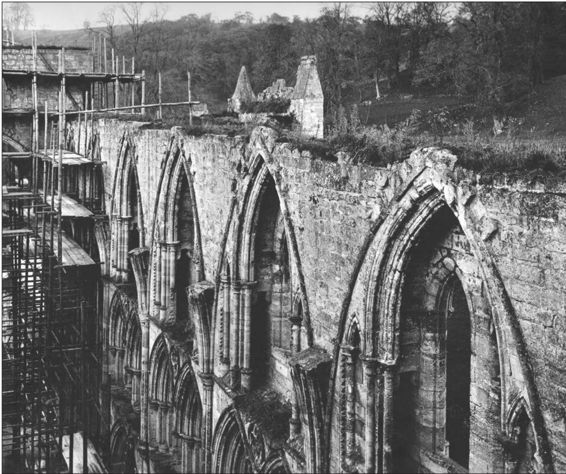
Figure 7.1 An early photograph showing the Church at Rievaulx before the Ministry of Works began consolidation in the early 20th Century. A natural soft capping had developed over the previous 350 years and seems to have provided good protection for the masonry below. Source: Historic England Archive (AL0876_011_01)
