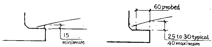
VARIATIONS ON SOFFIT AT DETAIL 'X' (1:5)
