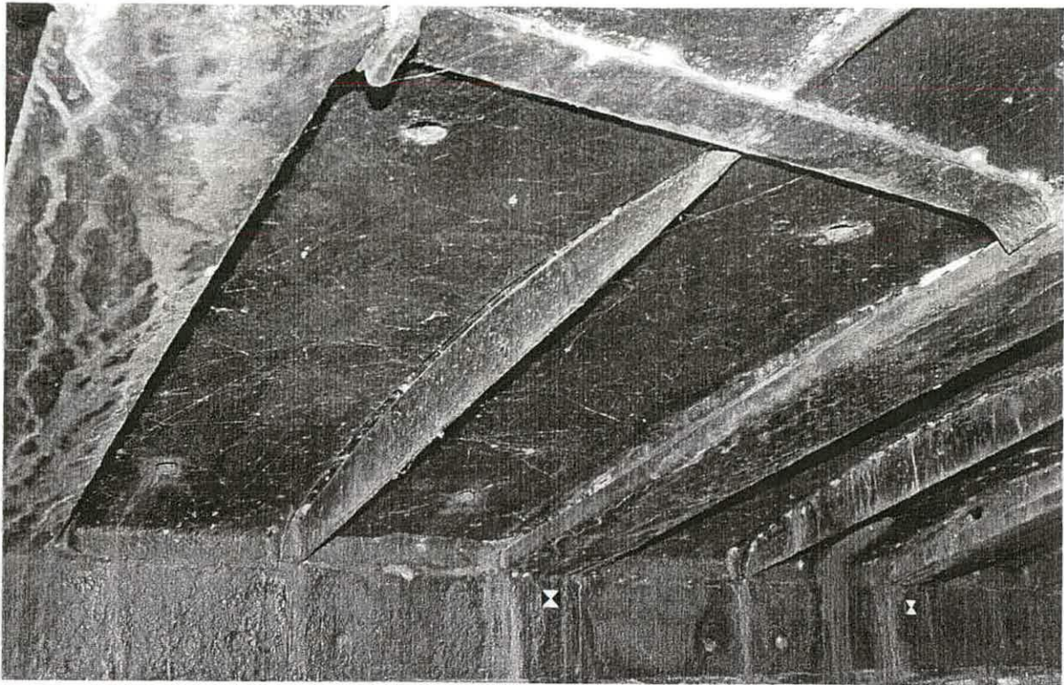
Main span, soffit adjoining seating on SW side
