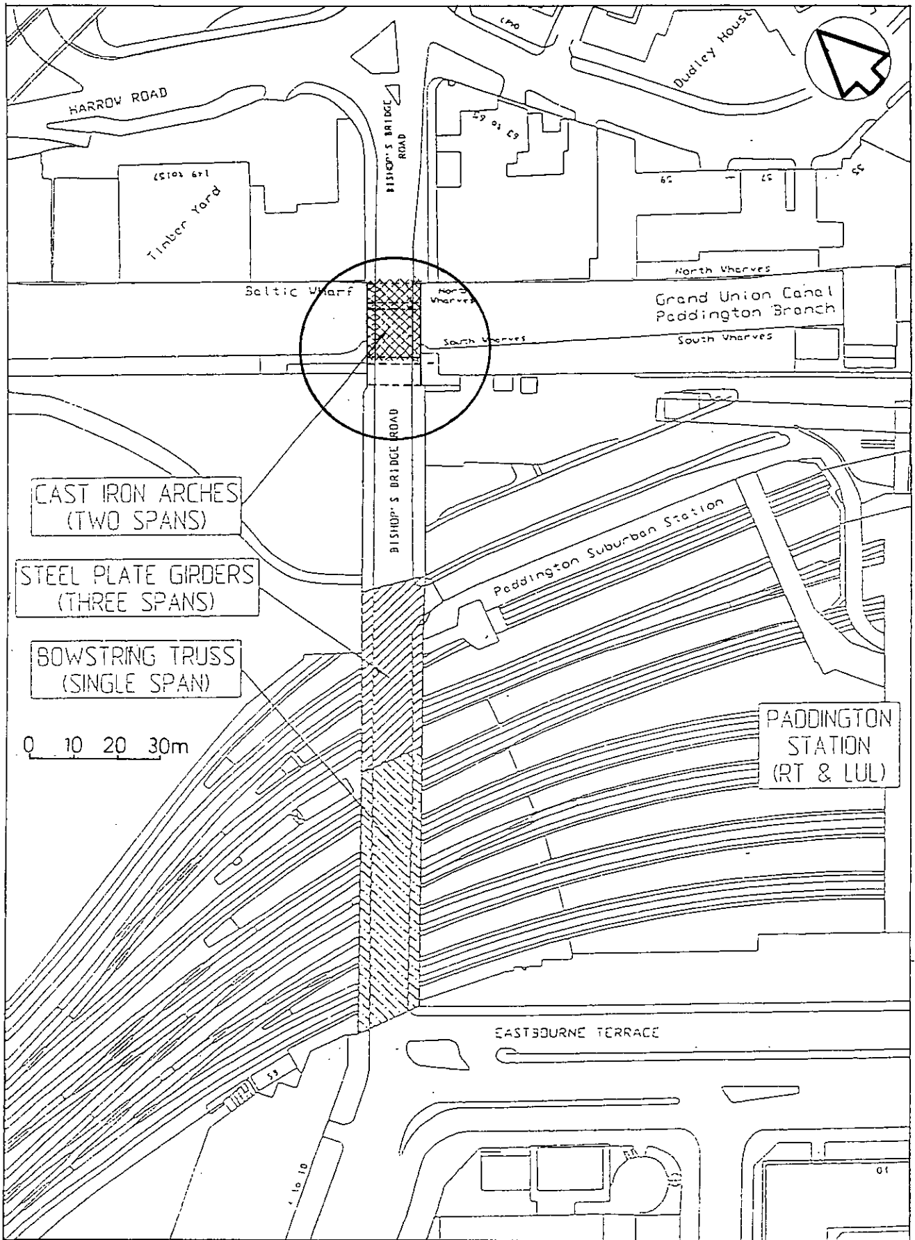
LOCATION PLAN
