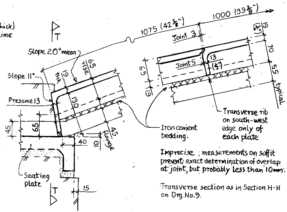
DETAIL 'Y' (1:5)
