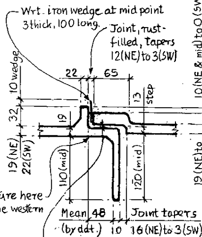
DEVELOPED VIEW ON TOP OF SOFFIT PLATES (1:10)
