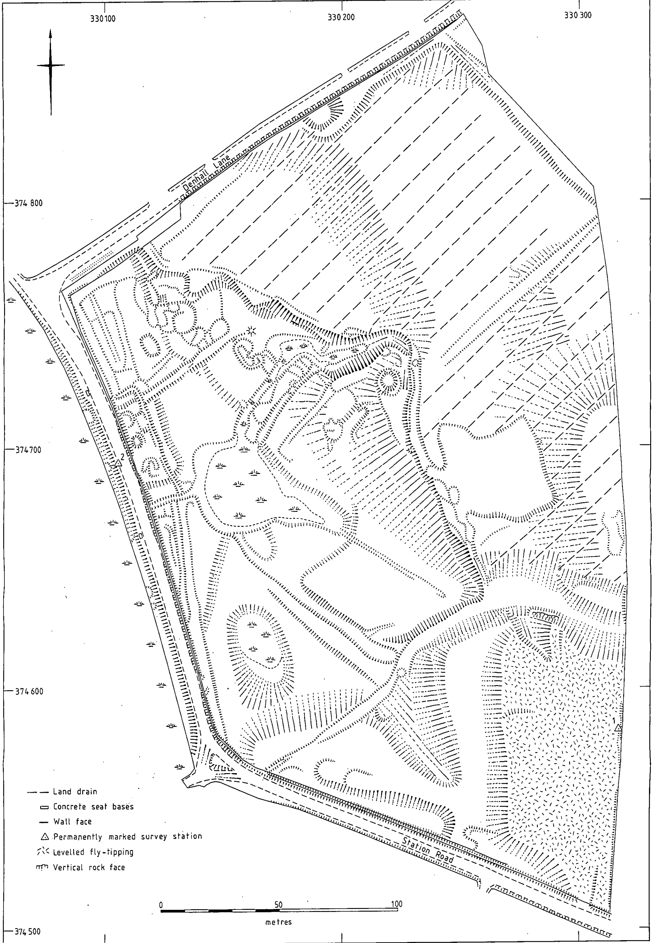
Figure 3. RCHME earthwork plan of Chapel Field at 1:1000 scale
