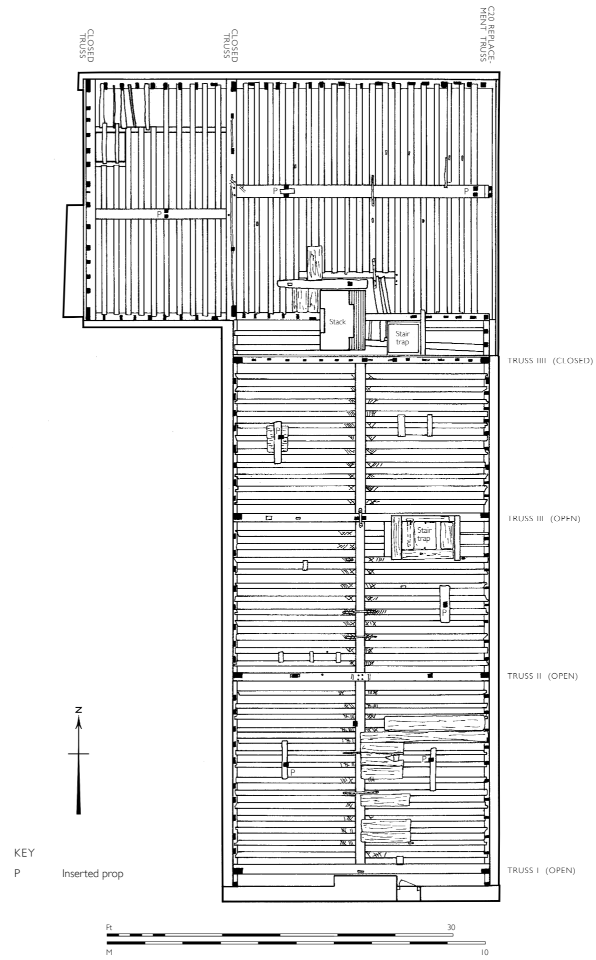
Fig. 69: Floor plan of attic. (Drawing by Linda Hall; © English Heritage).
