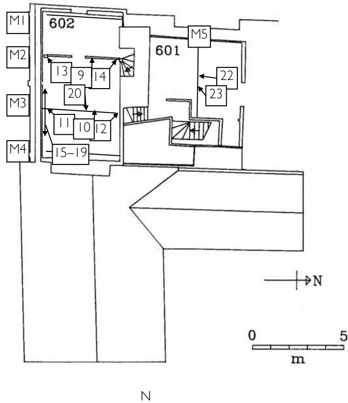
N Figure 9. Plan of Level 6 of Bessie Surtees House showing the location of rooms 601, and 602, the truss numbering scheme assigned to the Milbank House roof trusses M1–M5, and the approximate location and direction of samples 9–20, and 22–23. Based on Figure 9 of Heslop et al (1994)
