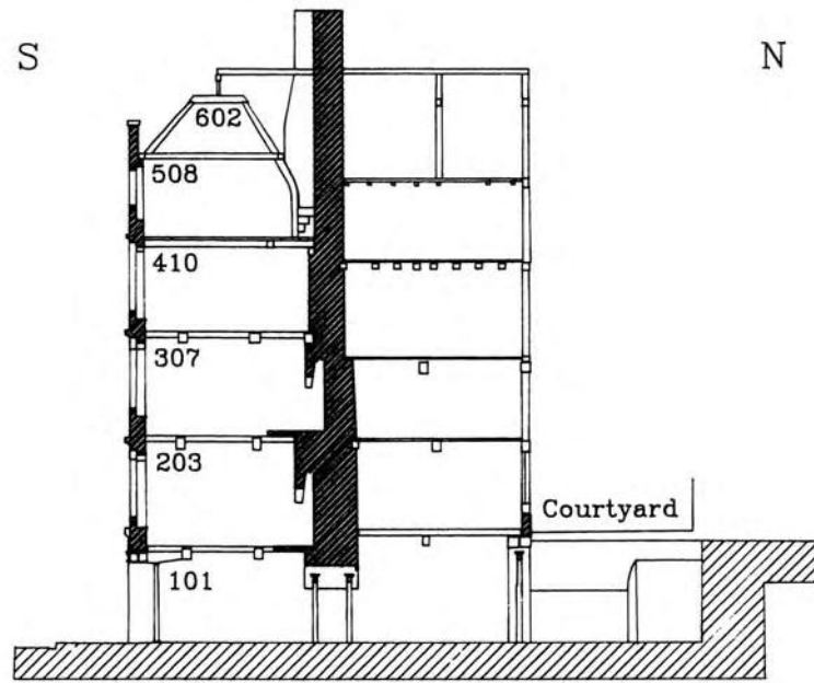
Figure 10. Section of Milbank House at Bessie Surtees House. Based on Figure 10 of Heslop et al (1994)
