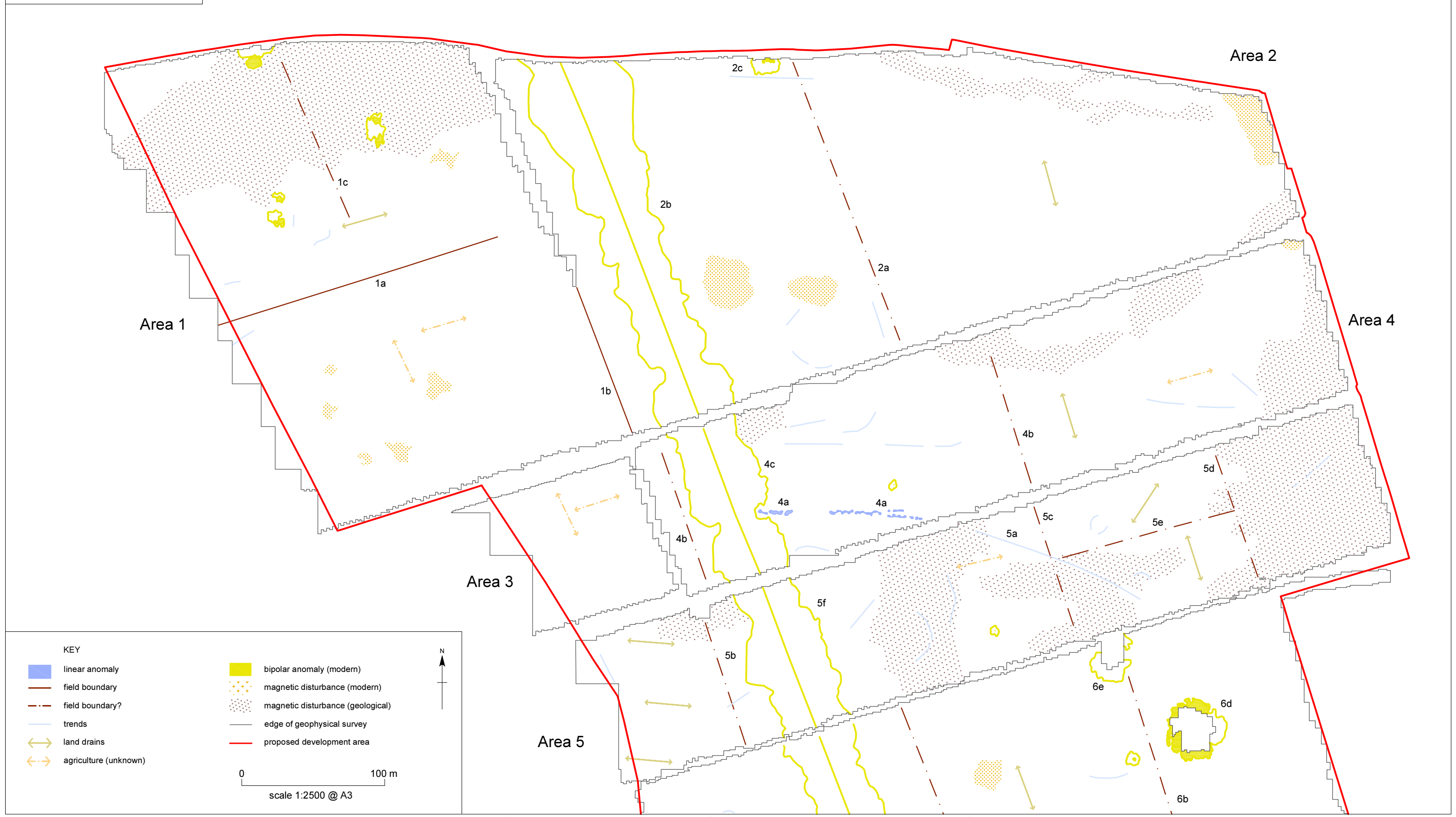
Sweetbriar Farm: interpretation of gradiometer survey results - Areas 1, 2, 3, 4 and 5
