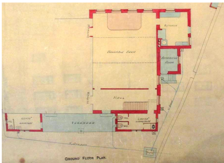
Figure 3: Ground Floor Plan of proposed Adult School (Brotherton Library, Special Collections, MS/DEP/1979/1/HUD/1/13)
