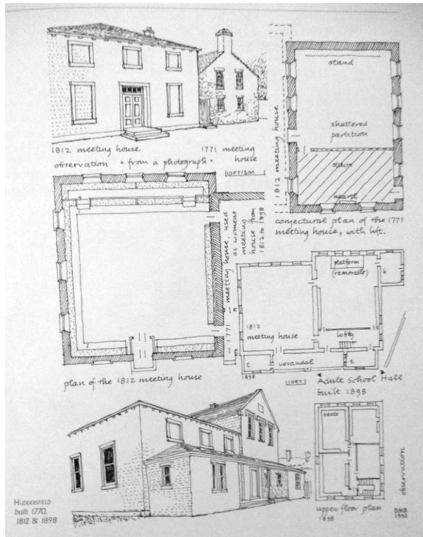
Figure 3: Ground floor plan (not to scale) and perspective (Butler, The Quaker Meeting Houses of Britain , 1999, vol. 2, p. 805)
