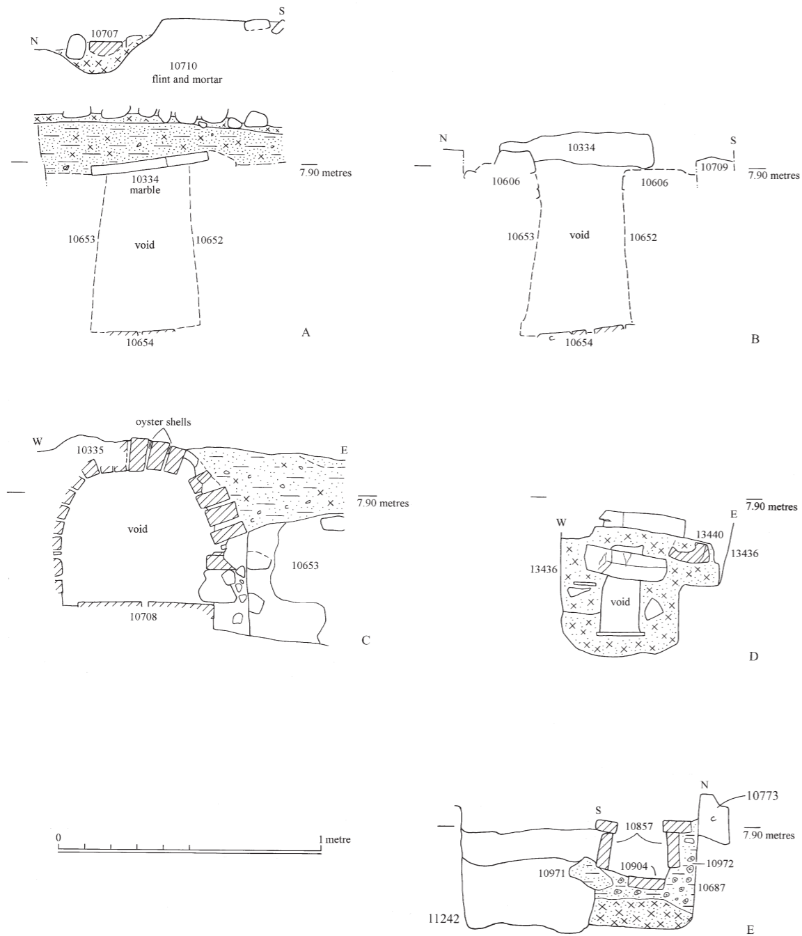
Figure 3.20 Sections across Friary drains A and B: Section of Great Drain 10654, Area A C: Section of tributary drain 10335, Area A D: Section of tributary drain 13440, Area D E: Section of tributary drain 10795/10857/10904, Area A
