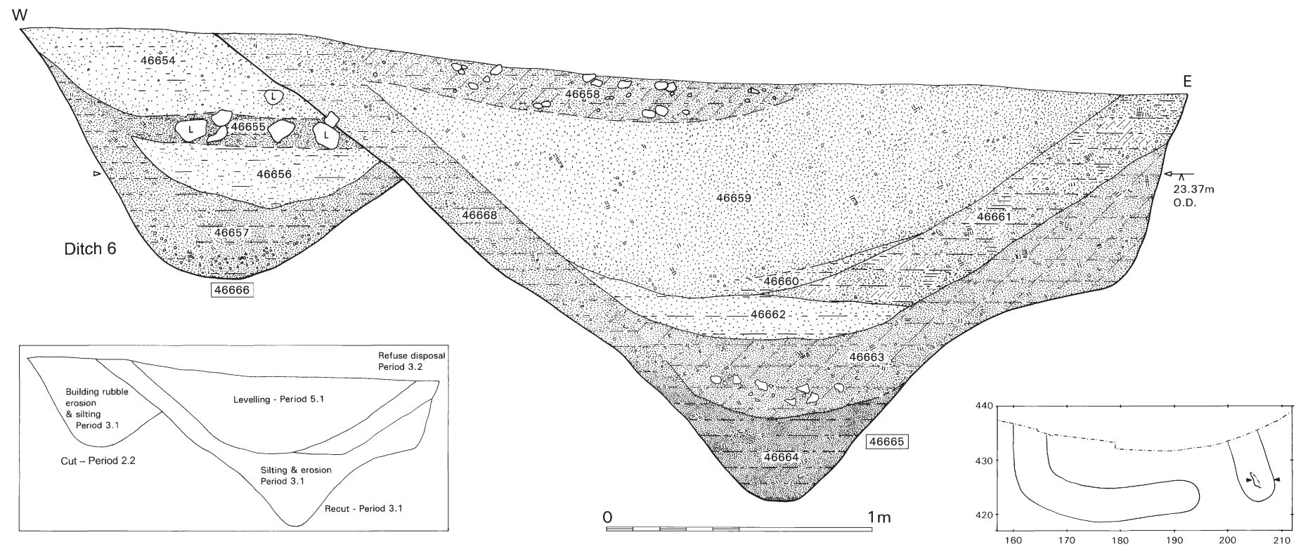
Figure 5.22 Period 2.2: South-facing section across Ditch 6 (Area 46, S.4613). Scale 1:20
