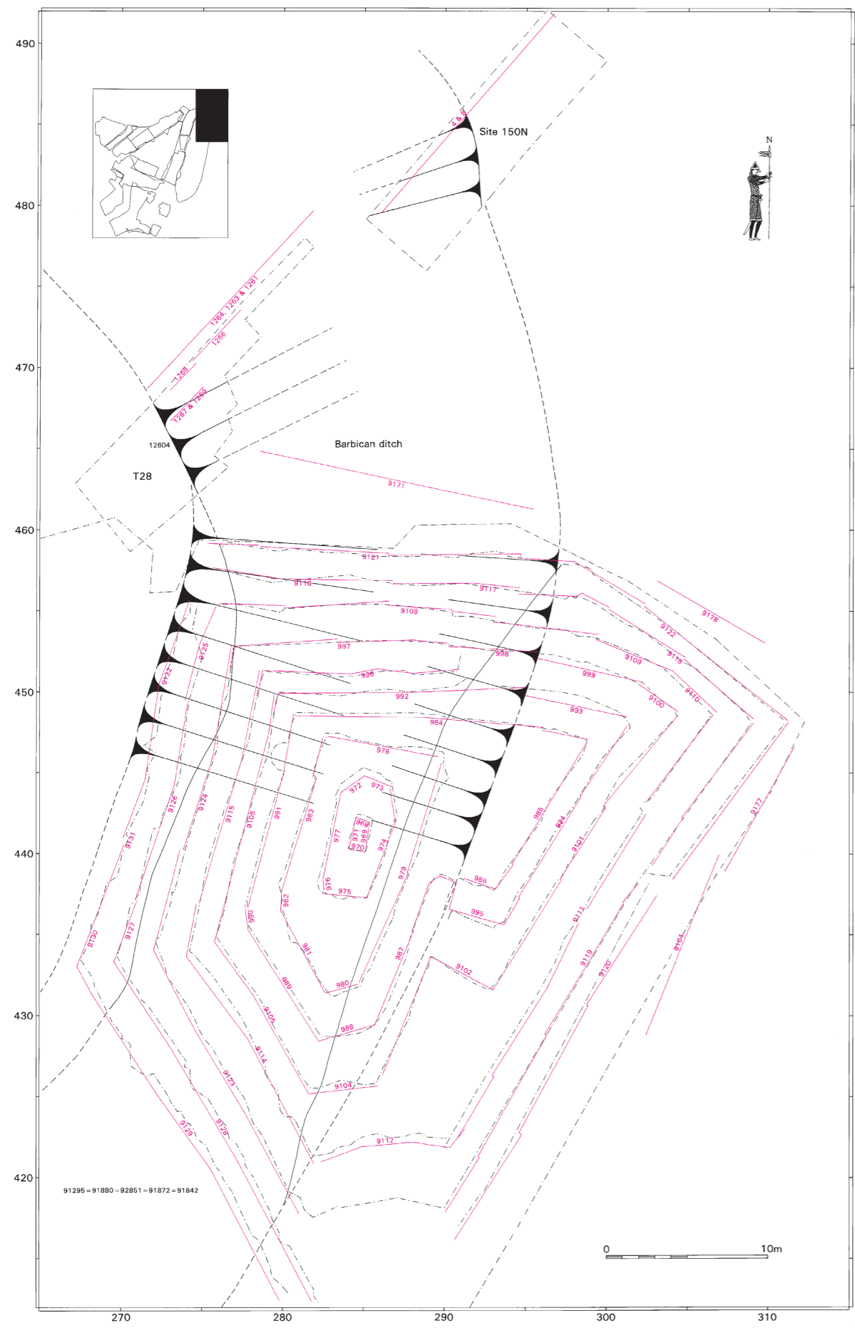
Figure 7.17 Period 4.2: Plan of machine trenches across Ditch 13 (barbican) (Area 9). Scale 1:300
