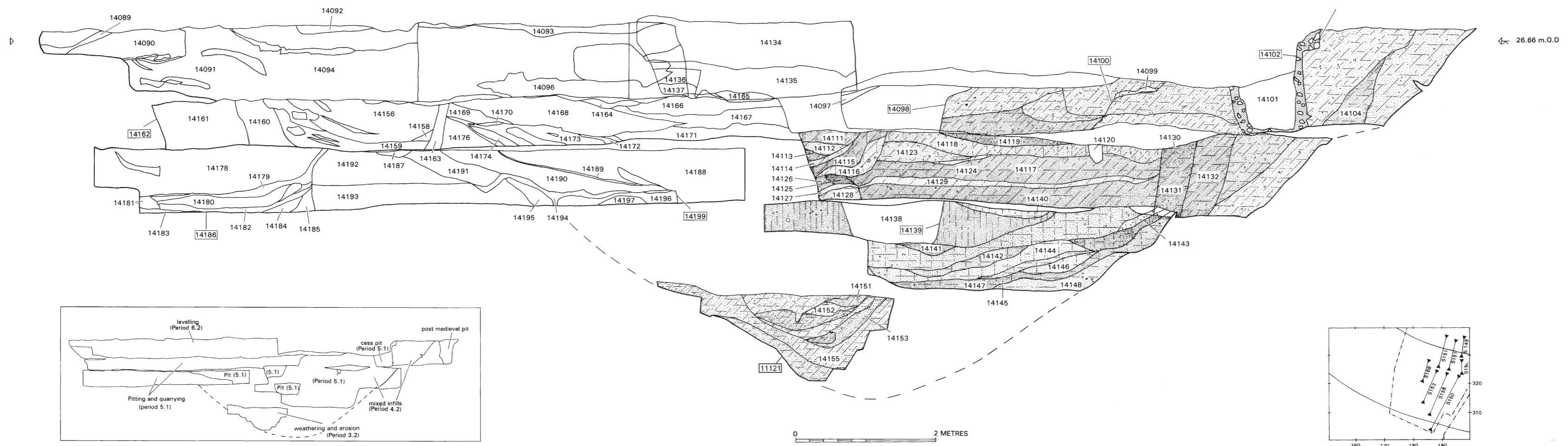
Figure 8.14 Period 5.1: West-facing section showing quarries above south bailey ditch (Ditch 10, Area 1). See Fig. 8.15 for location. Scale 1:50
