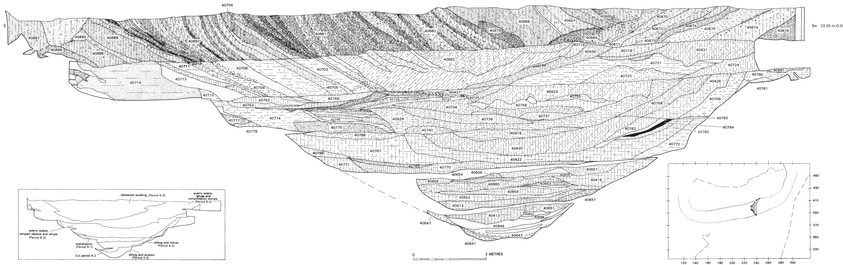
Figure 8.26 Periods 5 & 6: Composite west-facing section across Ditch 13 (barbican) (Area 4). Scale 1:50
