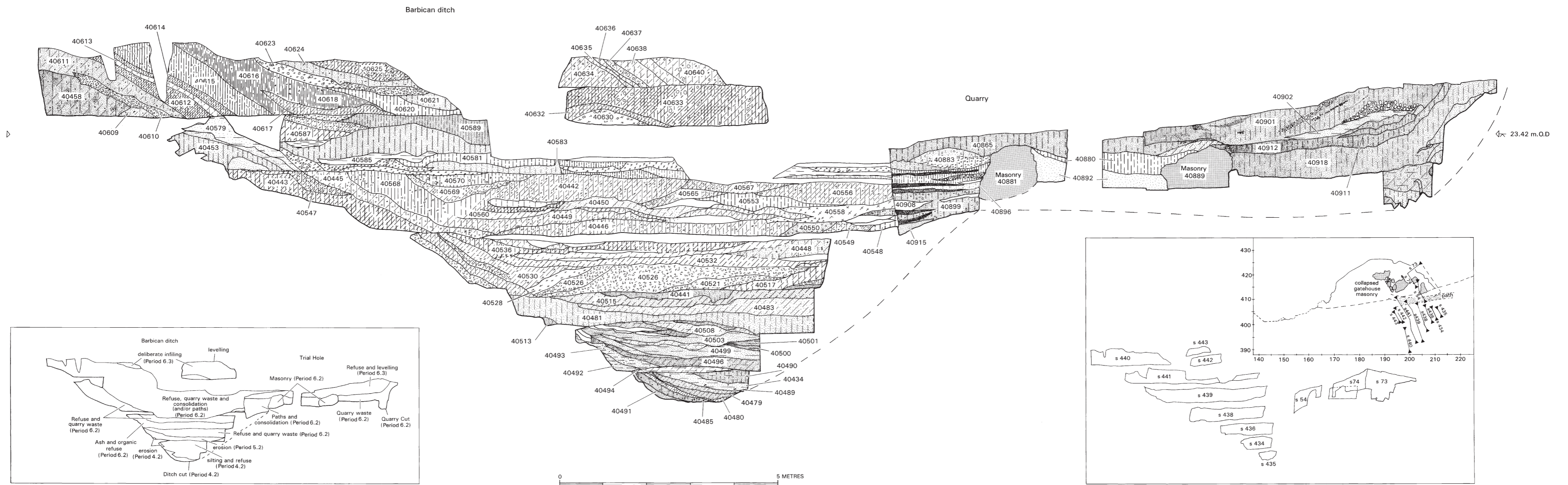
Figure 8.27 Periods 5 & 6: Composite east-facing section across Ditch 13 (barbican) and quarry to its north (Area 4). See Fig. 10.5 for location. Scale 1:75
