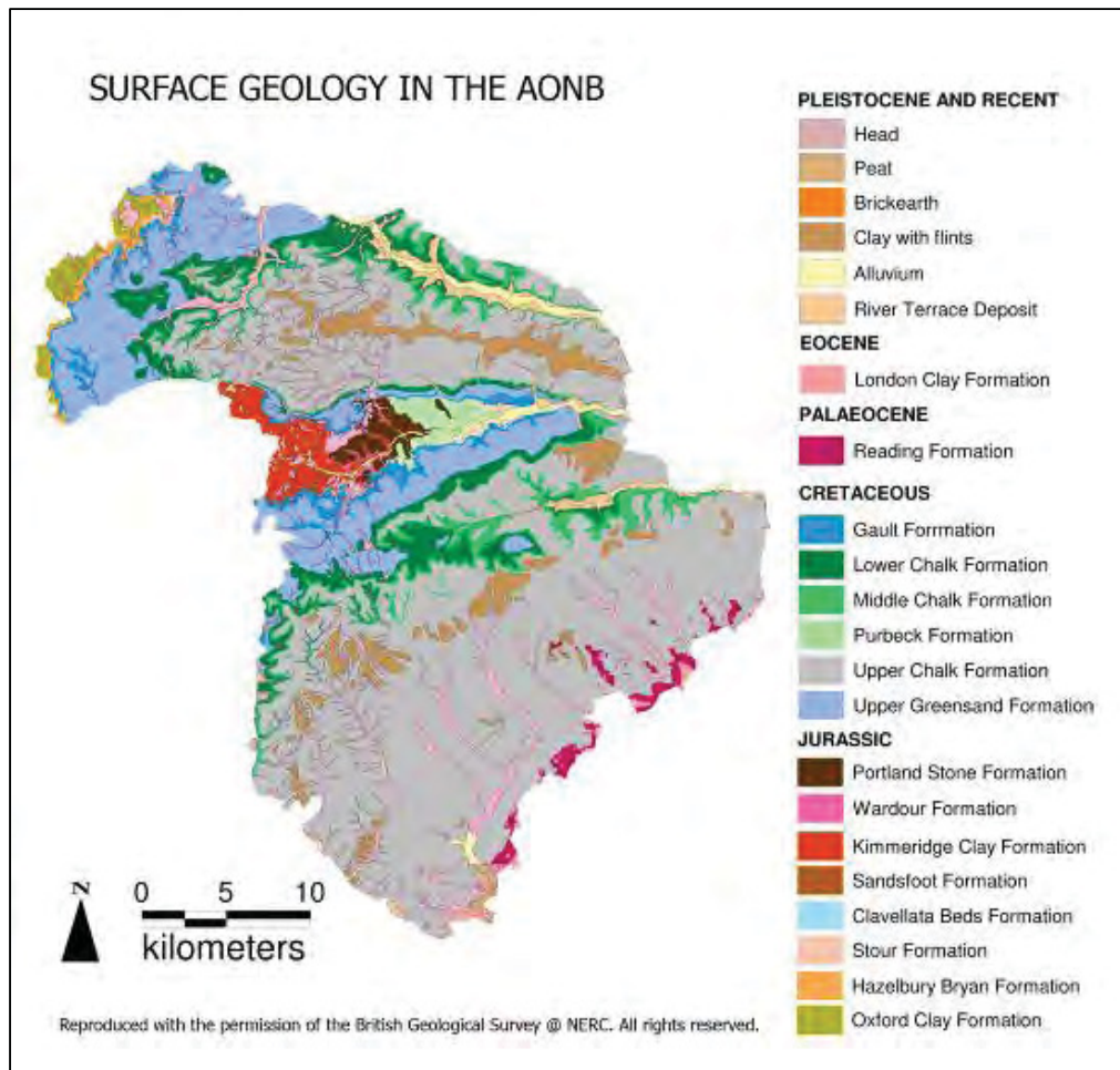
Figure 3: Geology of the AONB
