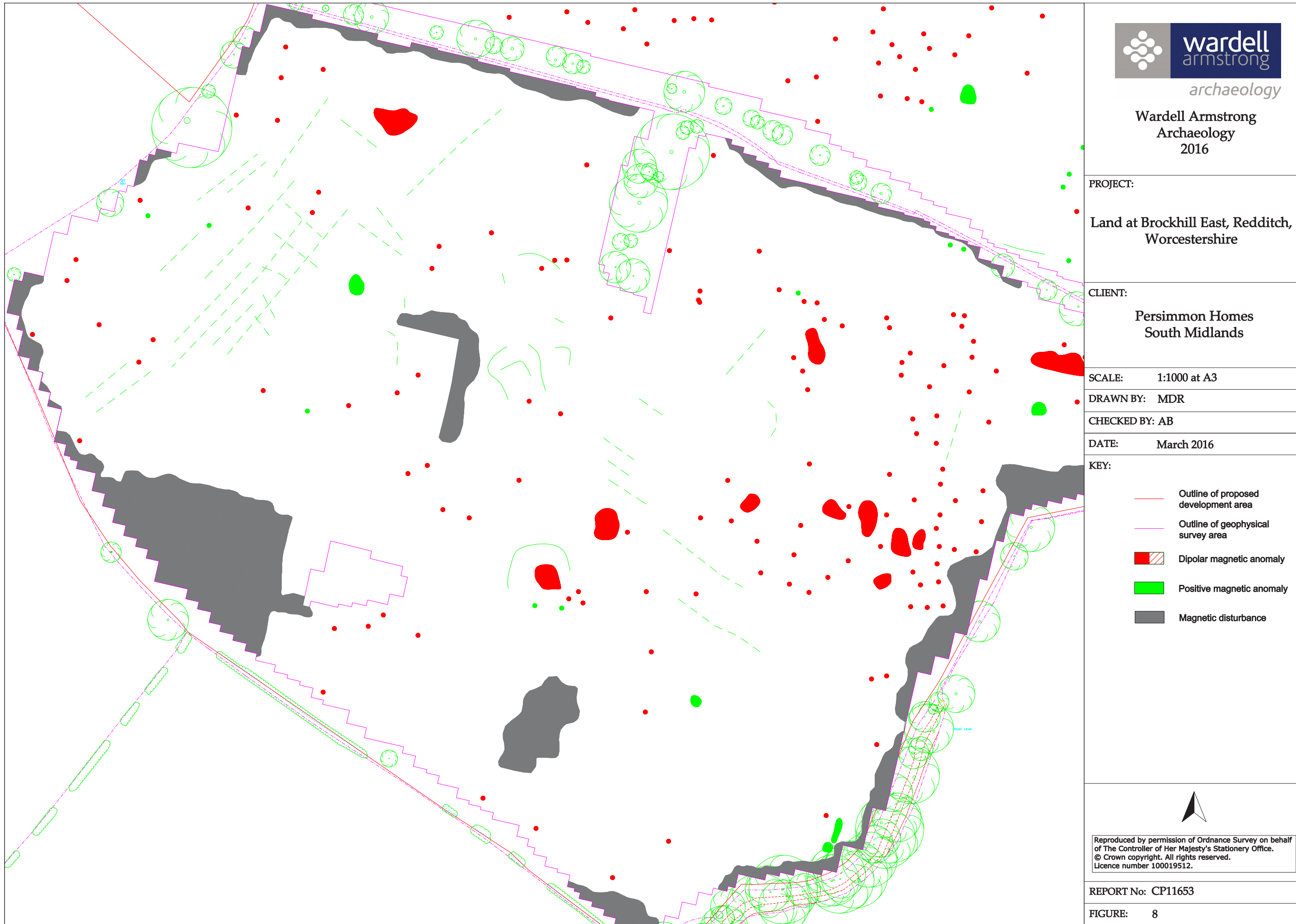
Figure 8: Geophysical interpretation of Area 2.
