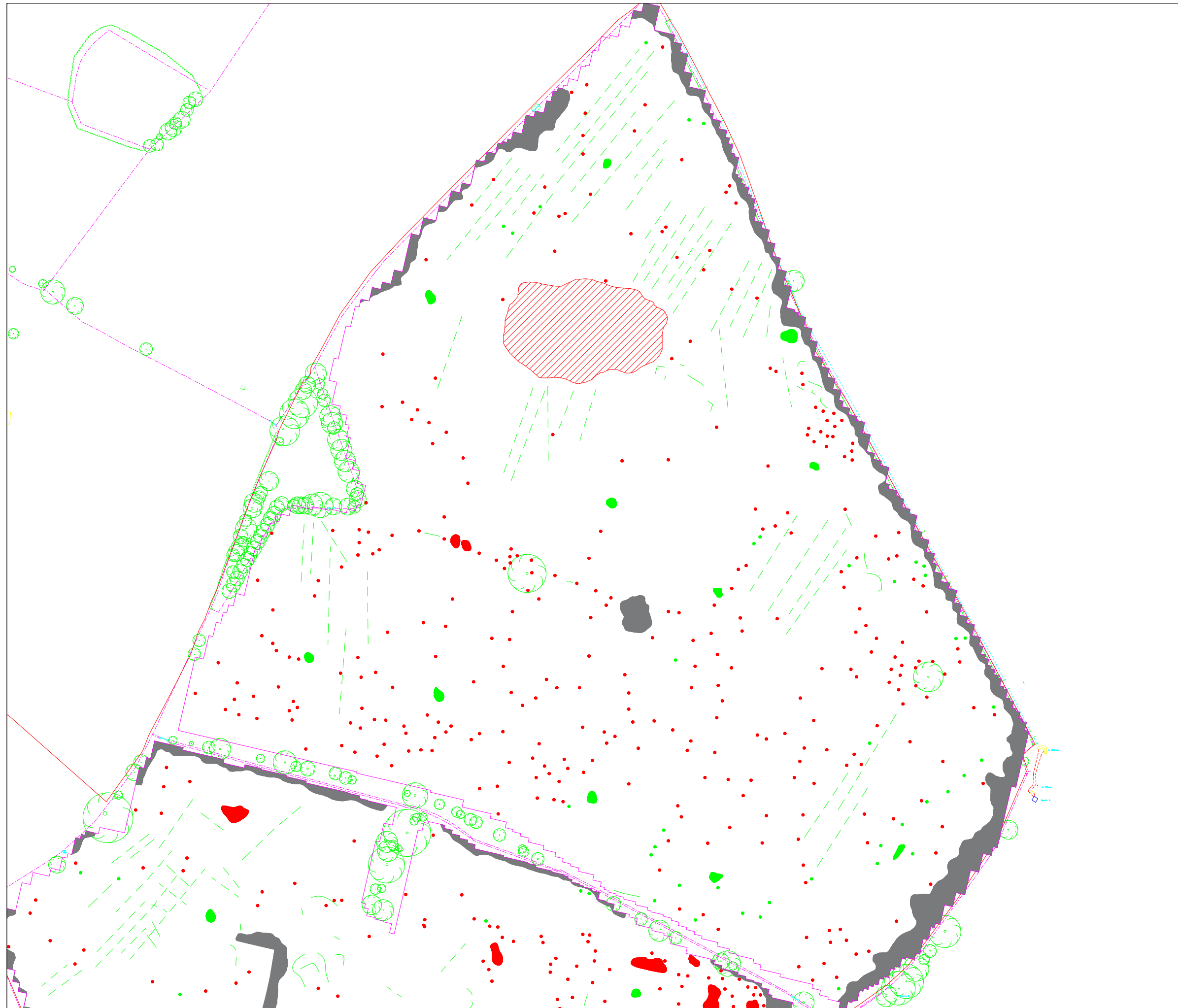
Figure 5: Geophysical interpretation of Area 1.
