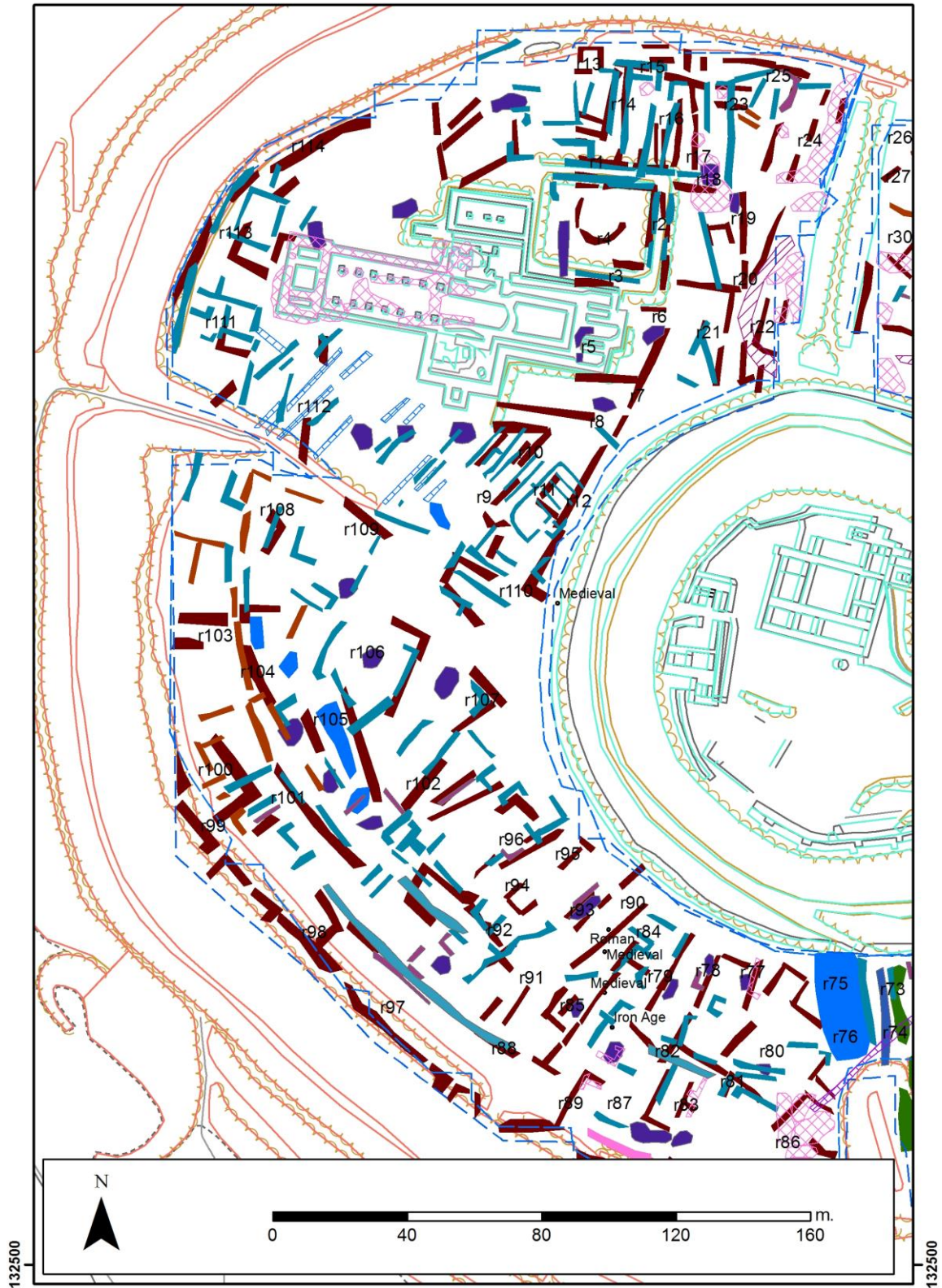
Figure 37 Composite image of the magnetometer, earth resistance and GPR interpretation plots for the western part of Old Sarum (© Crown Copyright/database right 2014. An Ordnance Survey/EDINA supplied service)
