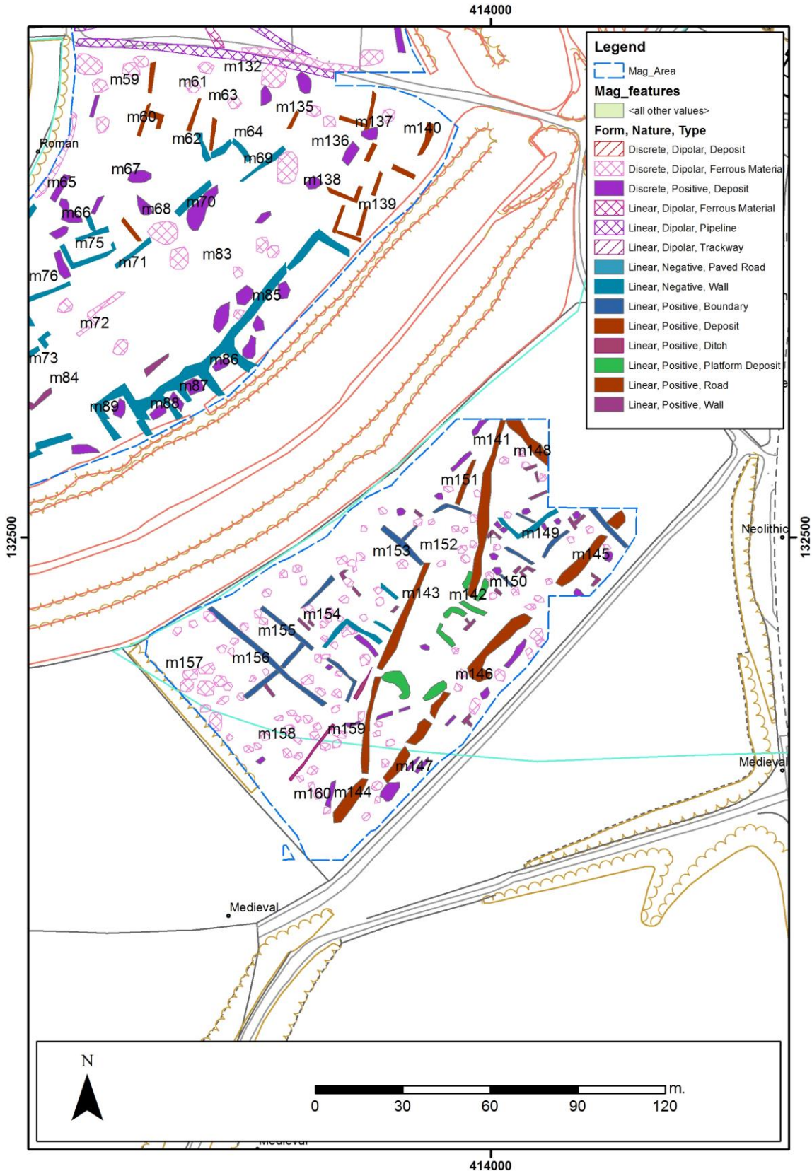
Figure 21 Interpretation plot derived from the results of the magnetometer survey for the field to the south of Old Sarum (© Crown Copyright/database right 2014. An Ordnance Survey/EDINA supplied service)
