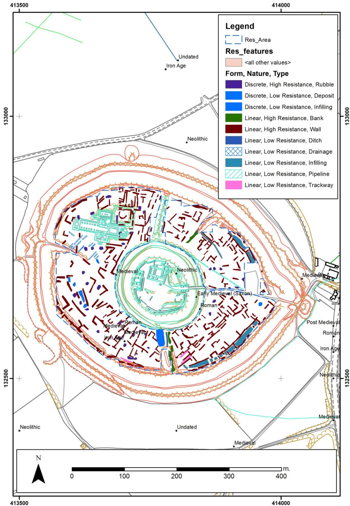
Figure 29 Interpretation plot derived from the results of the earth resistance survey for Old Sarum (© Crown Copyright/database right 2014. An Ordnance Survey/EDINA supplied service)
