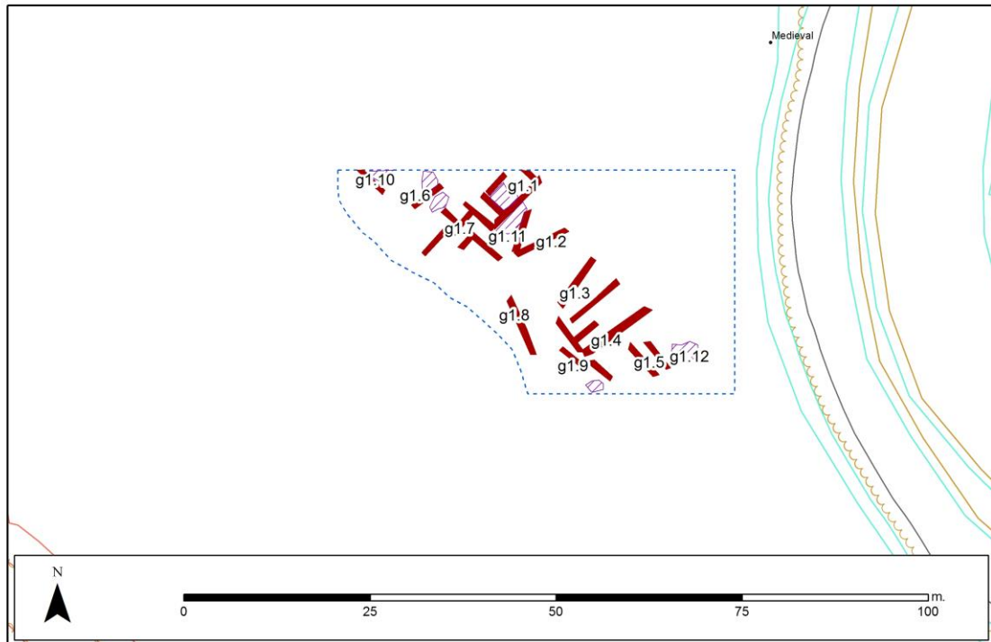
Figure 33 Interpretation plot for the GPR results for the west side of the outer bailey for 107.5-107.7m asl (© Crown Copyright/database right 2014. An Ordnance Survey/EDINA supplied service)
