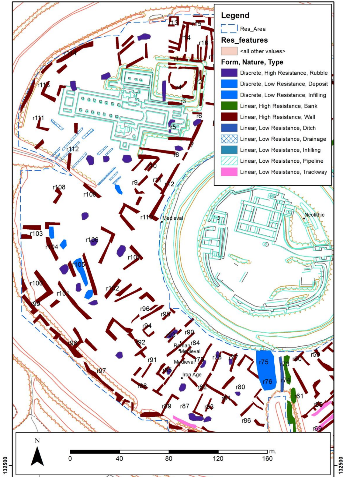
Figure 26 Interpretation plot derived from the results of the earth resistance survey for the western part of Old Sarum (© Crown Copyright/database right 2014. An Ordnance Survey/EDINA supplied service)
