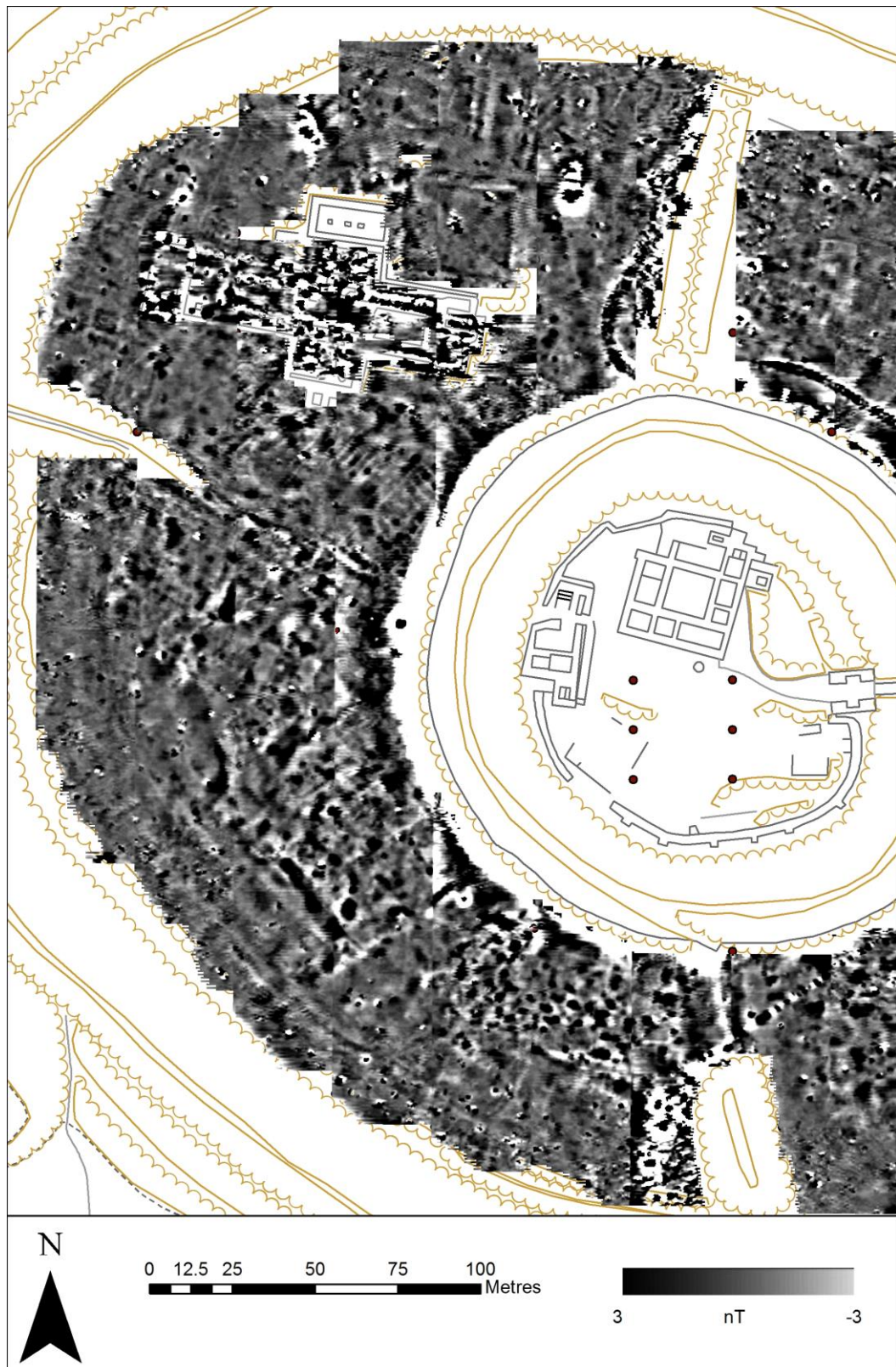
Figure 15 Greyscale image of the magnetometer survey for the western part of Old Sarum (© Crown Copyright/database right 2014. An Ordnance Survey/EDINA supplied service)
