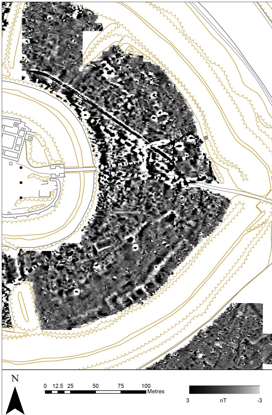
Figure 17 Greyscale image of the magnetometer survey for the eastern part of Old Sarum (© Crown Copyright/database right 2014. An Ordnance Survey/EDINA supplied service)
