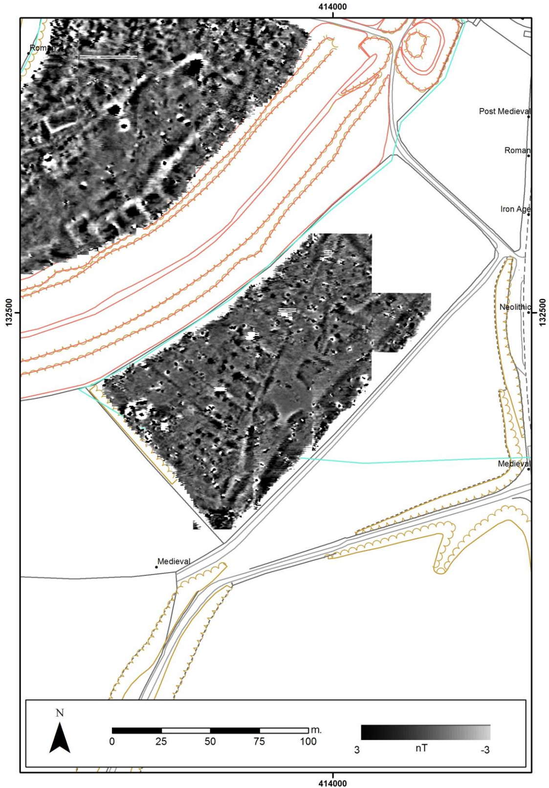
Figure 20 Greyscale image of the magnetometer survey for the field to the south of Old Sarum (© Crown Copyright/database right 2014. An Ordnance Survey/EDINA supplied service)
