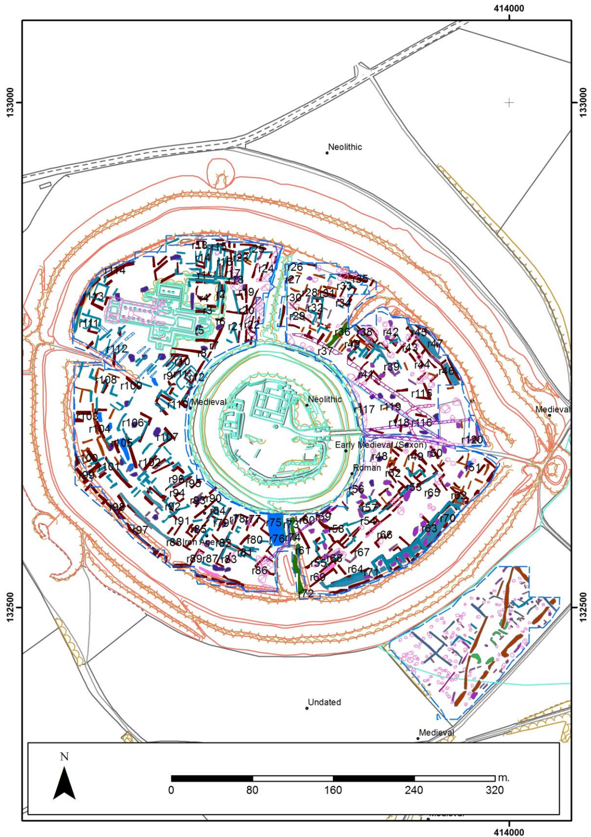
Figure 40 Composite image of the magnetometer and earth resistance plots for Old Sarum (© Crown Copyright/database right 2014. An Ordnance Survey/EDINA supplied service)
