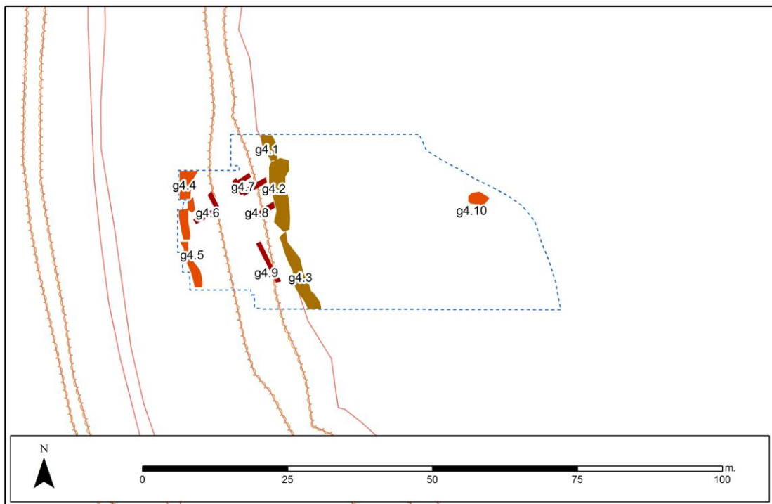
Figure 39 Interpretation plot for the GPR results for the west side of the outer bailey for 96.7-96.9m asl (© Crown Copyright/database right 2014. An Ordnance Survey/EDINA supplied service)
