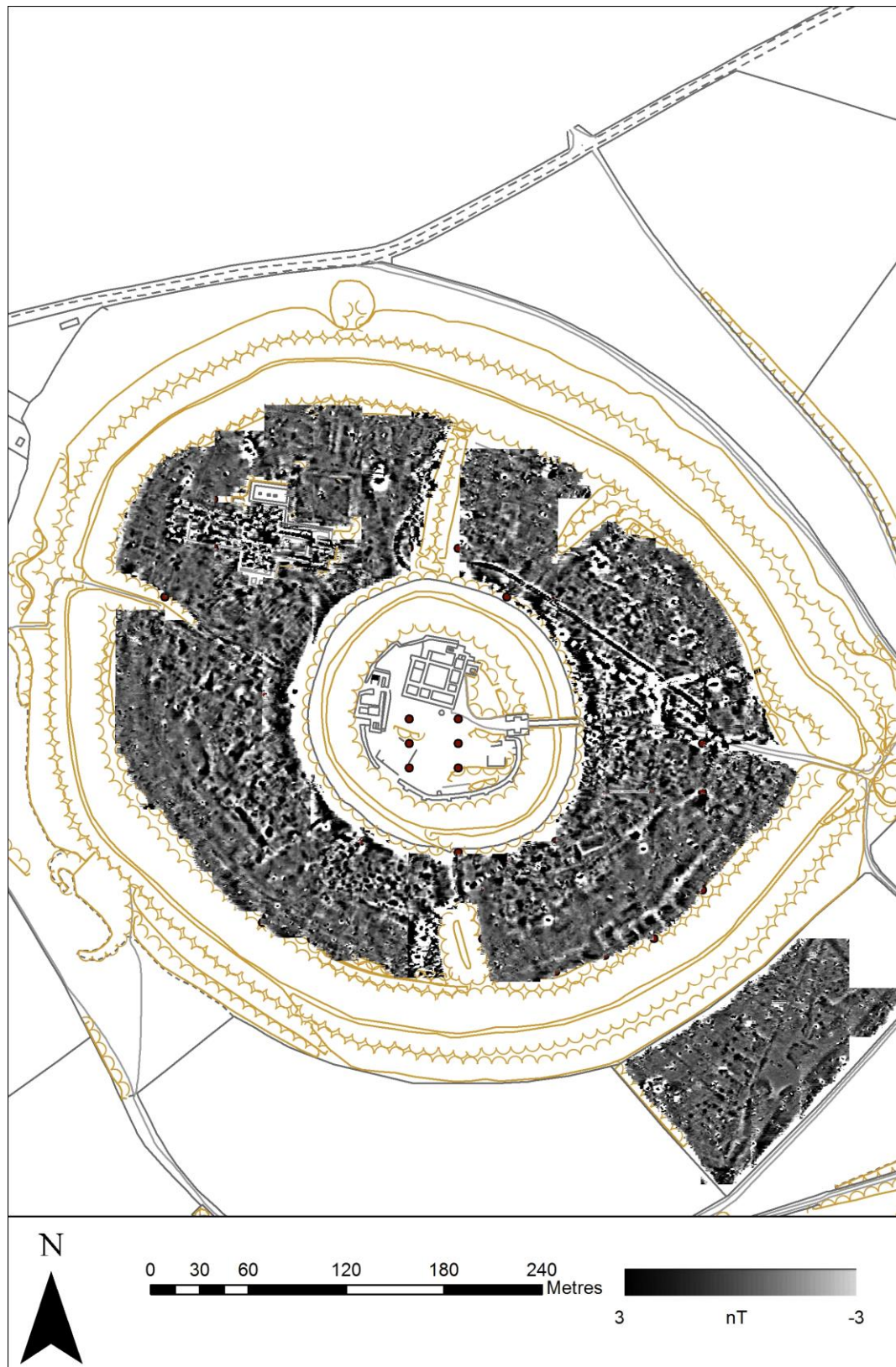
Figure 14 Greyscale image of the magnetometer survey at Old Sarum (© Crown Copyright/database right 2014. An Ordnance Survey/EDINA supplied service)
