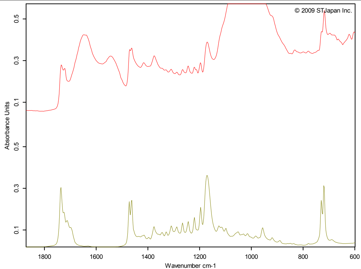
Figure 3: Detail showing spectral match in IR region between 600 and 1800 cm -1 wavenumbers. Top (red) K400-1-7. Bottom (green) Beeswax reference spectrum, ST Japan 2009.
