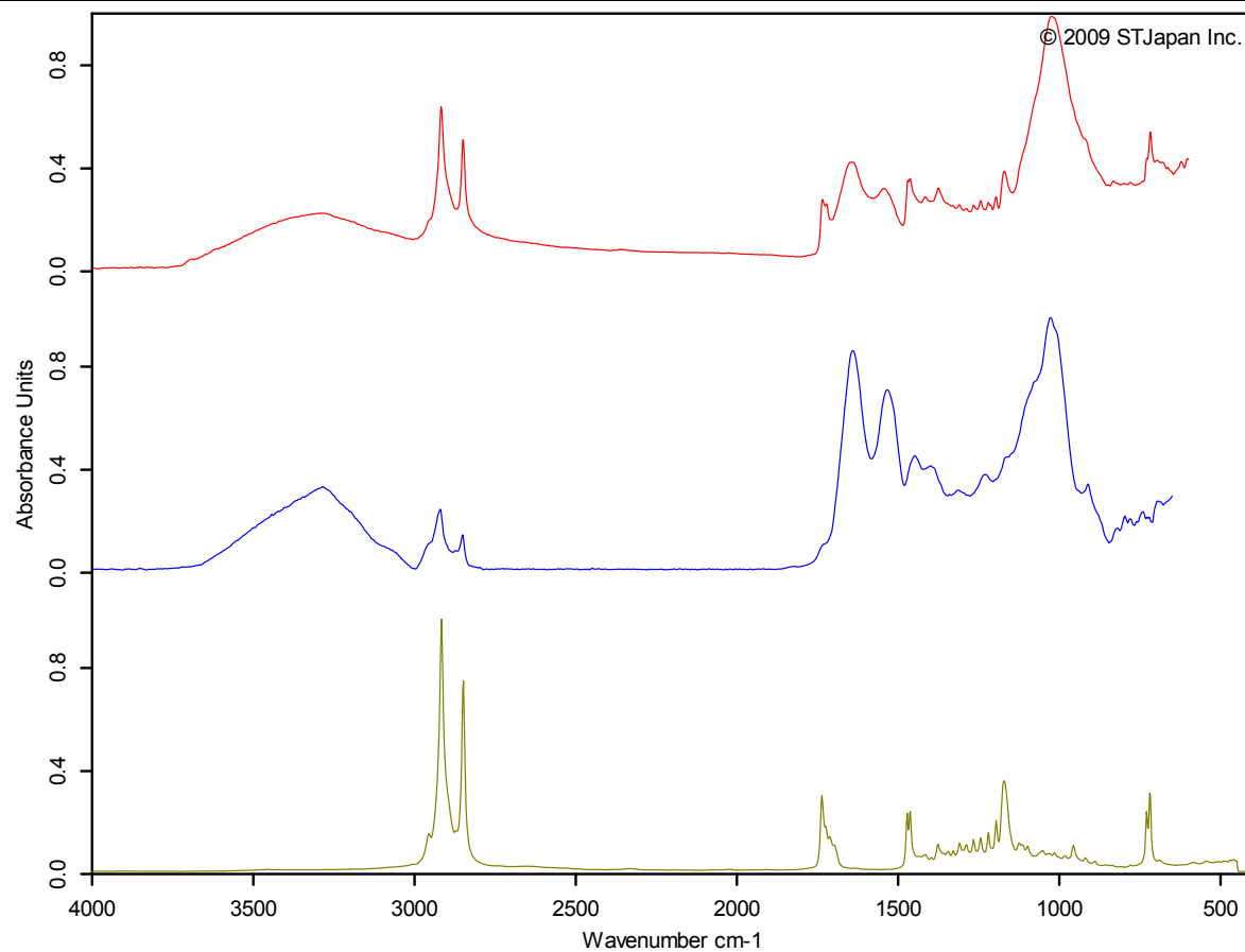
Figure 2: Top (red) K400-1-7. Middle (blue) Oxidised horse hair reference spectrum, ST Japan 2009. Bottom (green) Beeswax reference spectrum, ST Japan 2009.
