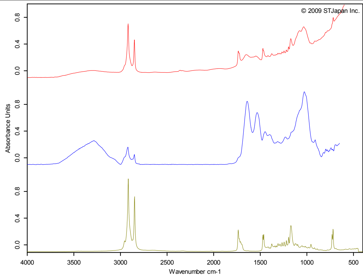
Figure 4. Top (red) spectrum for K850-1-2. Middle (blue) Oxidised horse hair reference spectrum, ST Japan 2009. Bottom (green) Beeswax reference spectrum, ST Japan 2009.
