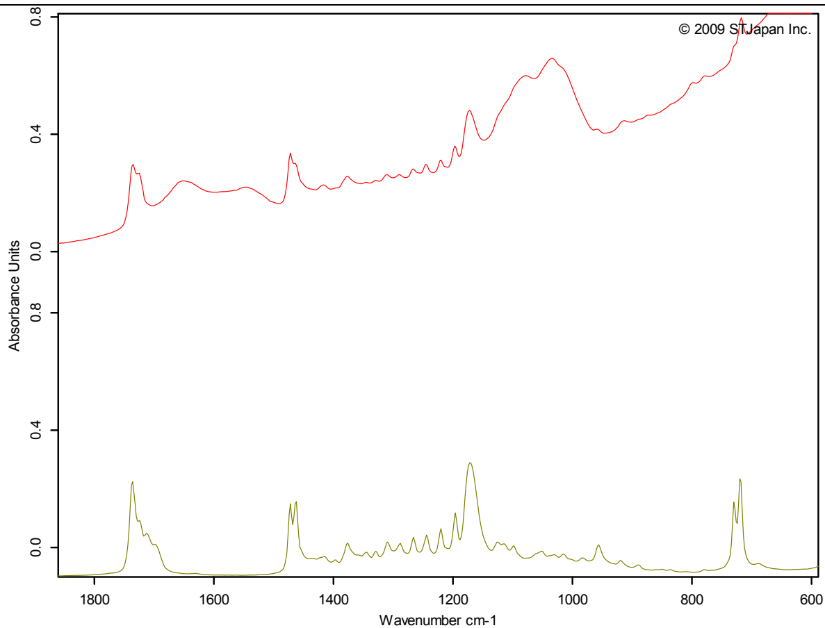
Figure 5. Detail of 600-1800cm -1 region of spectra- top (red) spectrum for K850-1-2, and bottom (green) Beeswax reference spectrum, ST Japan 2009, showing subtle confirmative peaks for beeswax represented in this part of the spectrum.
