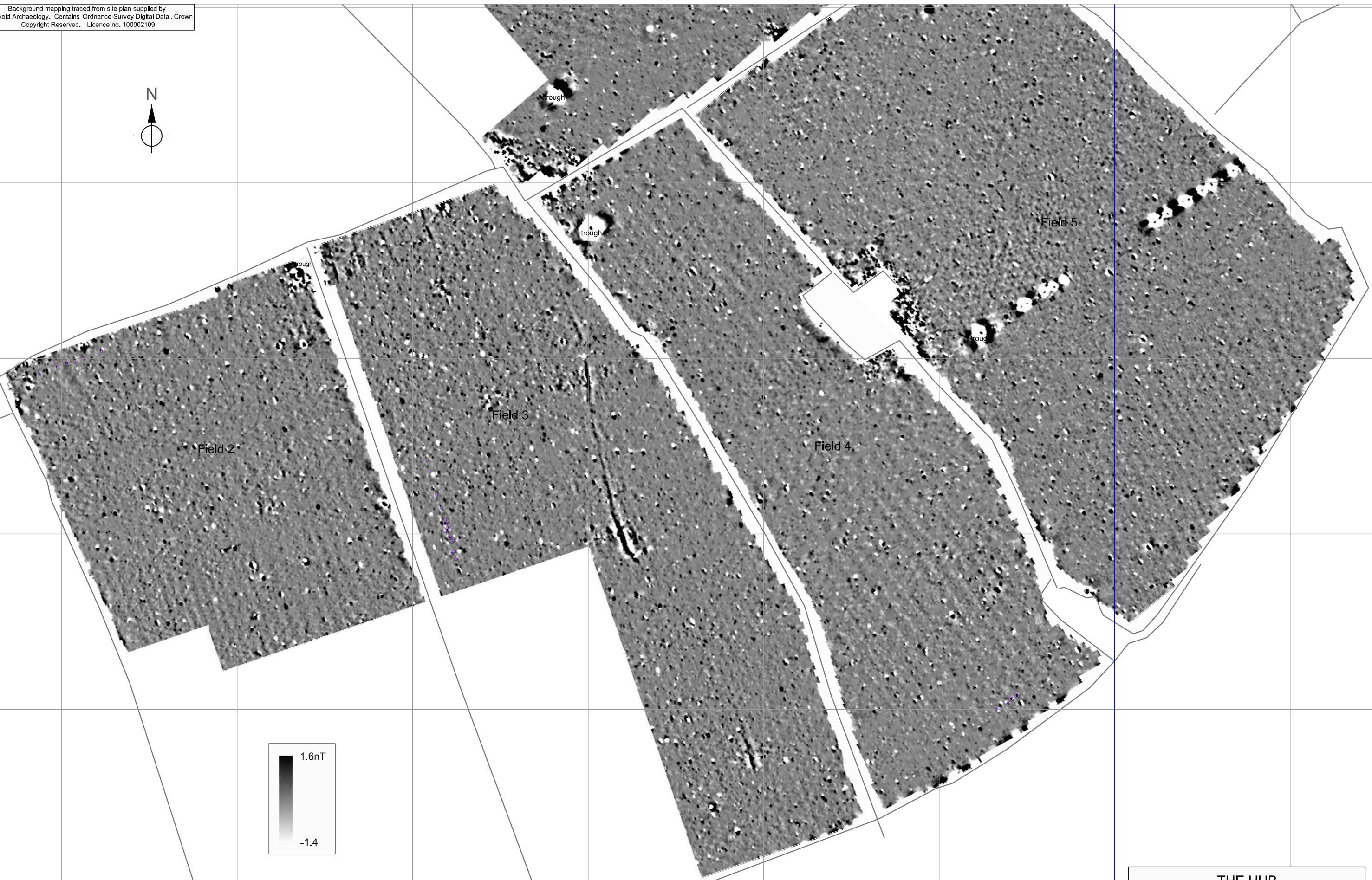
THE HUB SWINDON, WILTSHIRE Geophysical Survey 2013 Figure 3: Magnetometer survey (grey scale plot)
