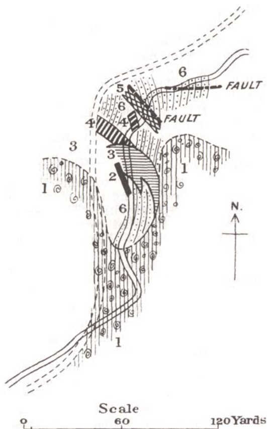
Illus 31 Sketch-map of exposures in the main western headwater of the Lag a' Bheith, 2 miles SSW of Brodick Pier: 1 = felsite sill; 2 = basalt dyke; 3 = shattered basaltic intrusion; 4 = pitchstone dykes; 5 = crushed basalt dyke along fault; 6 = marls, cornstones, and sandstones of the Trias period (Tyrrell 1928, fig 28).
