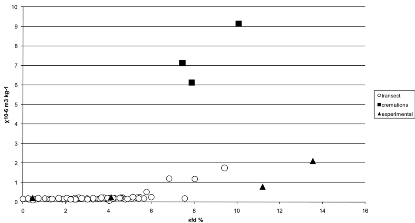
Illus 20 Biplot of \kappa \text{fd}\% vs \chi for all samples
