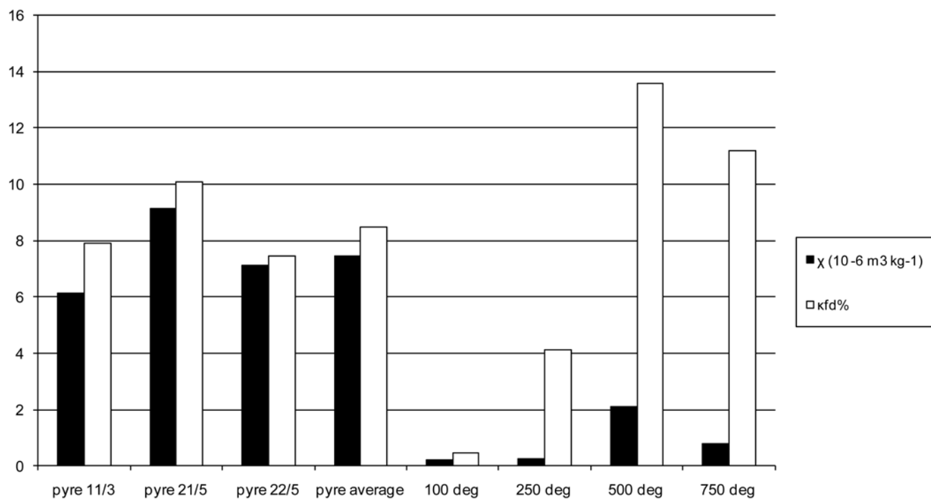
Illus 19 Mass specific and frequency dependent magnetic susceptibility of cremation and experimental samples
