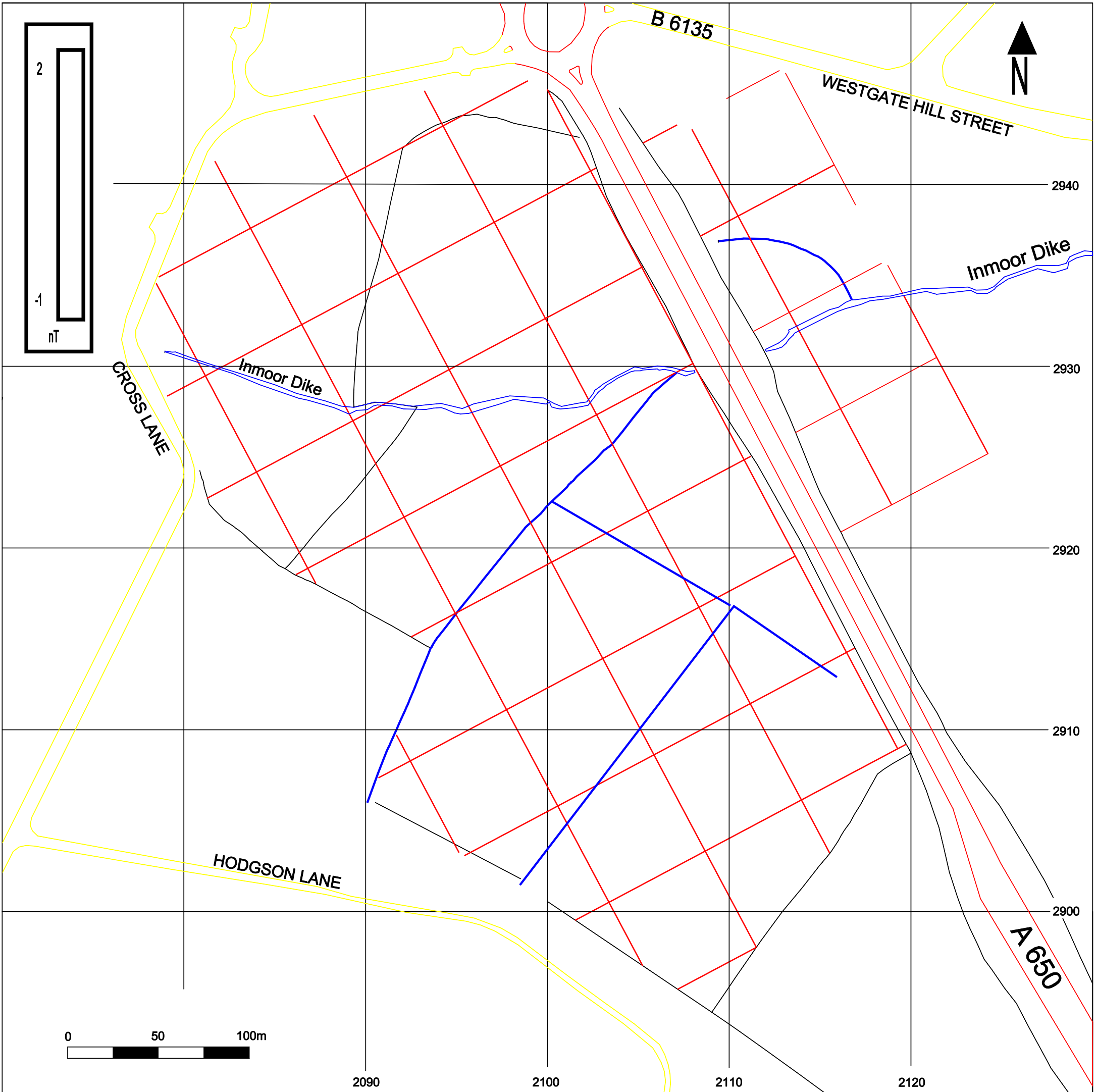
Fig. 2. Site location showing geophysical survey area and gradiometer data (dot density 1:2500)
