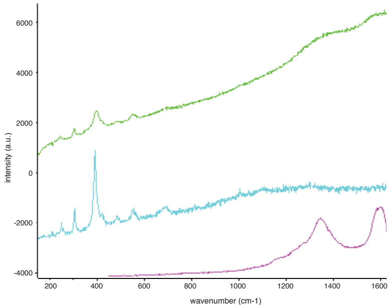
Data Fig 15 Raman spectrum obtained for yellow material on wood <142>a from box <S22>: top spectrum (green), sample material; middle spectrum (blue), reference spectrum for goethite; bottom spectrum (pink), reference spectrum for amorphous carbon
