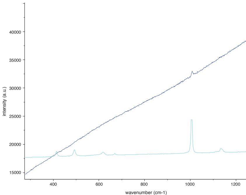
Data Fig 17 Raman spectrum obtained for white material on wood <142>a from box <S22>: top spectrum (dark blue), sample material; bottom spectrum (light blue), reference spectrum for gypsum
