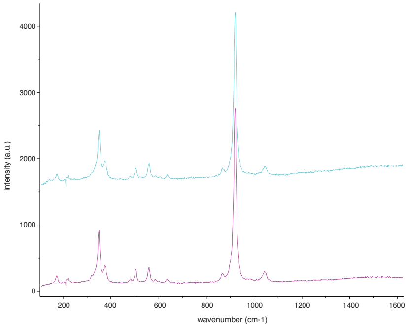
Data Fig 18 Raman spectra obtained for the two garnets on lyre <S58>: top spectrum, <164>; bottom spectrum, <165>
