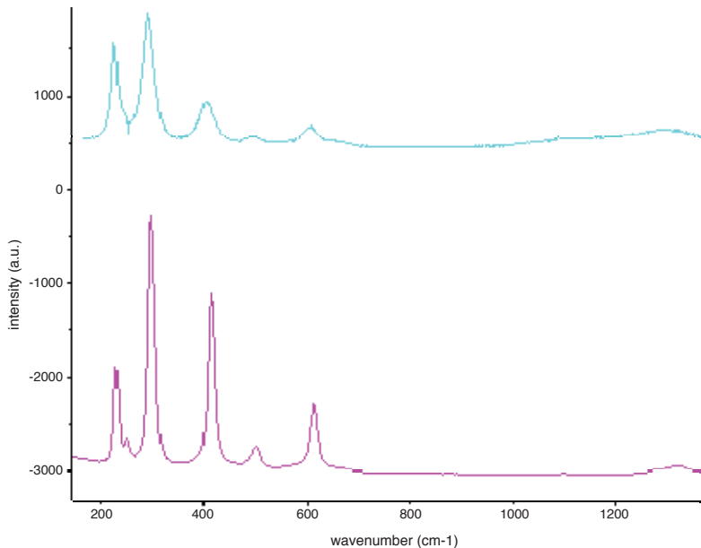
Data Fig 16 Raman spectrum obtained for red material on wood <142>a from box <S22>: top spectrum (blue), sample material; bottom spectrum (pink), reference spectrum for haematite
