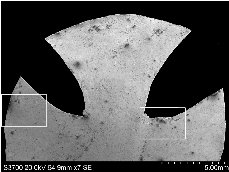
Data Fig 20 Secondary electron photomicrograph of gold-foil cross <S17> (the white squares show the locations of Data Fig 21 (right) and Data Fig 22 (left))
